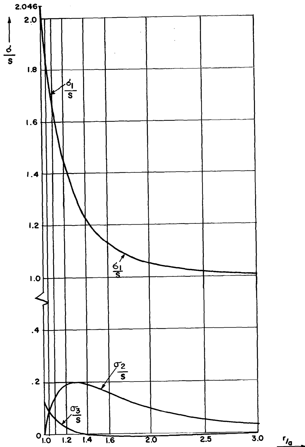
Figure 15 Stress Distribution Around A Spherical Void Equatorial Plane \mu_m = .3
