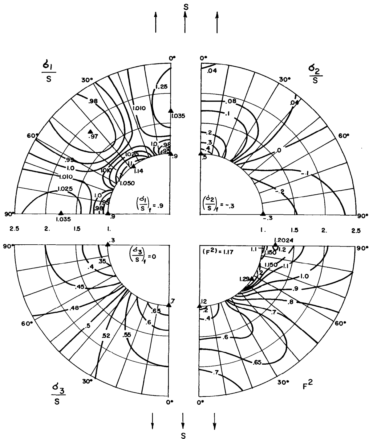
Figure 13 Stress Distribution Around A Cylindrical Inclusion With Different Poisson's Ratio (Plane Strain Assumption) \mu_f = 0 , \mu_m = .5
