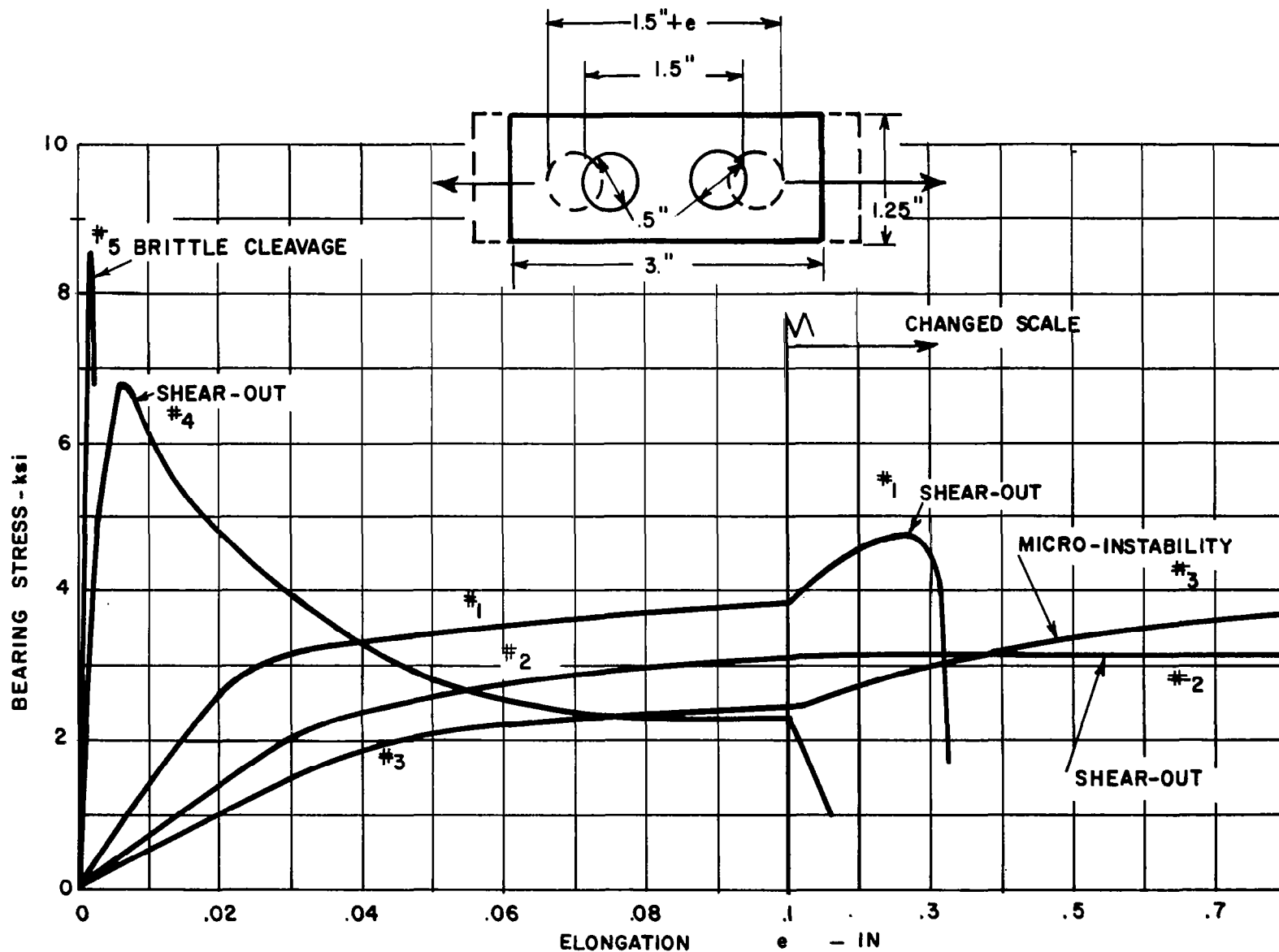
Figure 30 Bearing Stress Vs Elongation
