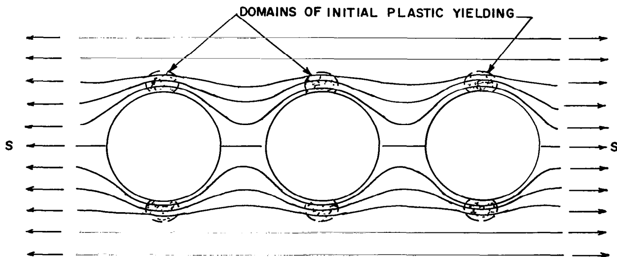
Figure 20b Array of Voids Exhibiting Parallel Failure Mode - Ductile Stress Relief
