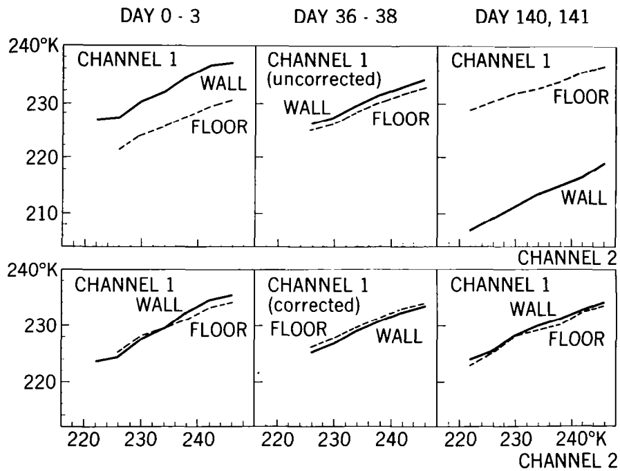
Fig.3.3: Simultaneous measurements of channel 1 (averaged) vs. those of channel 2 (corrected for degradation).
