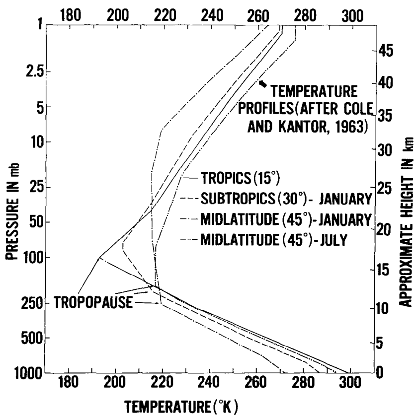
Fig.2.5: Temperature profiles
