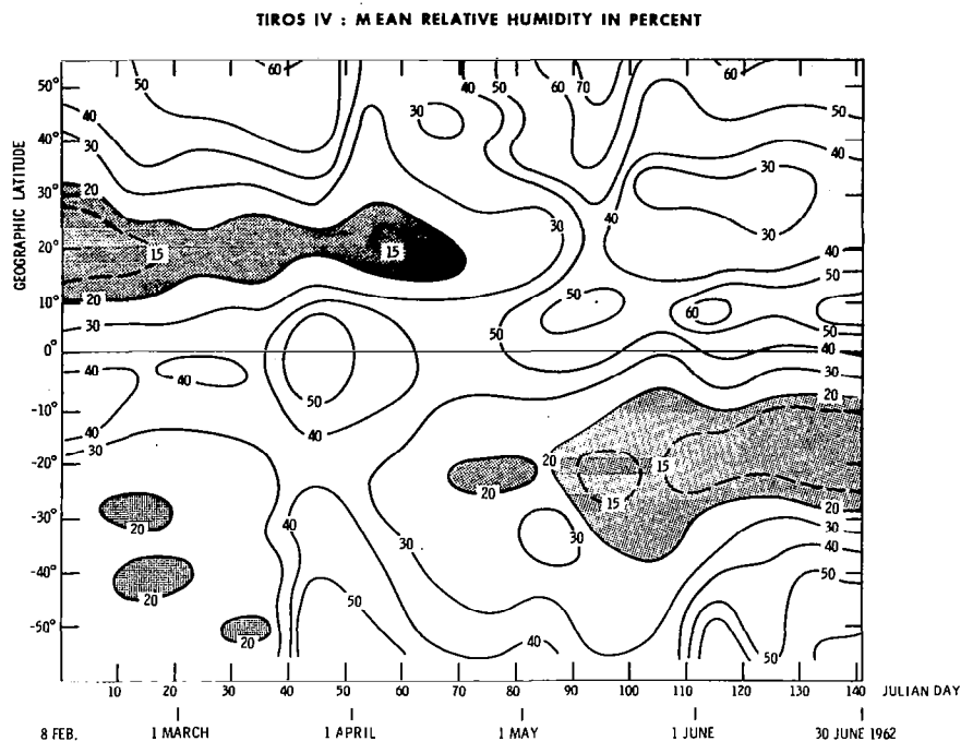
Fig.4.11: Zonal averages of the mean relative humidity for 10-day periods
