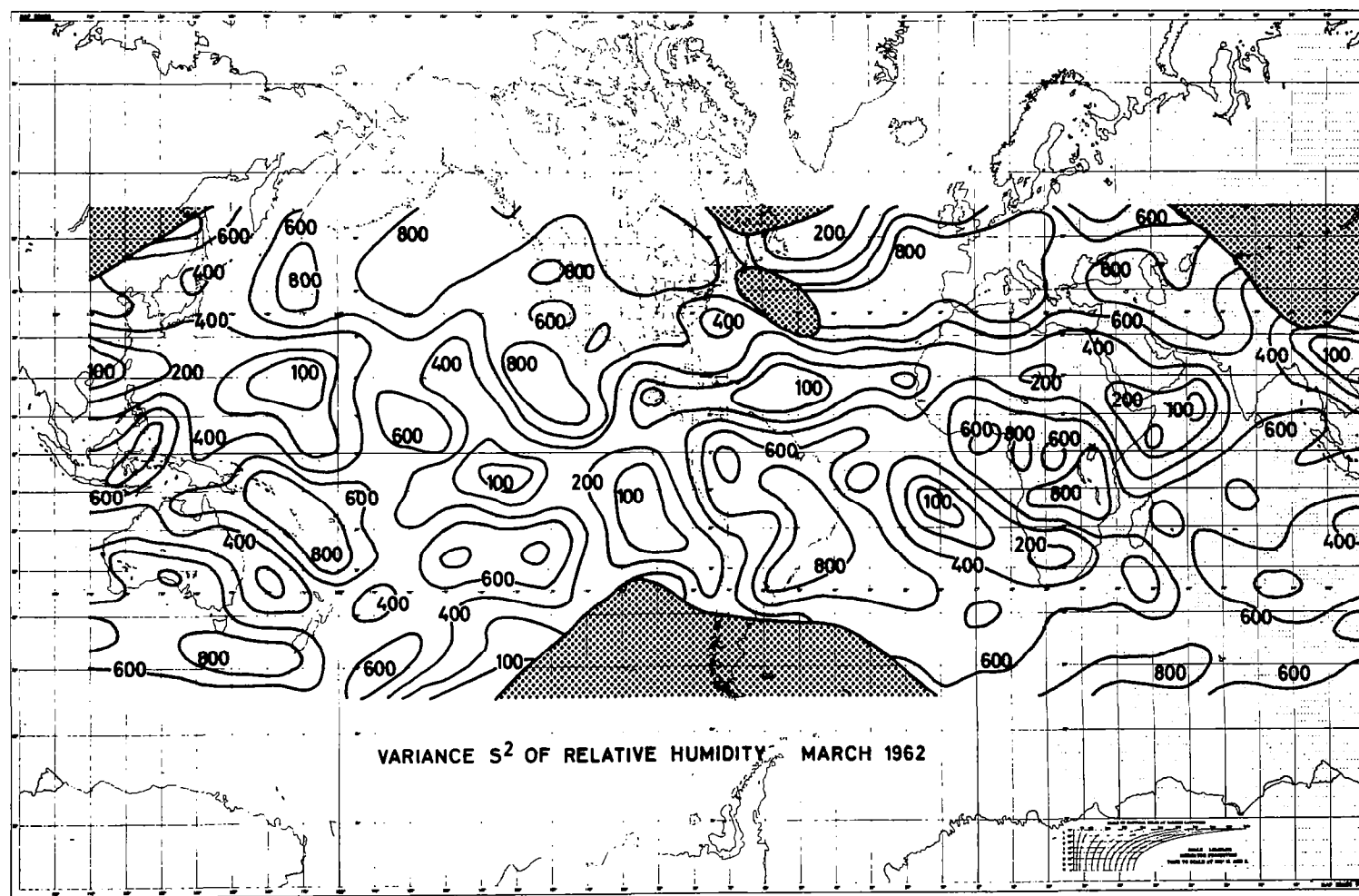
Fig.4.15: Variances S^2 (in per cent 2 ) of the mean relative humidity (March 1962)
