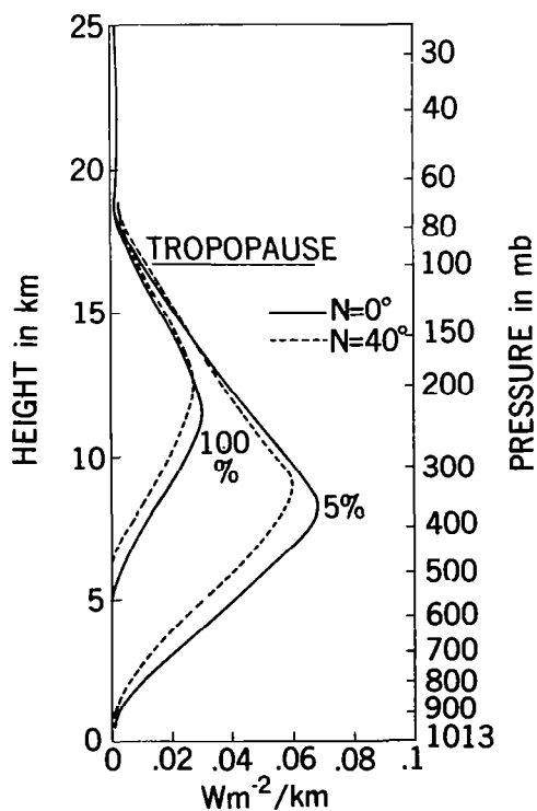
Fig.2.3: Curves \int_0^\infty \phi_v B_v(\log p) \frac{d\tau_v(w \log p)}{d \log p} dv vs. height for the upward going radiation in the spectral range of channel 1 in a tropical model atmosphere
