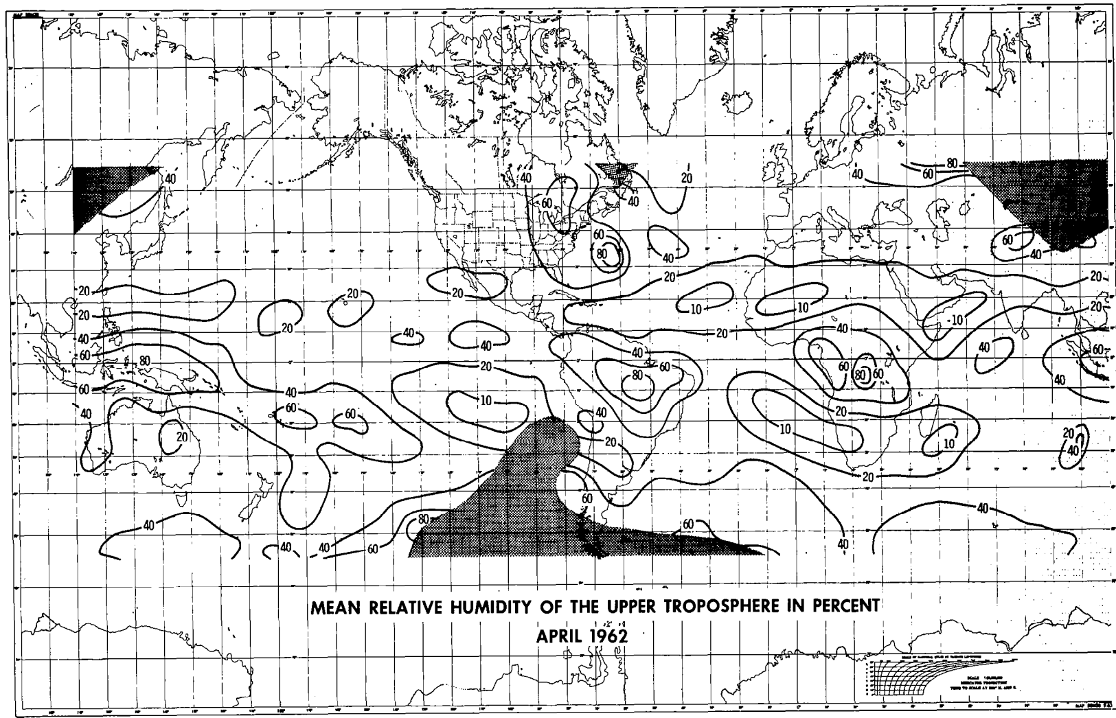
Fig. 4.5 : Quasi-global distribution of the mean relative humidity of the upper troposphere for April 1962.
