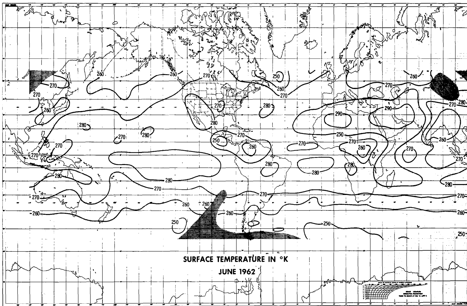
Fig. 4.10 : Quasi-global distribution of the (effective) surface temperature for June 1962.
