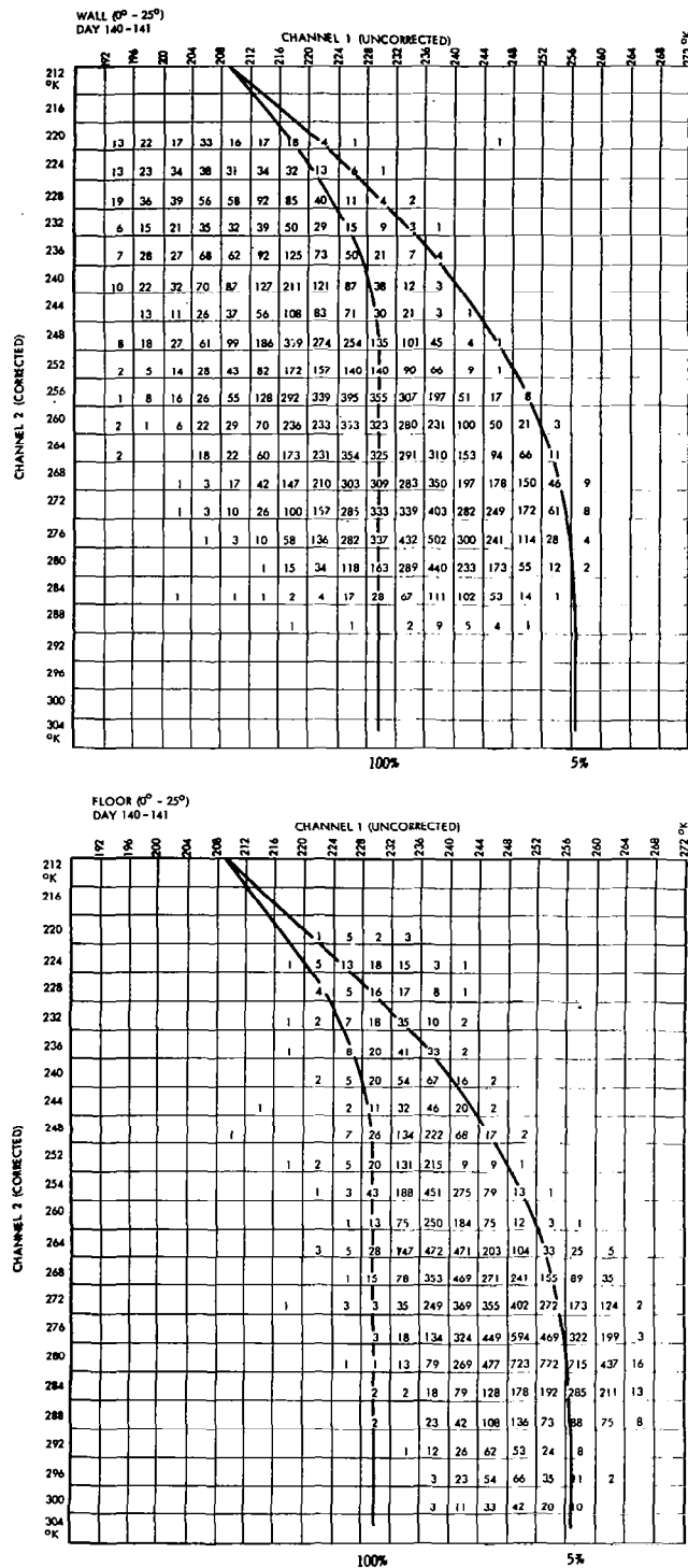
Fig.3.2: Scatter diagrams of simultaneous equivalent black body temperature measurements of channels 1 and 2 during the orbital days 140 and 141 at nadir angles N between 0^\circ and 25^\circ .
