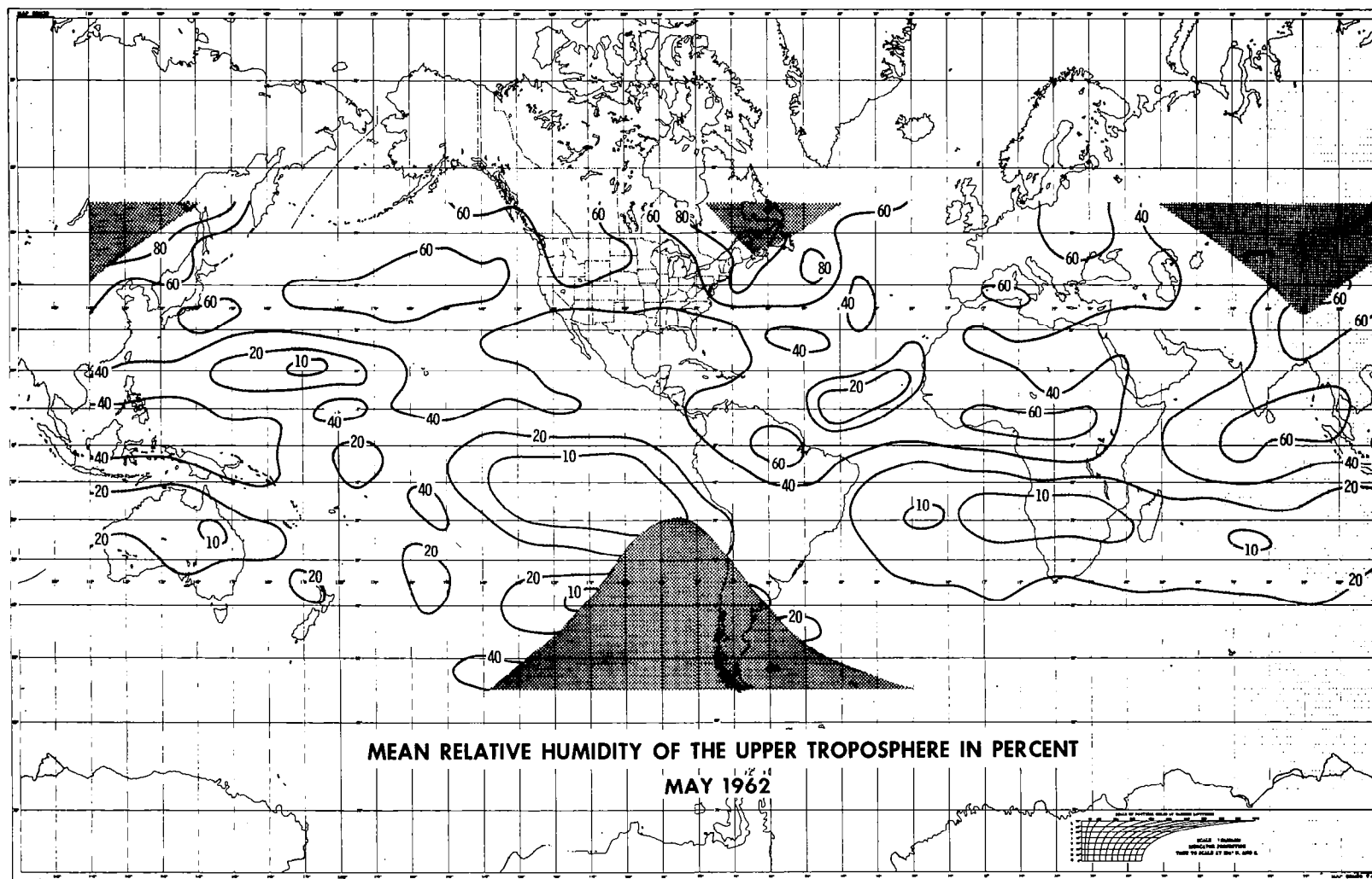
Fig. 4.7 : Quasi-global distribution of the mean relative humidity of the upper troposphere for May 1962.
