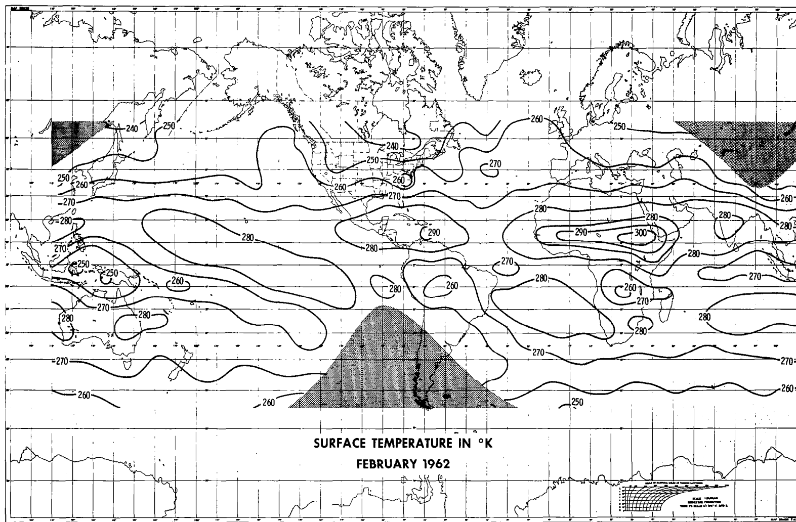
Fig. 4.2 : Quasi-global distribution of the (effective) surface temperature for February 1962.
