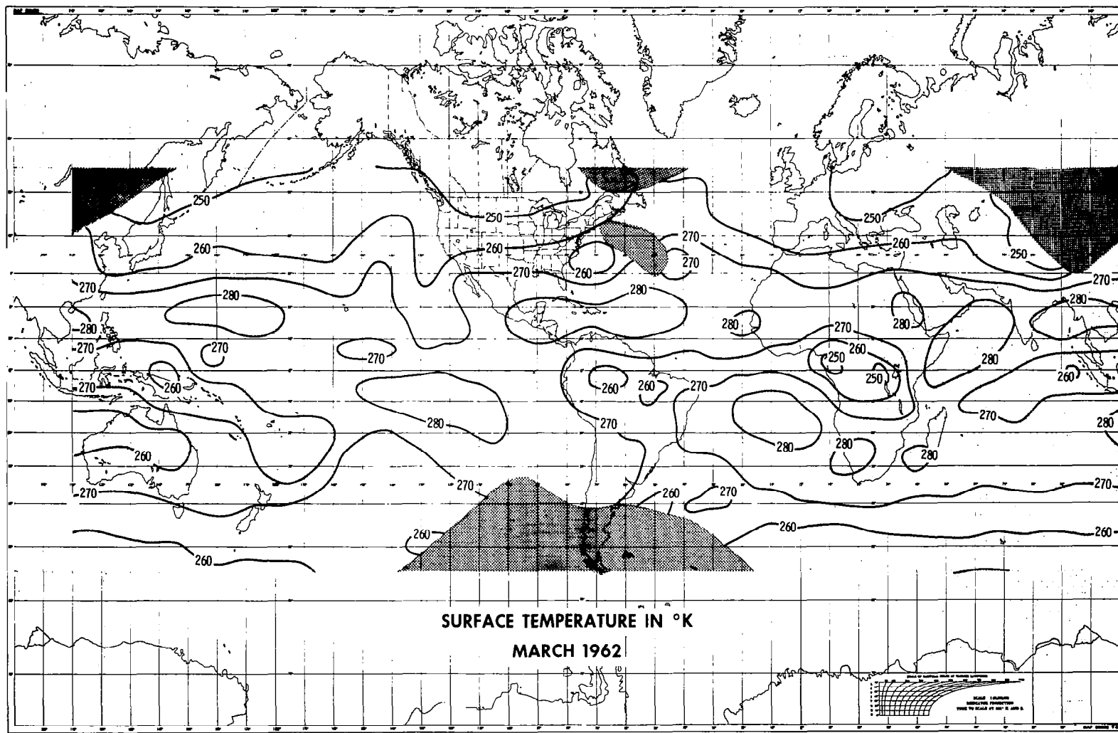
Fig. 4.4 : Quasi-global distribution of the (effective) surface temperature for March 1962
