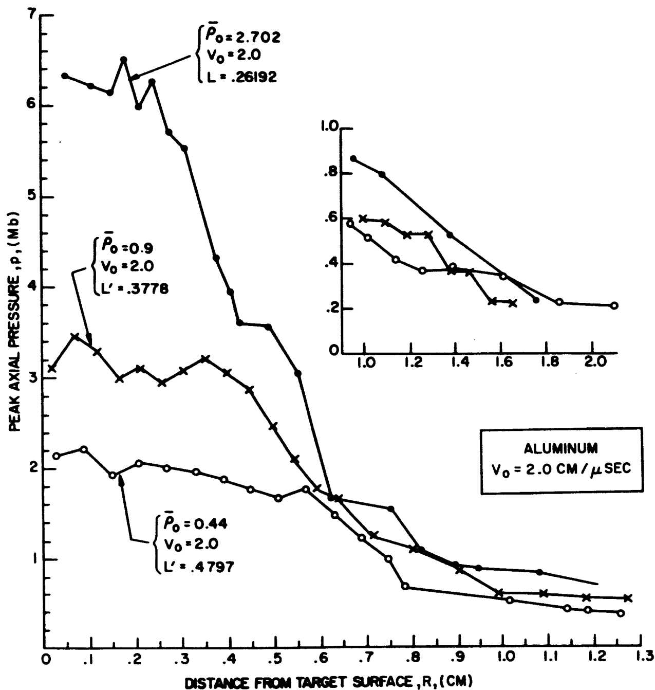
Figure 15. PICWICK I computations of peak axial pressures in aluminum target for impacts at 2 cm/ \mu sec of equi-mass aluminum projectiles of densities 2.702, 0.9 and 0.44 gm/cc. as functions of axial distance below target surface.
