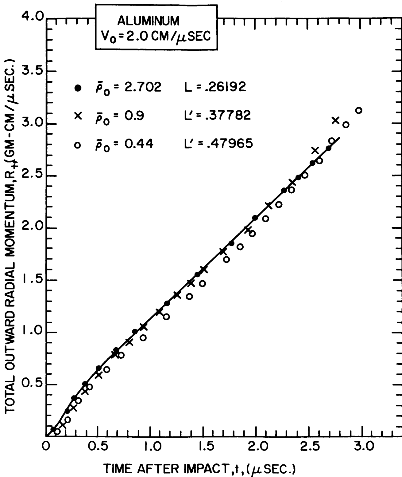
Figure 14. Total outward radial momentum for flow fields generated by equi-mass, equi-velocity aluminum projectiles of indicated bulk densities impacting an aluminum target at 2 cm/ \mu sec. for time t after impact.
