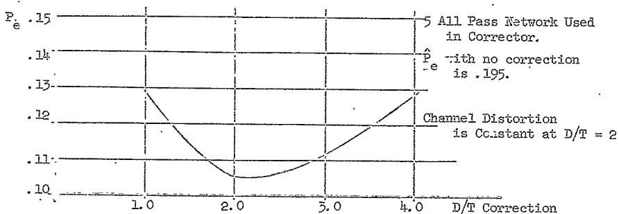
Figure 7-Sensitivity of All-Pass Correction to Channel - Corrector Mismatch
