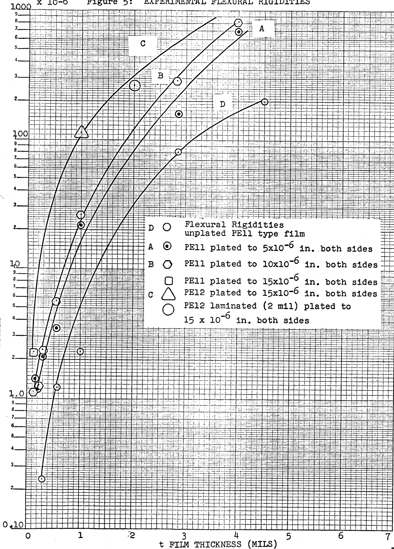
Figure 5: EXPERIMENTAL FLEXURAL RIGIDITIES
