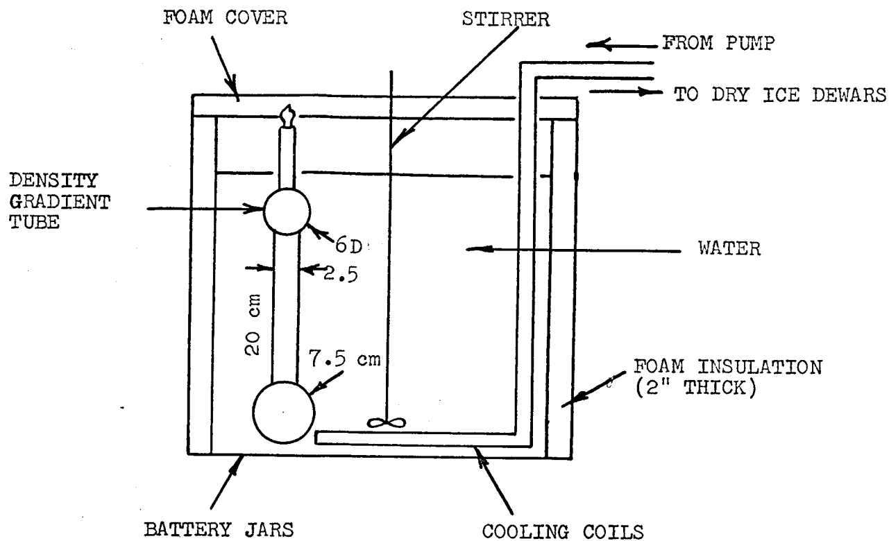
Figure 3: DENSITY GRADIENT APPARATUS
