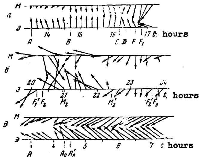
Fig. 2. - Vector of the magnetic field observed on Mariner-2 (M — in a plane perpendicular to the ecliptic, \mathcal{D} in the ecliptic plane; the direction at the Sun is to the right) for 3 periods.
