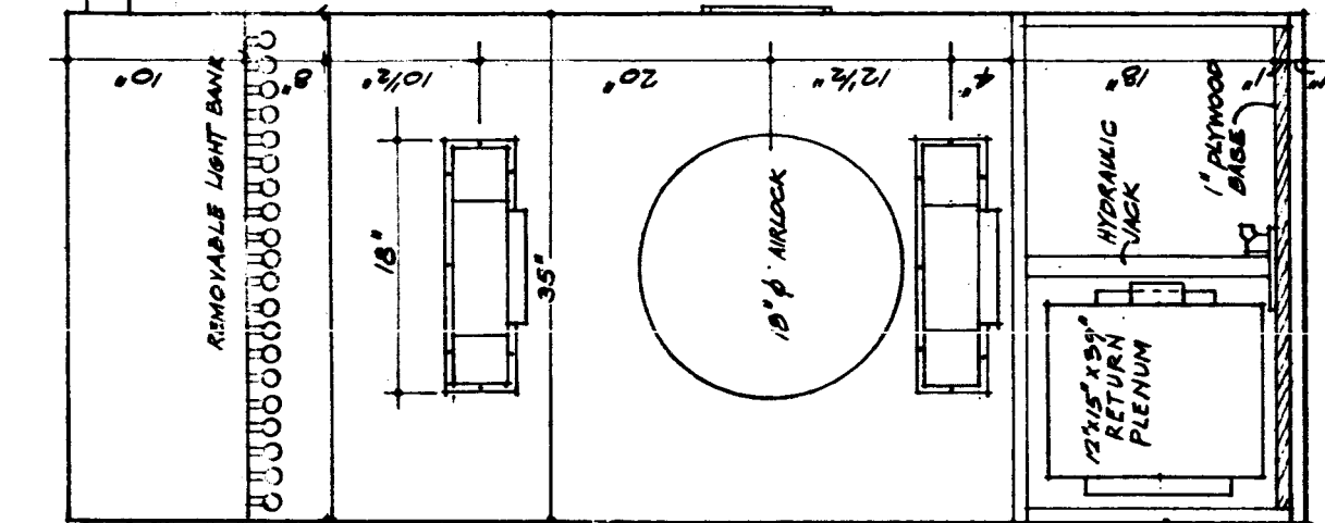
REDUCING Y DET. FOR DNG 2-B SCALE 1/2" = 1'-0"
