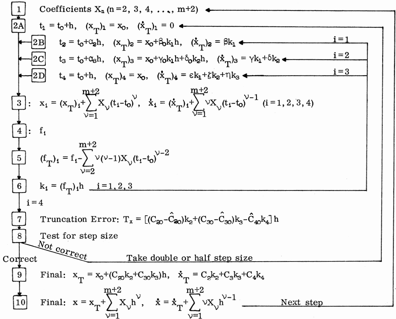
FIGURE 1. FLOW CHART
