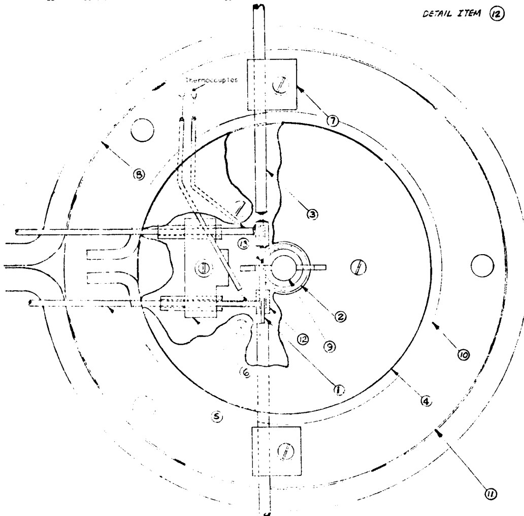
Fig. 4. Static Irradiation Cell.
