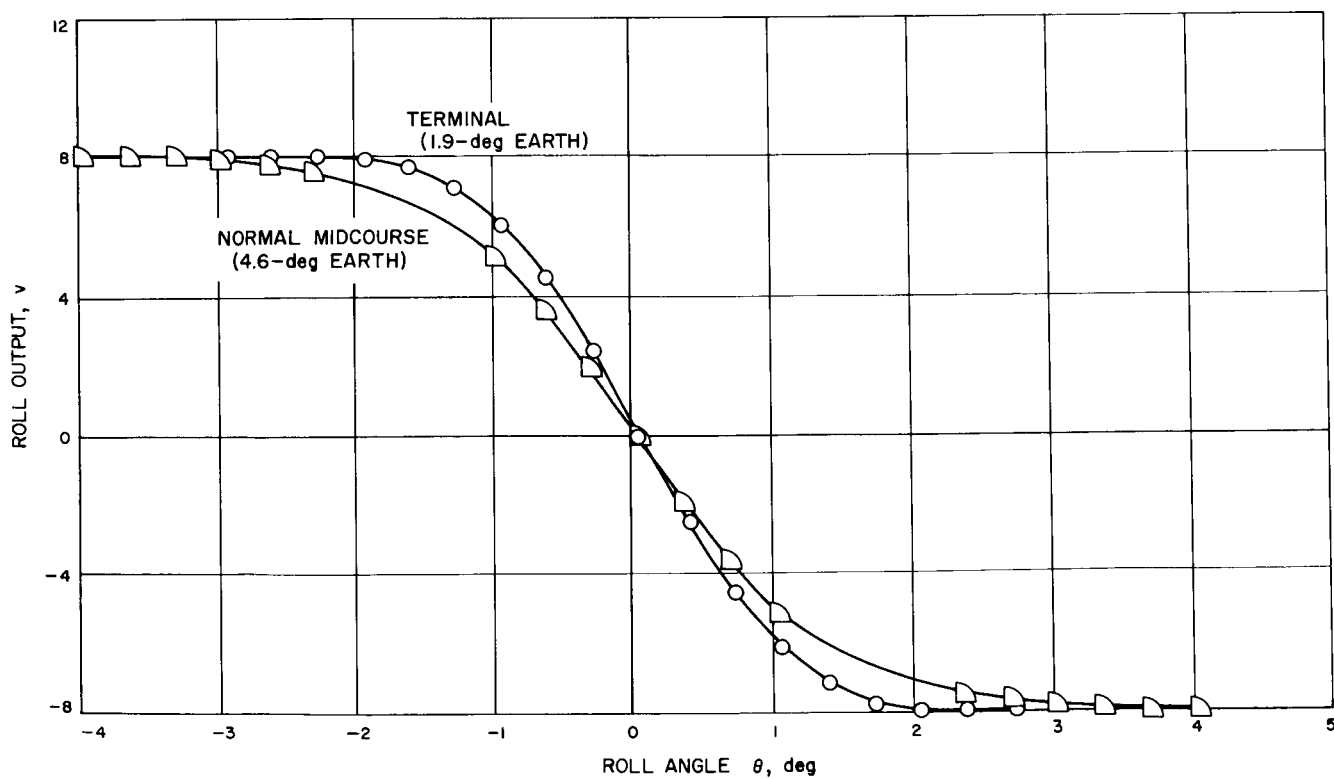
Fig. 32. Roll output versus roll angle
