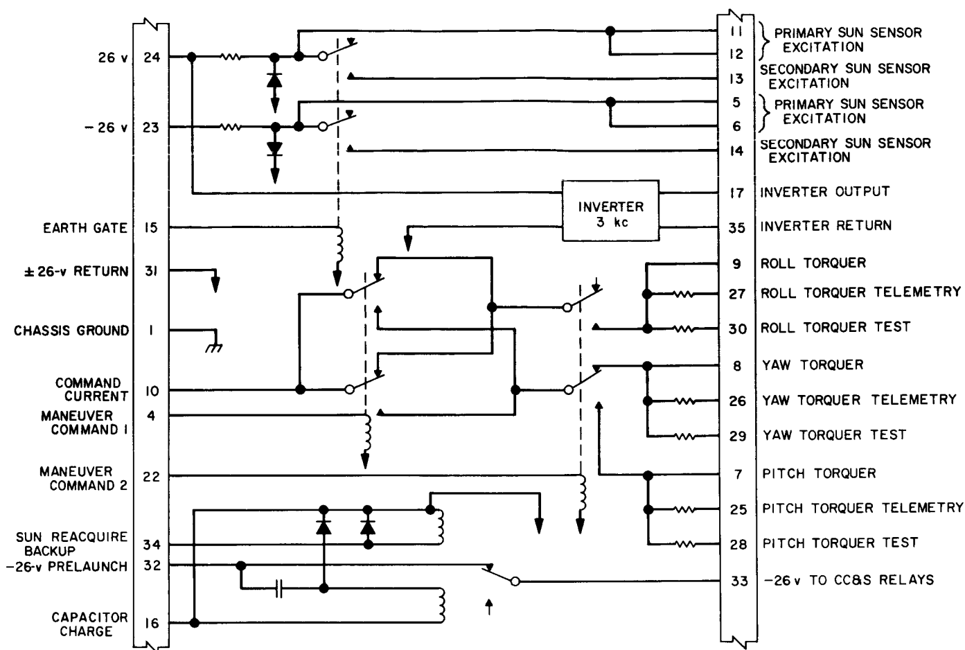
Fig. 70. Command switch and logic
