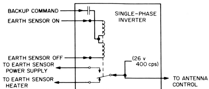
Fig. 21. Earth sensor power switching
