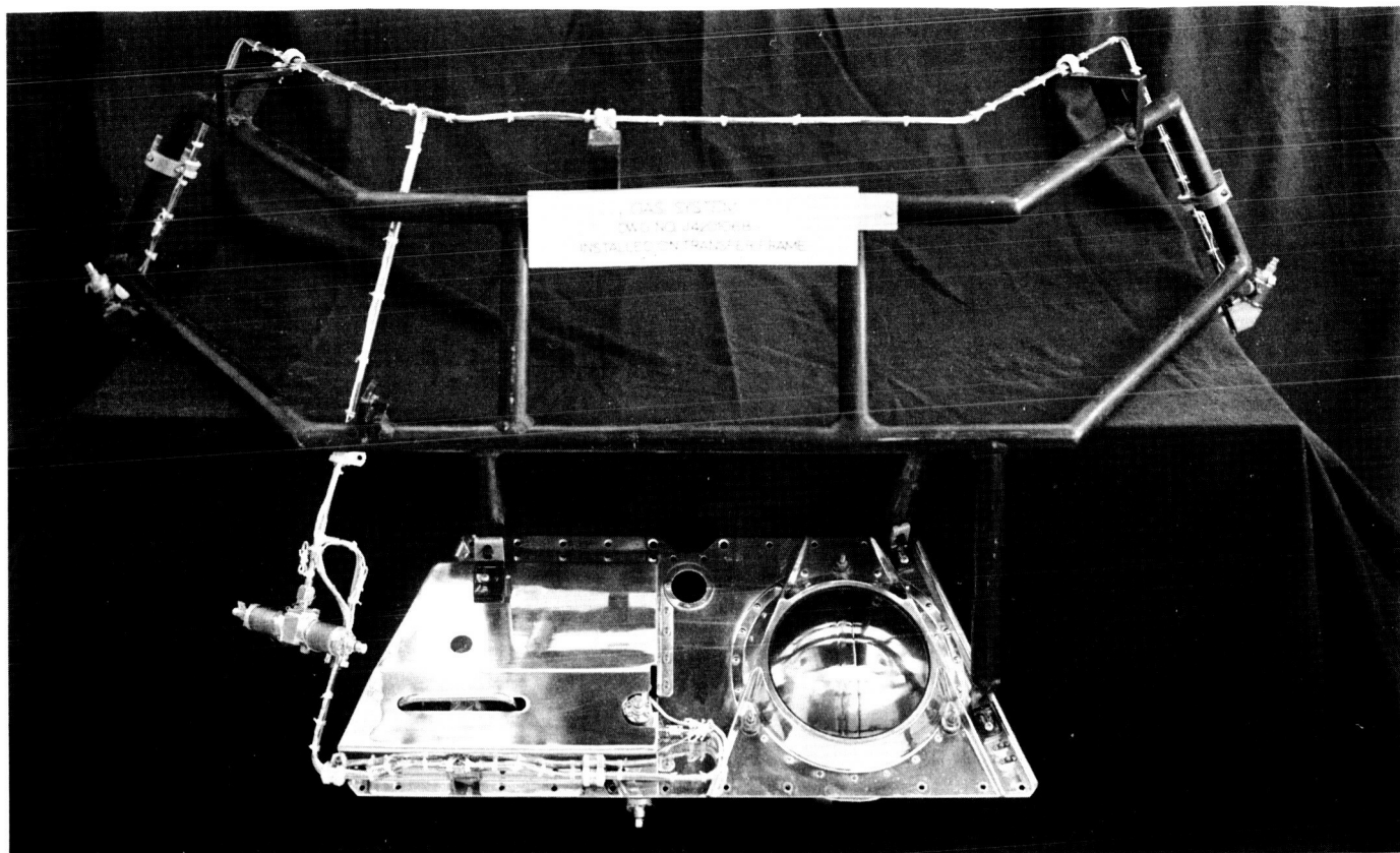
Fig. 60. Gas subsystem installed on transfer frame
