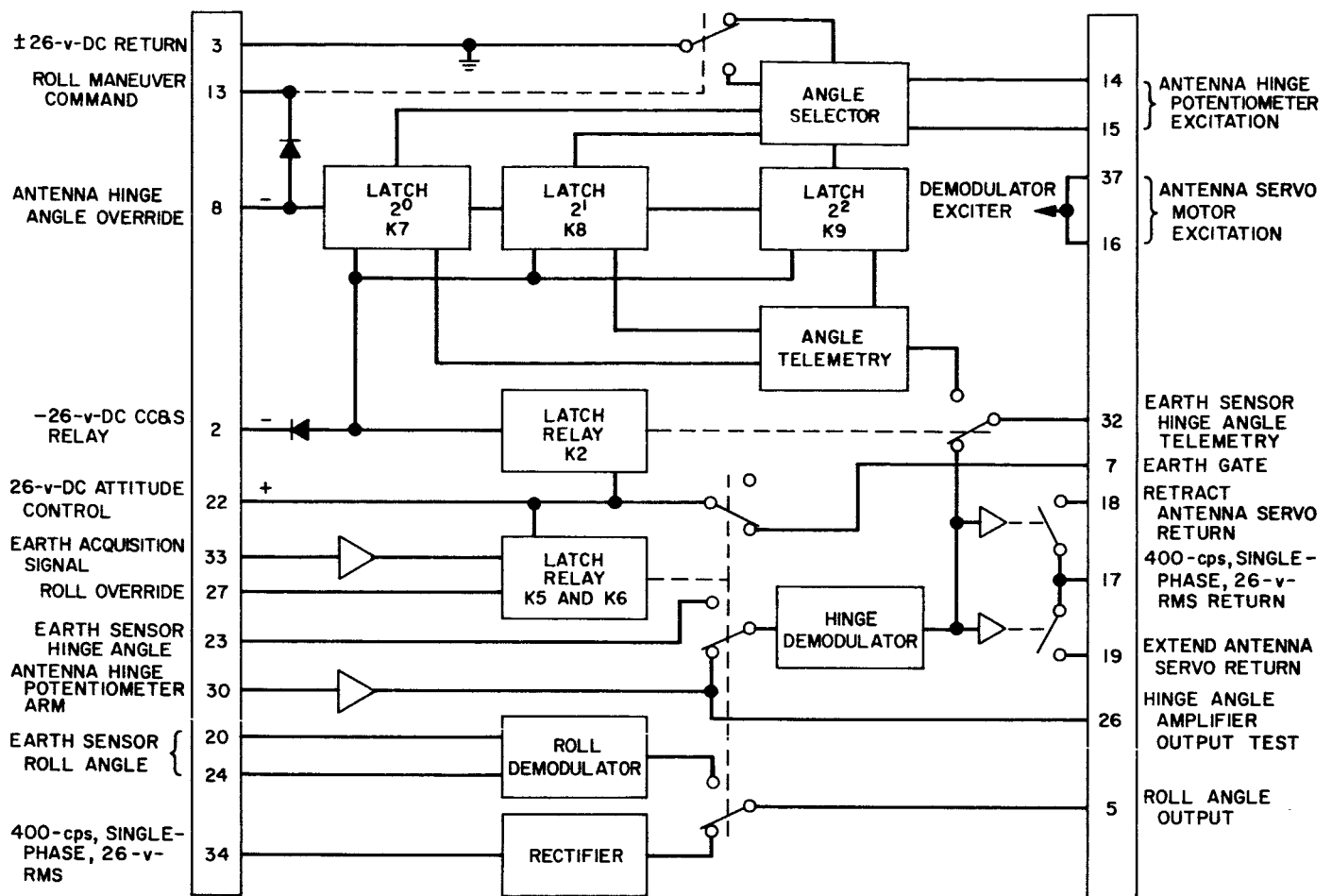
Fig. 71. Antenna control
