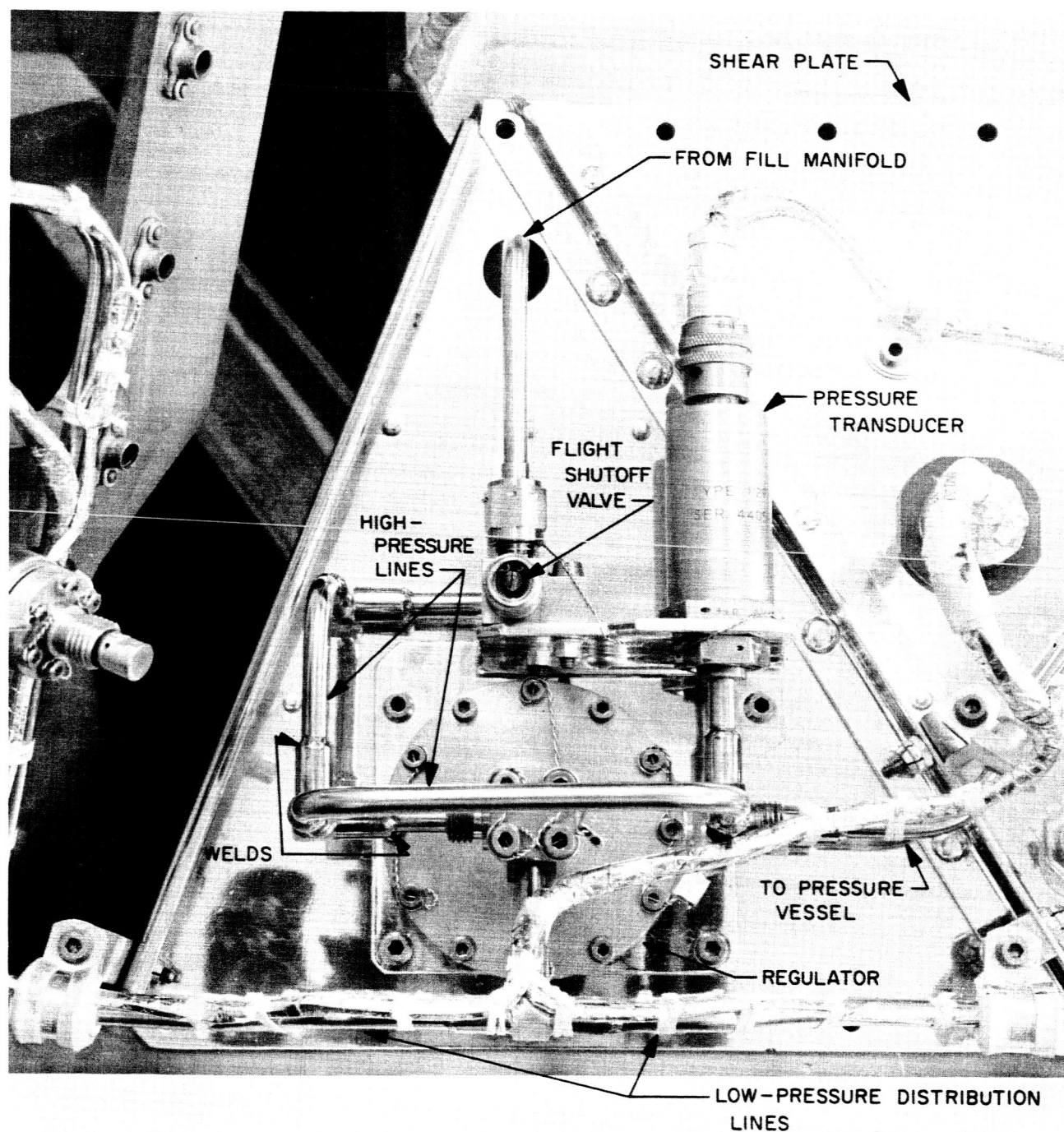
Fig. 53. Gas subsystem installed on handling frame
