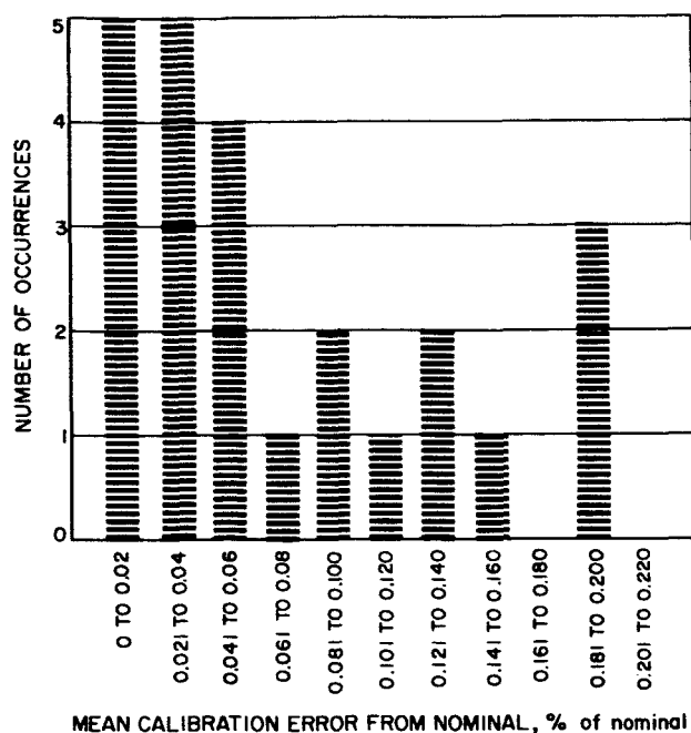
Fig. 64. Accelerometer mean digital calibration
