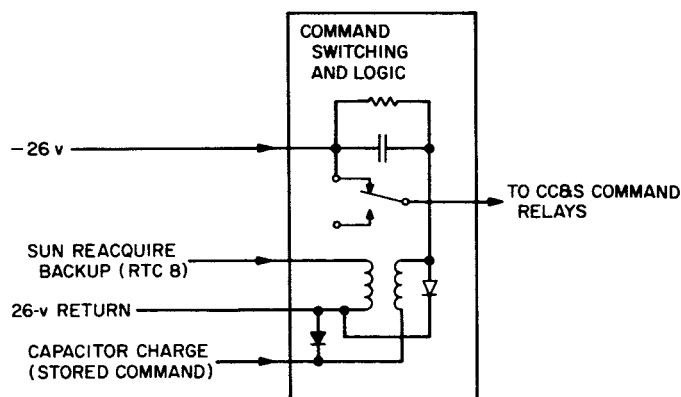
Fig. 8. Sun-reacquire backup details
