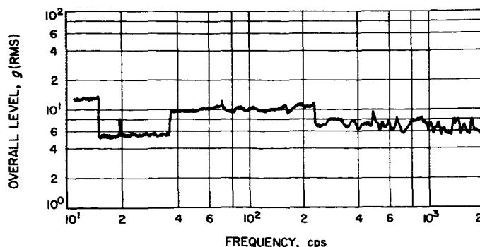
Fig. 54. Typical test level: y-axis (TA level)
