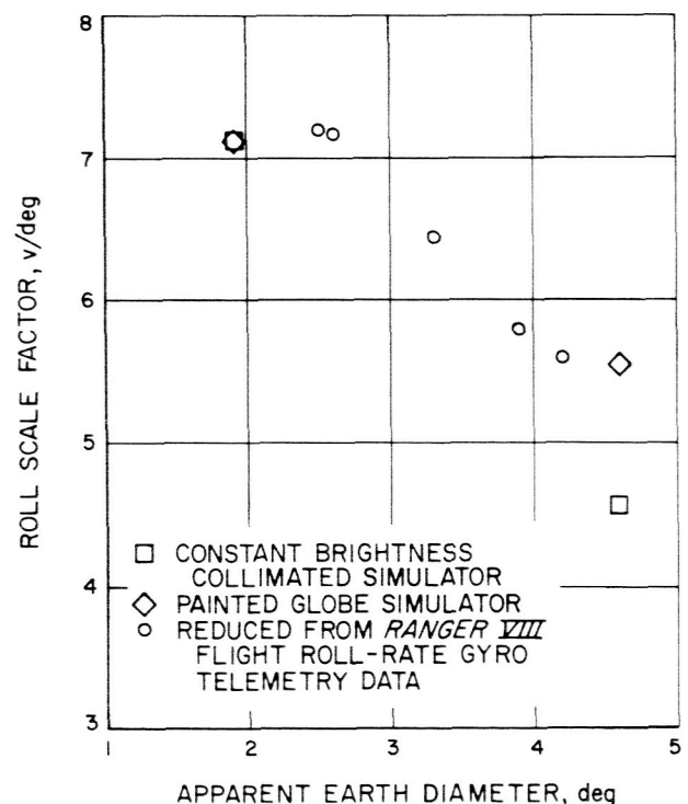
Fig. 38. Roll scale factor
