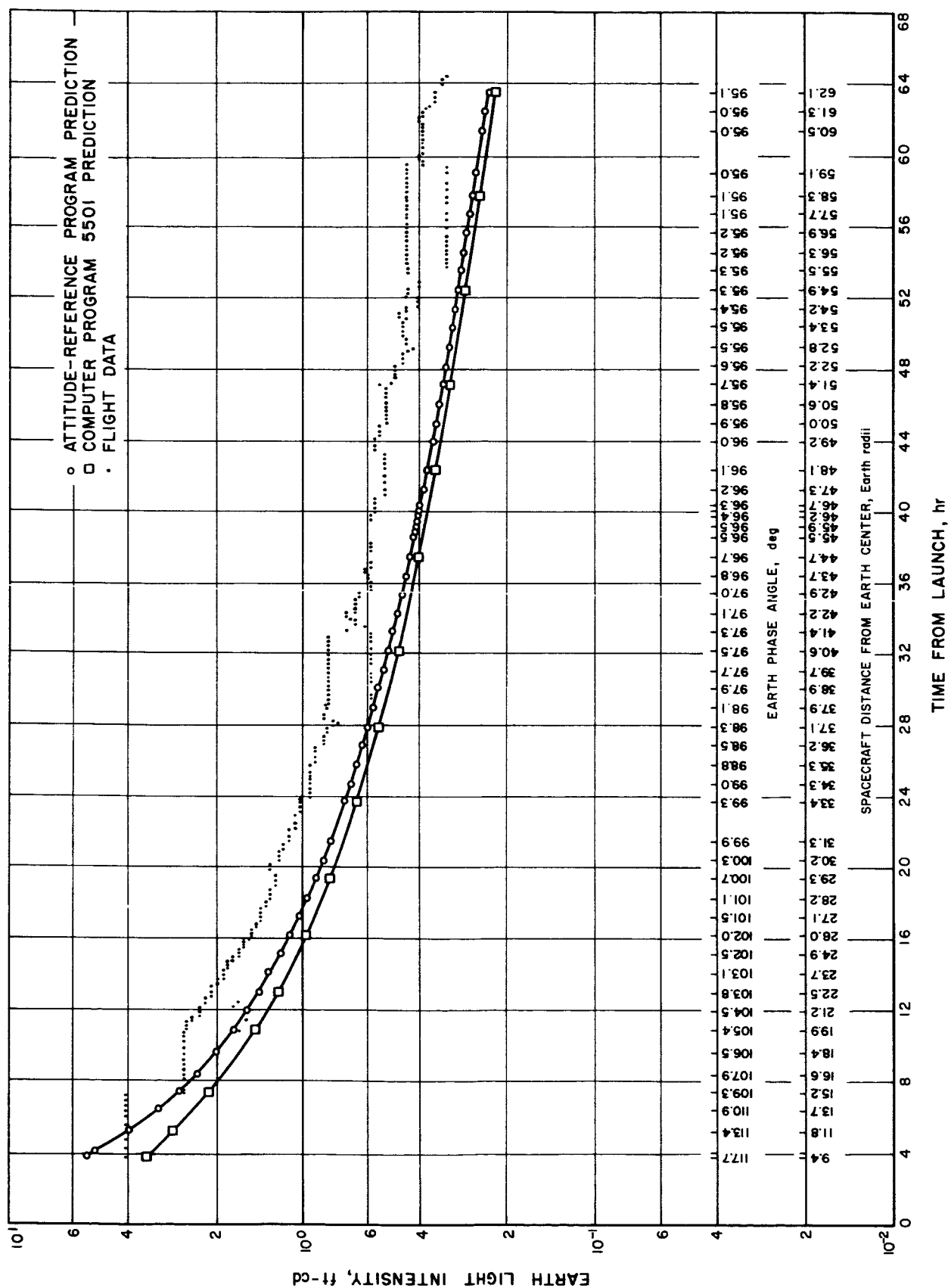
Fig. 43. Earth sensor light-intensity plot: Ranger IX
