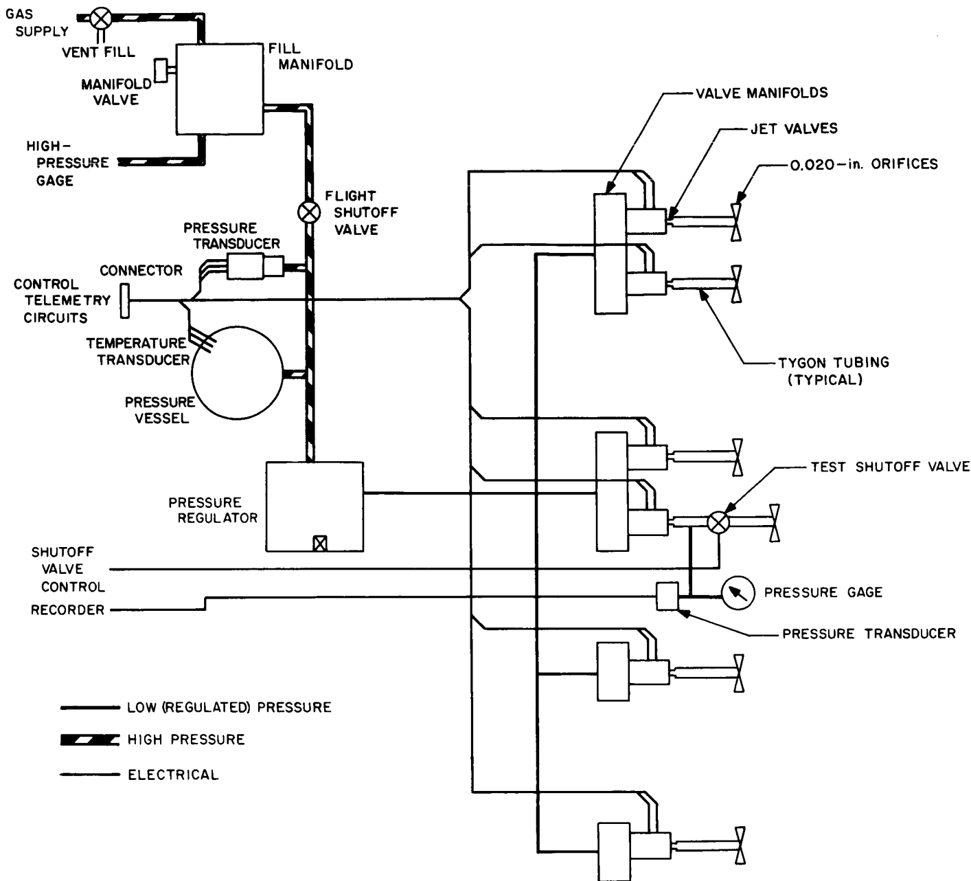
Fig. 55. Gas actuator assembly test setup
