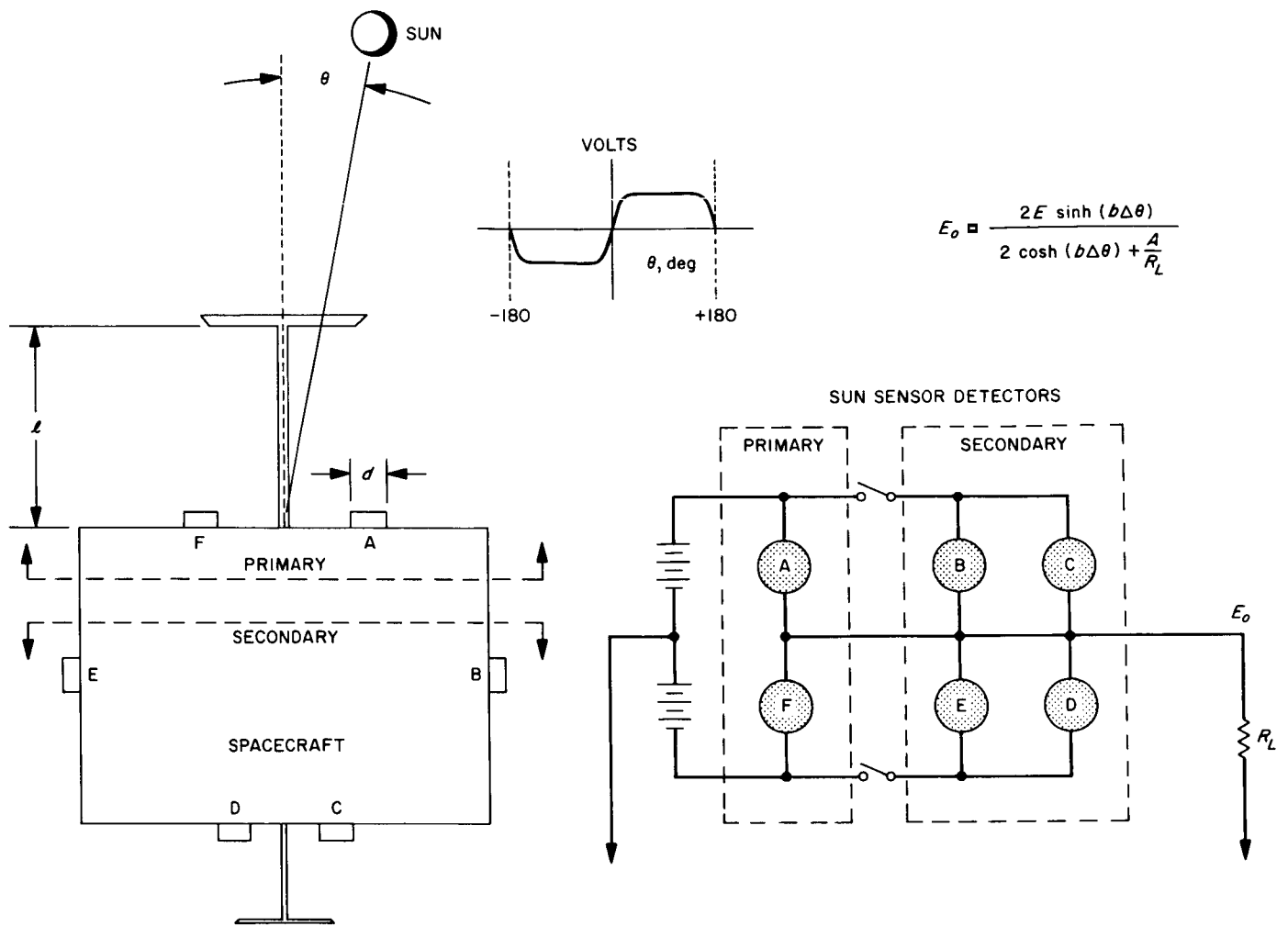
Fig. 44. Sun sensor schematic
