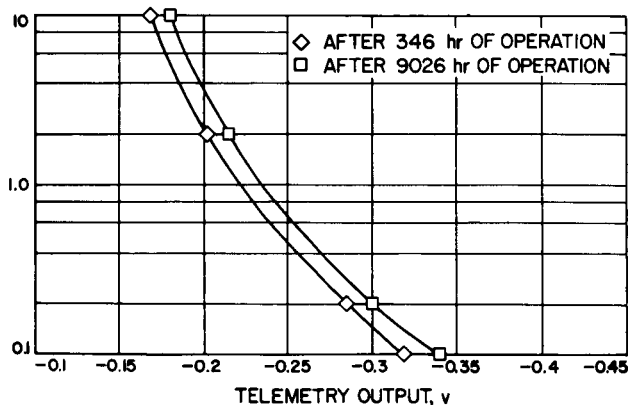
Fig. 29. Earth sensor life test results (S/N 39)
