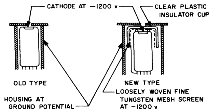
Fig. 16. PMT electrostatic shield
