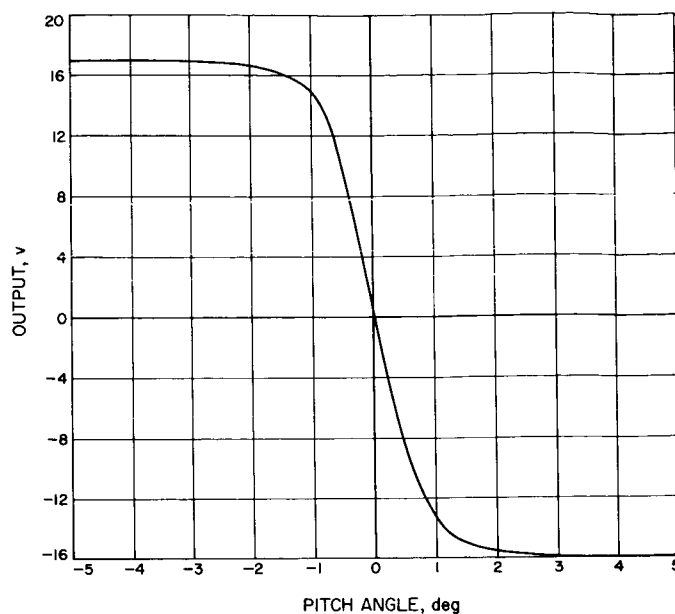
Fig. 46. Sun sensor flight calibration (pitch)
