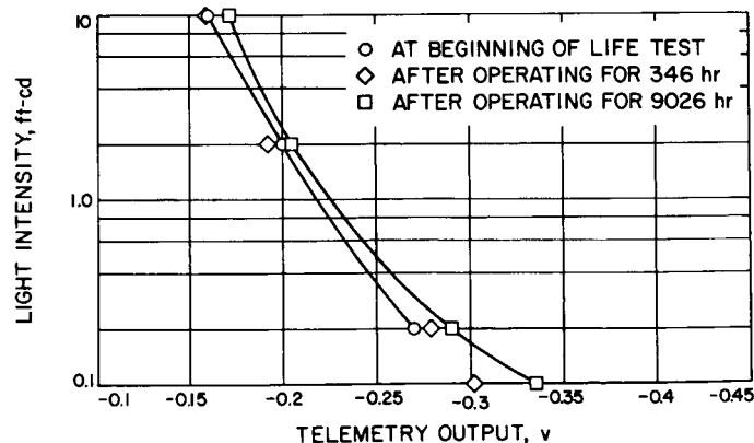
Fig. 30. Earth sensor life test results (S/N 42)
