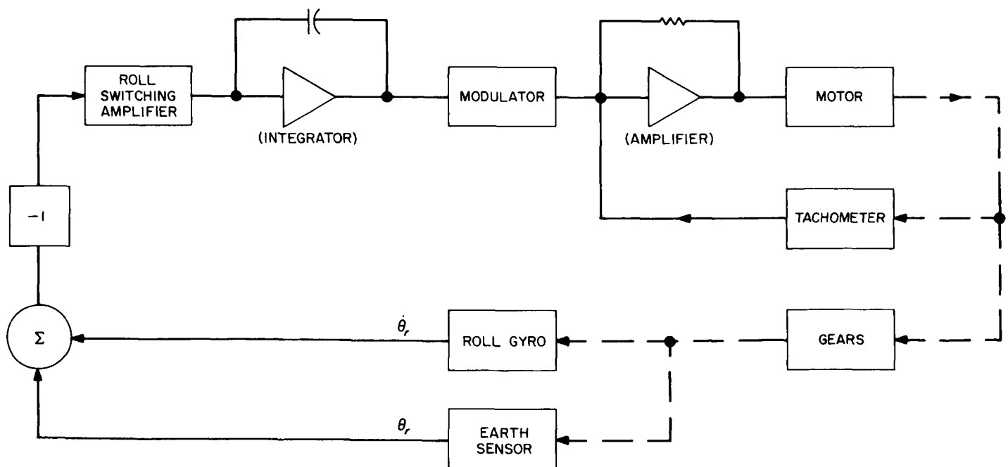
Fig. 75. Single-axis simulation
