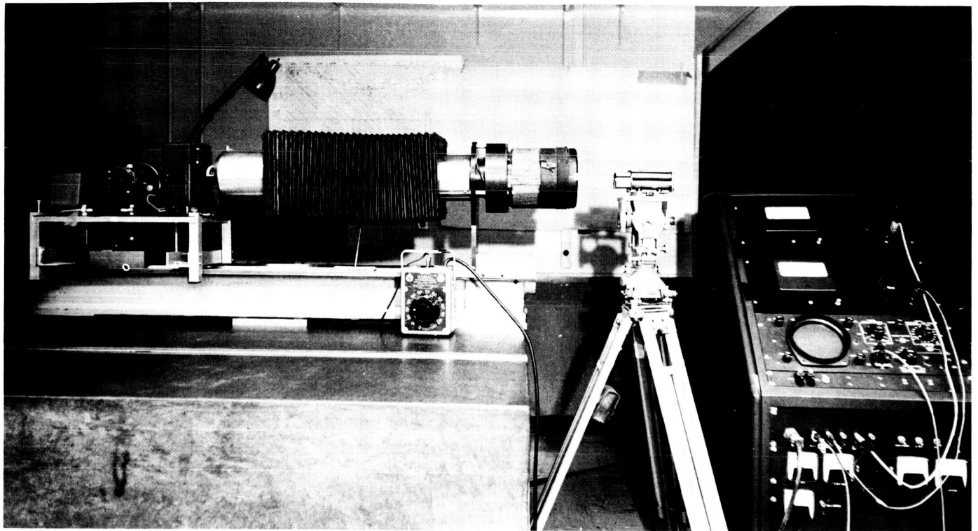
Fig. 25. Earth sensor mounted on T-2 theodolite
