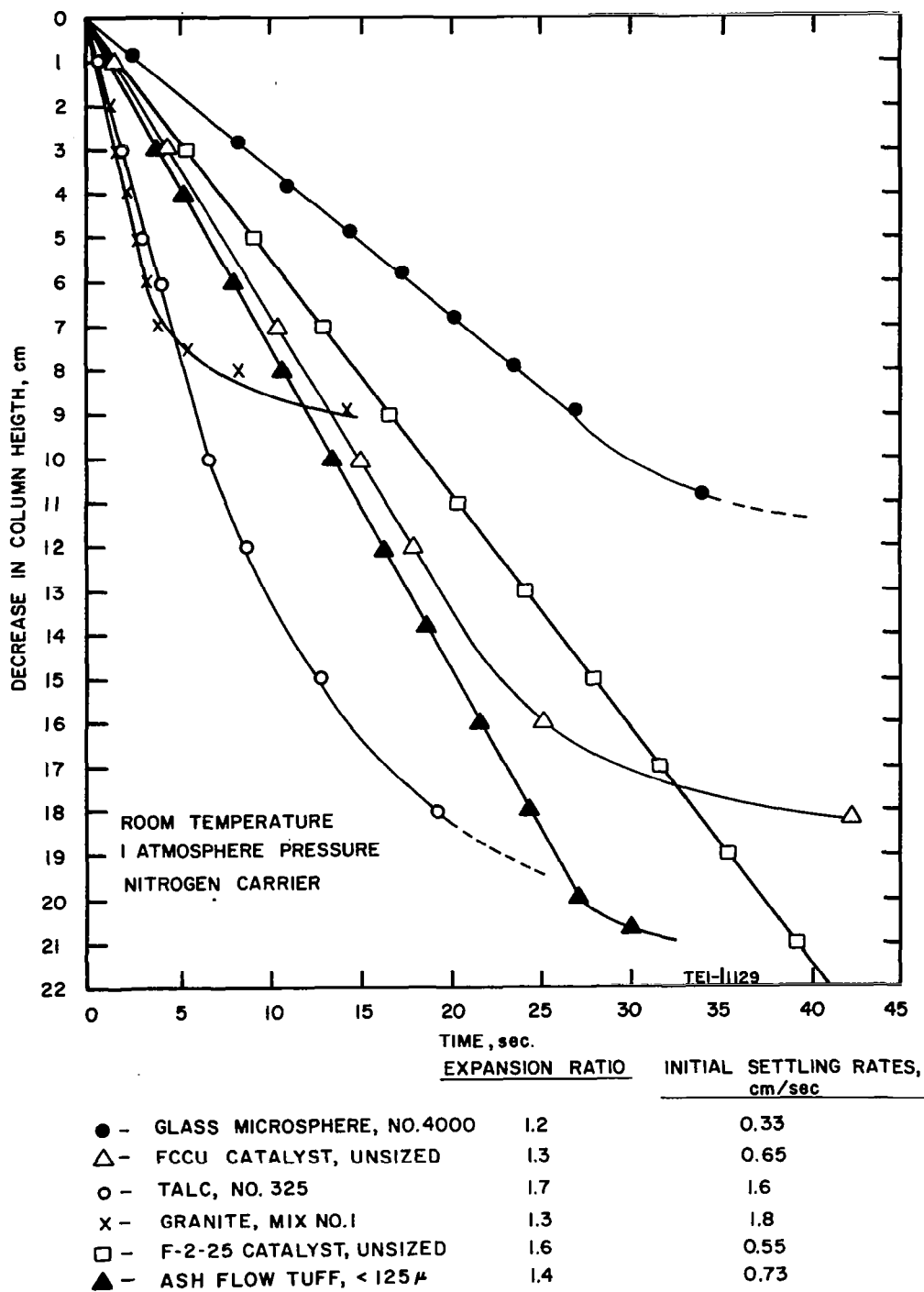
Fig. 11 Effect of Particle Shape on Settling Rates
