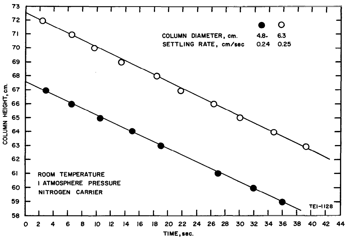
Fig. 14 Effect of Column Diameter on Settling Rates (Bed Material No. 2332.5 Glass Microspheres)
