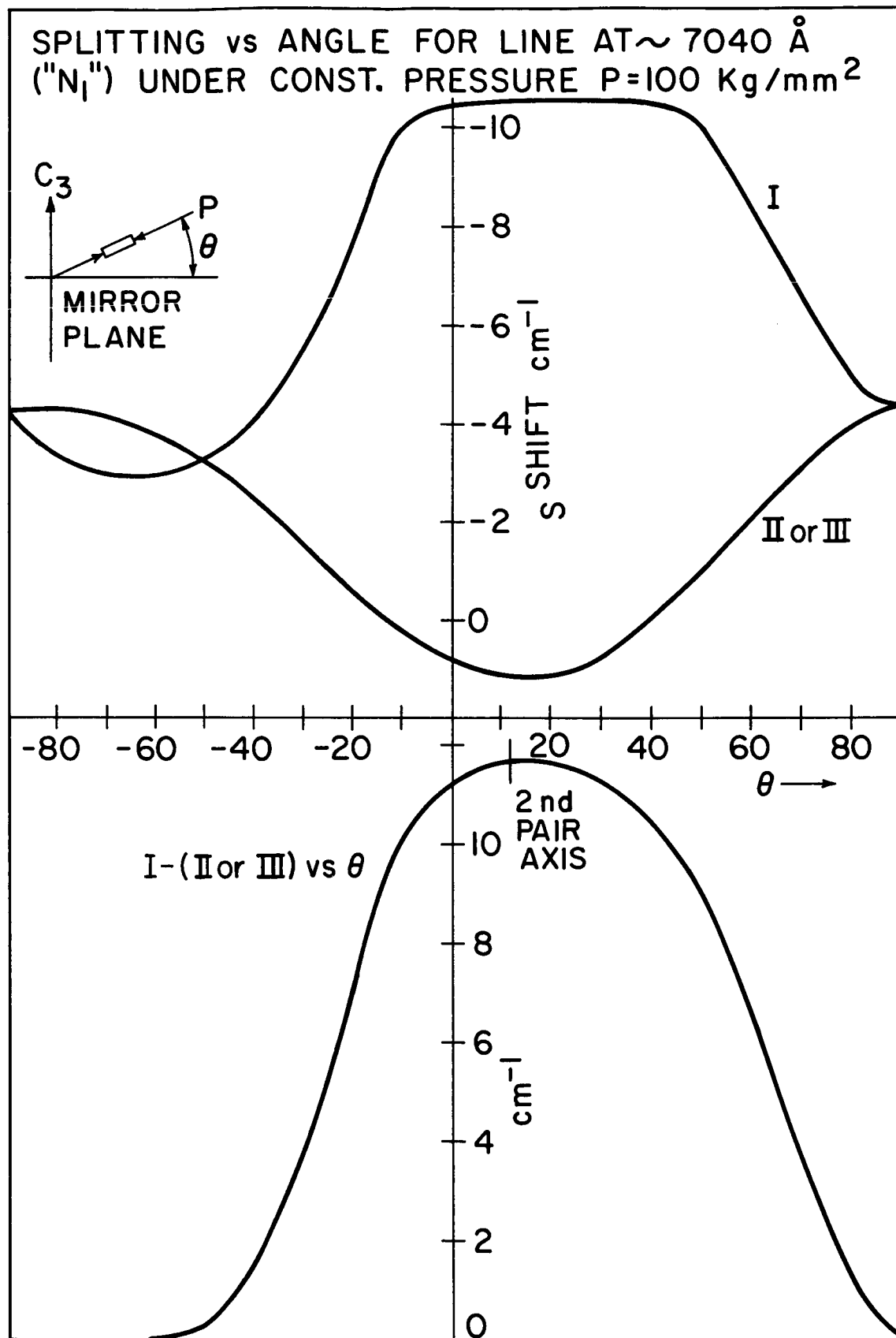
FIG. 3.13--N 1 splitting pattern and splitting curve.
