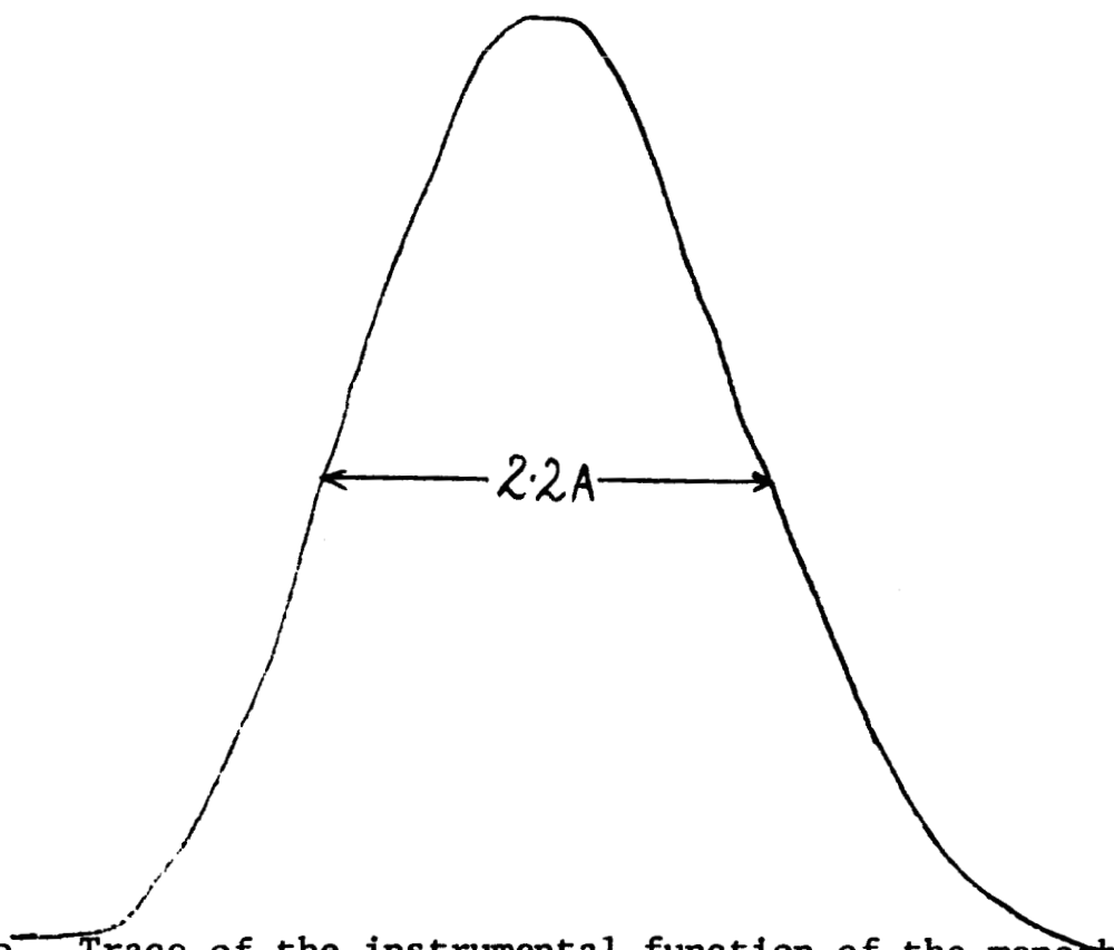
Fig. 10b. Trace of the instrumental function of the monochromator using the Fabry-Perot interferometer.
