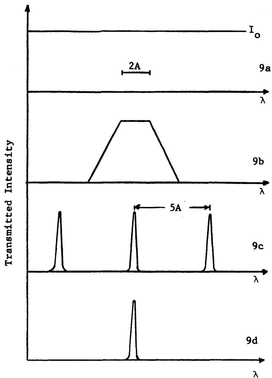
Figure 9a Intensity distribution of tungsten ribbon filament lamp over short wavelength interval.
