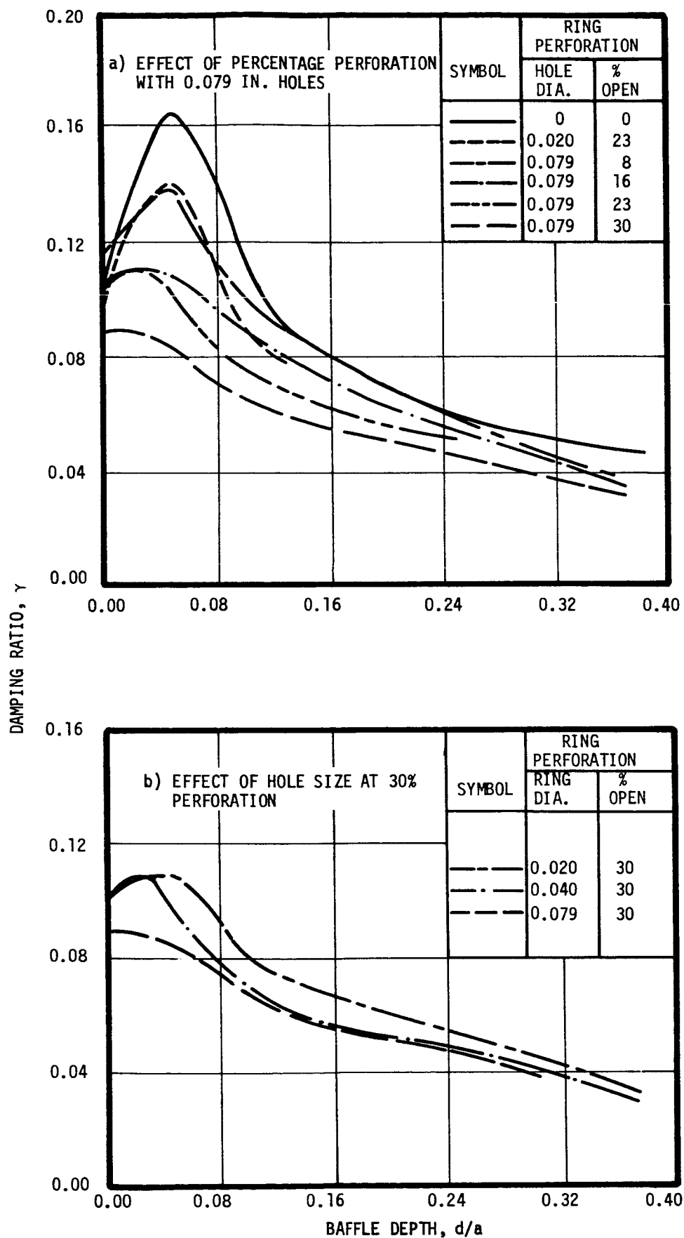
Figure 11. Damping Effectiveness as a Function of Baffle Depth (from Reference 6)
