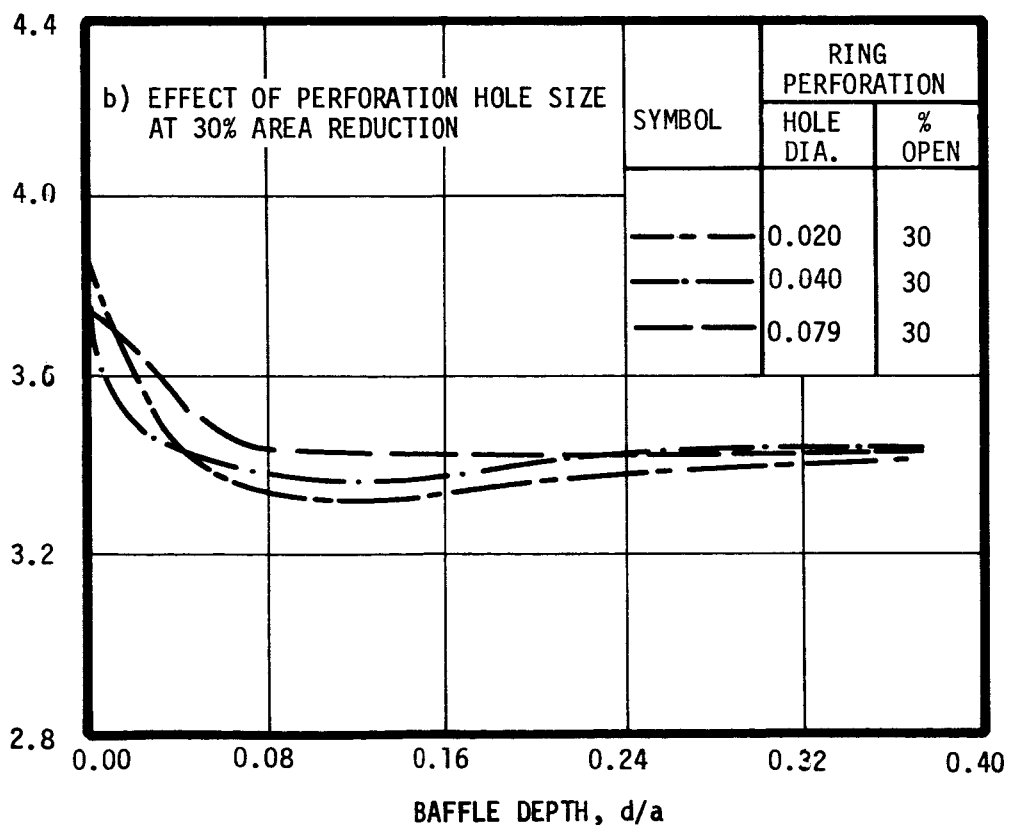
Figure 12. Liquid Resonant Frequencies as a Function of Baffle Depth (from Reference 6)
