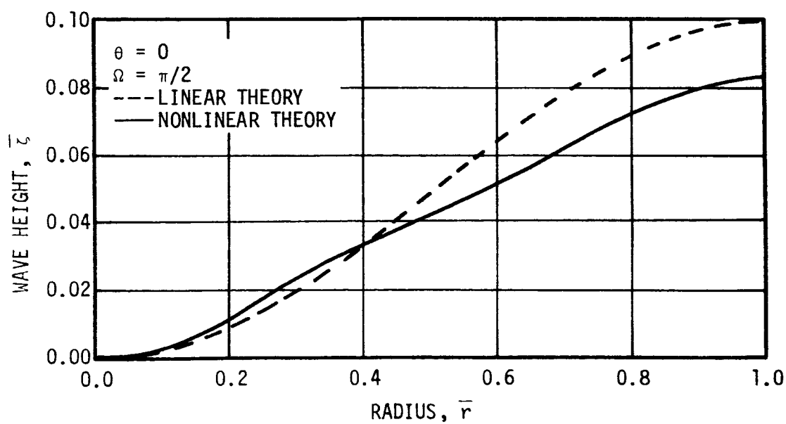
Figure 7. Wave Profile, \bar{\epsilon} = 0.1 , \bar{h} = 0.6
