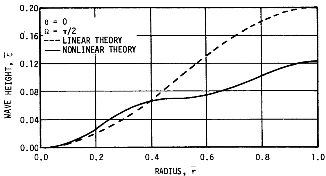
Figure 8. Wave Profile, \bar{\epsilon} = 0.2 , \bar{h} = 0.6
