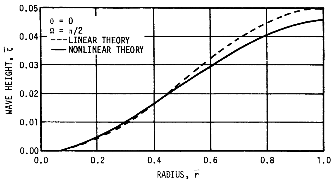
Figure 6. Wave Profile, \bar{\epsilon} = 0.05 , \bar{h} = 0.6
