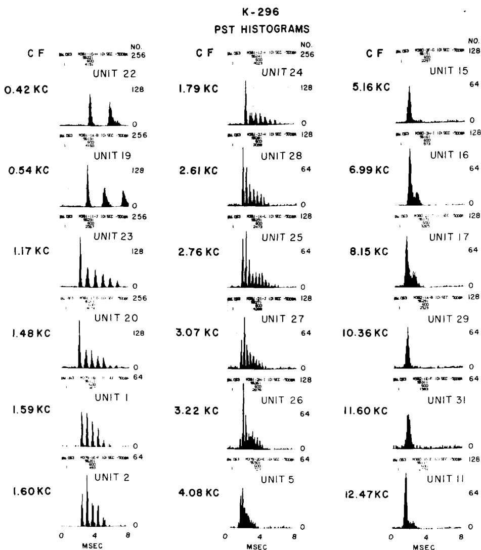
Figure 4.7 PST histograms of responses to clicks from 18 units obtained in a single cat.
