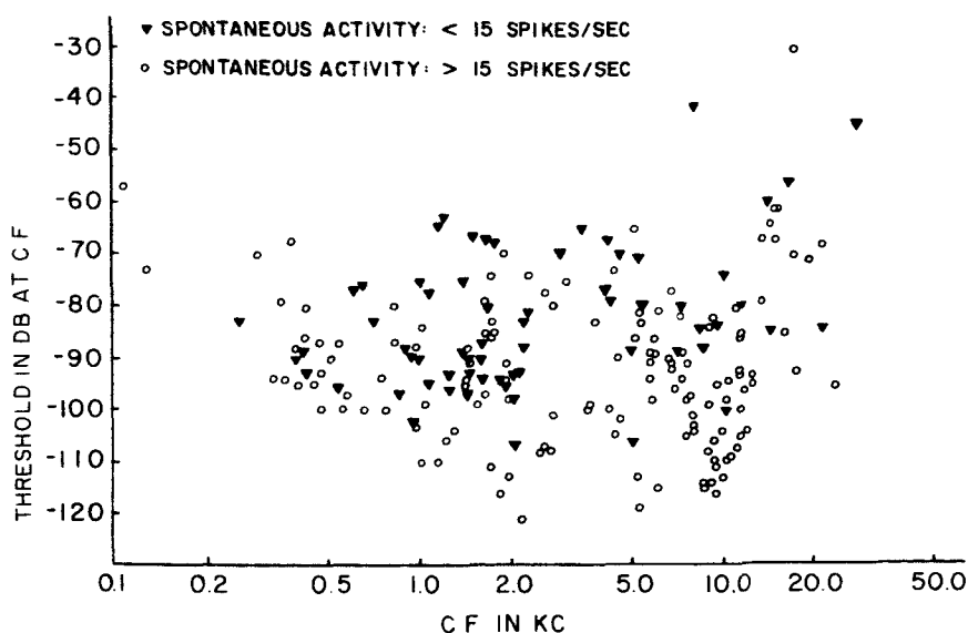
Figure 8.12 The threshold of 205 units from a large number of cats plotted against CF.
