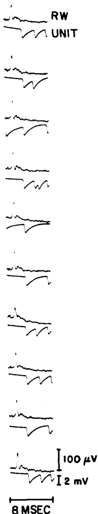
Figure 4.1 Time patterns of responses of a single unit to clicks displayed in a poststimulus-time histogram (PST histogram).
