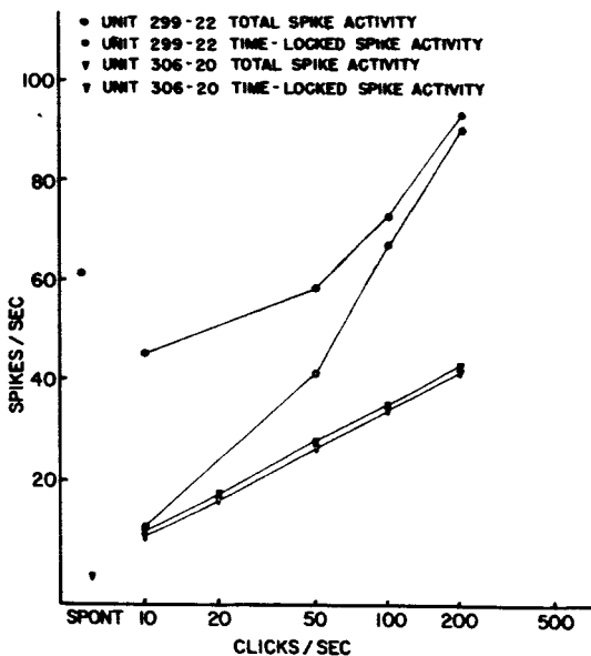
Figure 5.23 Rate of activity plotted against click rate for 2 units, one with a low rate of spontaneous activity, the other with a relatively high rate of spontaneous activity.
