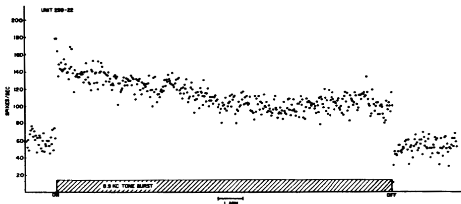
Figure 6.7 Changes in the rate of discharge of a unit with high CF (8.9 kc) when a tone burst of 13 minutes' duration is presented.
