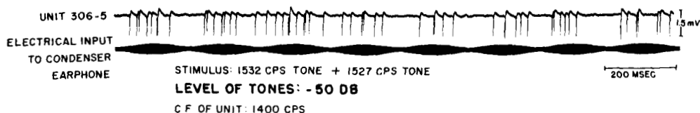
Figure 9.6 Spike trains of a unit in response to a mixture of 2 tones that beat at 5 cycles/sec.
