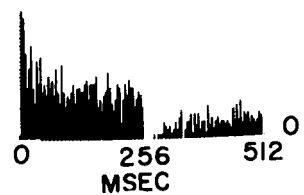
Figure 6.2 Response patterns of a unit to tone bursts as a function of stimulus level.
