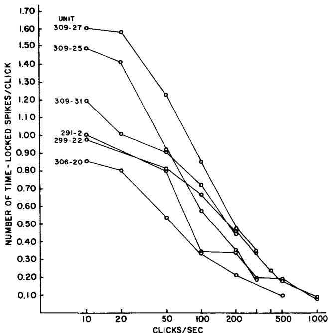
Figure 5.24 The number of time-locked spikes/click plotted against clicks/sec.
