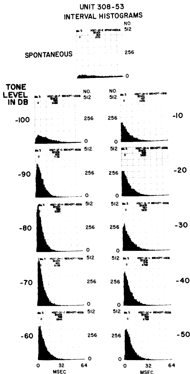
Figure 6.8 Interval histograms of discharges from a unit as the level of a continuous tone at 9.8 kc (CF) is changed in 10-db increments.
