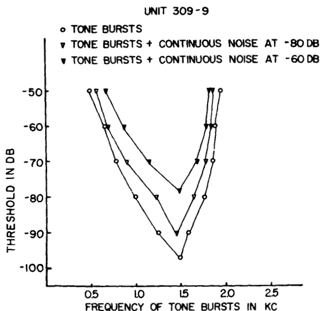
Figure 9.5 The effect of broadband continuous noise on the tuning curve. Tuning curves were taken under normal conditions and also in the presence of broadband noise at 2 different levels. The frequency scale is linear. Similar results are obtained for units with high CF.
