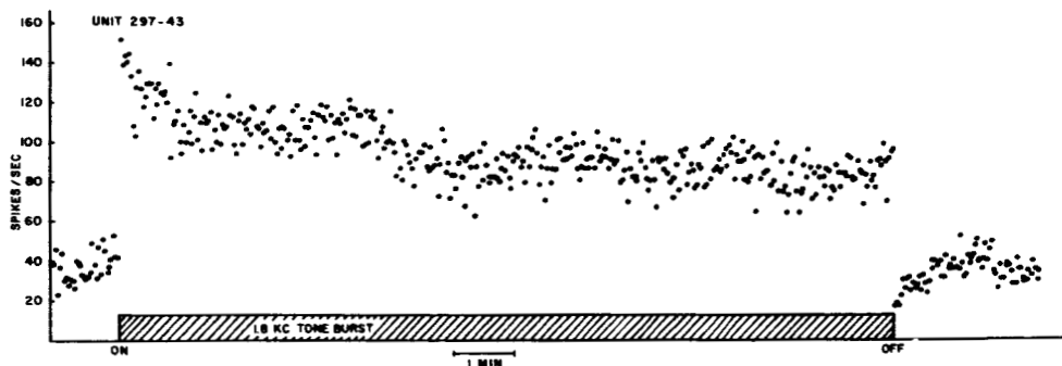
Figure 6.6 Changes in the rate of discharge of a unit with low CF (1.8 kc) when a tone burst of 13 minutes' duration is presented.
