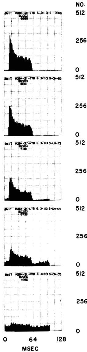
Figure 9.4 Masking of responses to tone bursts by broadband noise.
