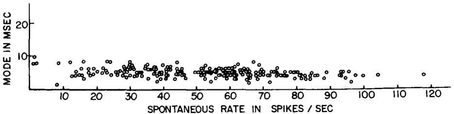
Figure 8.9 The mode of the interval histograms of spontaneous activity plotted against rate of spontaneous discharges for 227 auditory nerve fibers.
