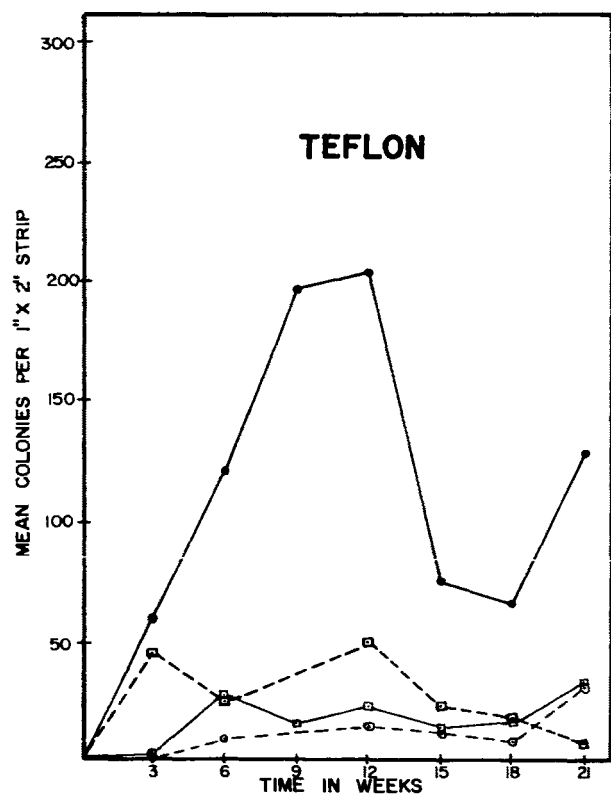
FIGURE II FLUCTUATIONS IN LEVELS OF CUMULATIVE MICROBIAL CONTAMINATION ON PLASTIC MATERIALS EXPOSED OVER A 21 WEEK PERIOD IN UNIVAC ROOM D.
