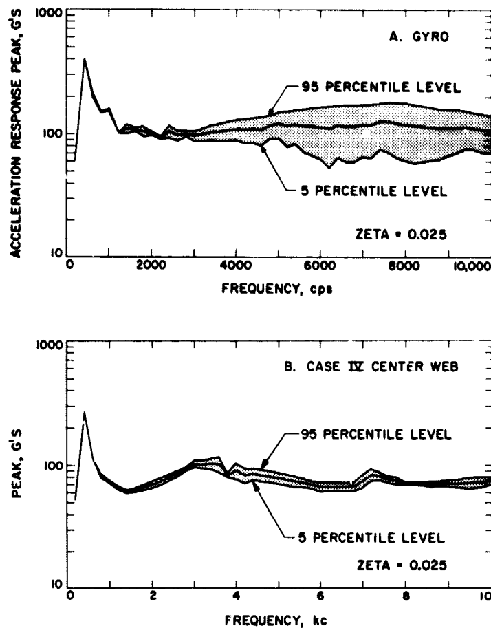
Fig. 17. Percentile levels of shock spectra, Ranger Case IV TA assembly shock
