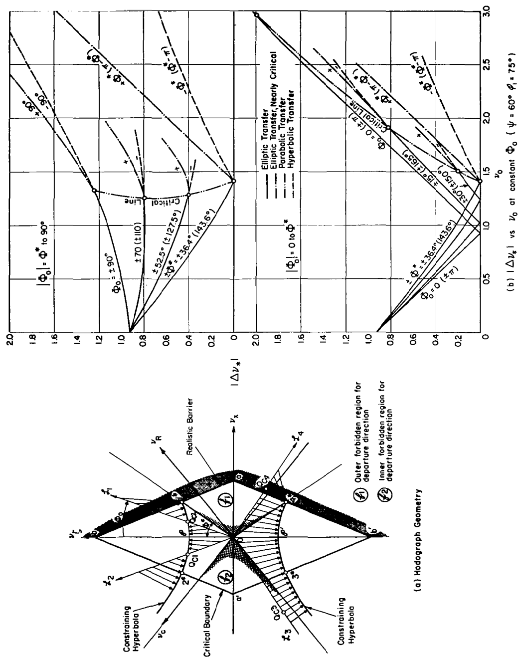
Fig. 10. Variation of the minimum velocity increment with the initial velocity vector at constant direction and varying magnitude.
