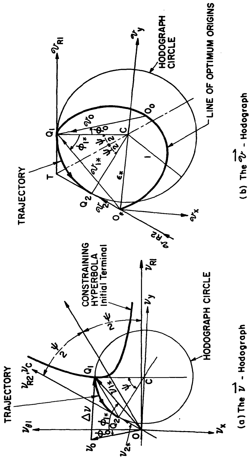
Fig. 20. The optimum trajectory hodograph for transfer to infinity.
