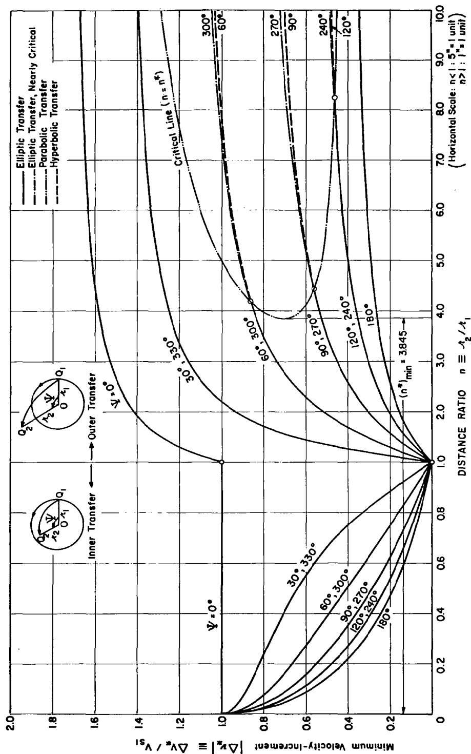
Fig. 22. Minimum velocity-increment for the transfer from a circular orbit to a coplanar point.
