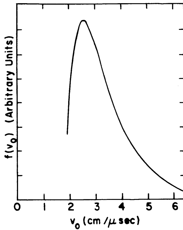
FIG. 29 : ION VELOCITY DISTRIBUTION DERIVED FROM VELOCITY PROBE DATA
