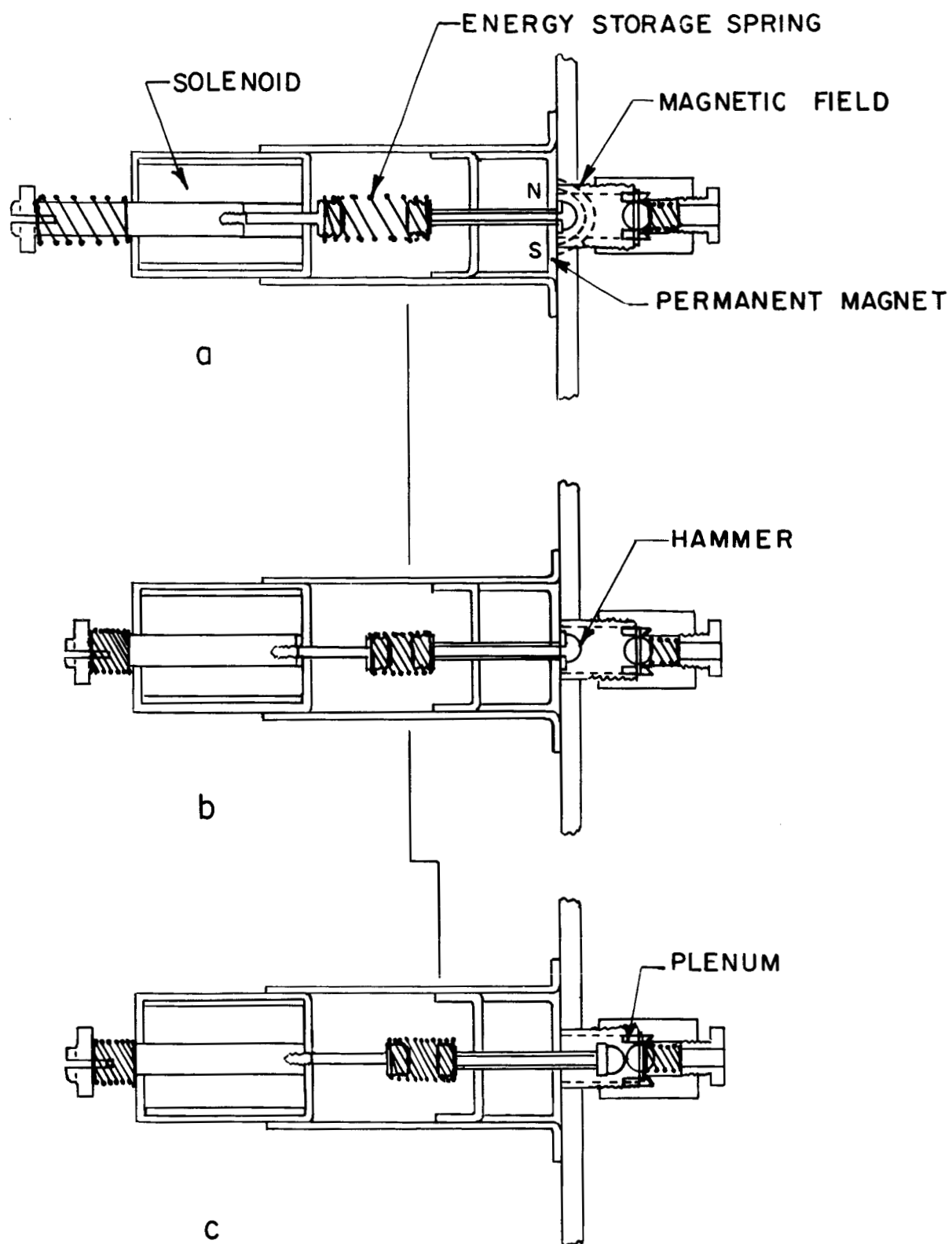
FIG. 34 : SOLENOID - COCKED, SPRING-ACTUATED VALVE
