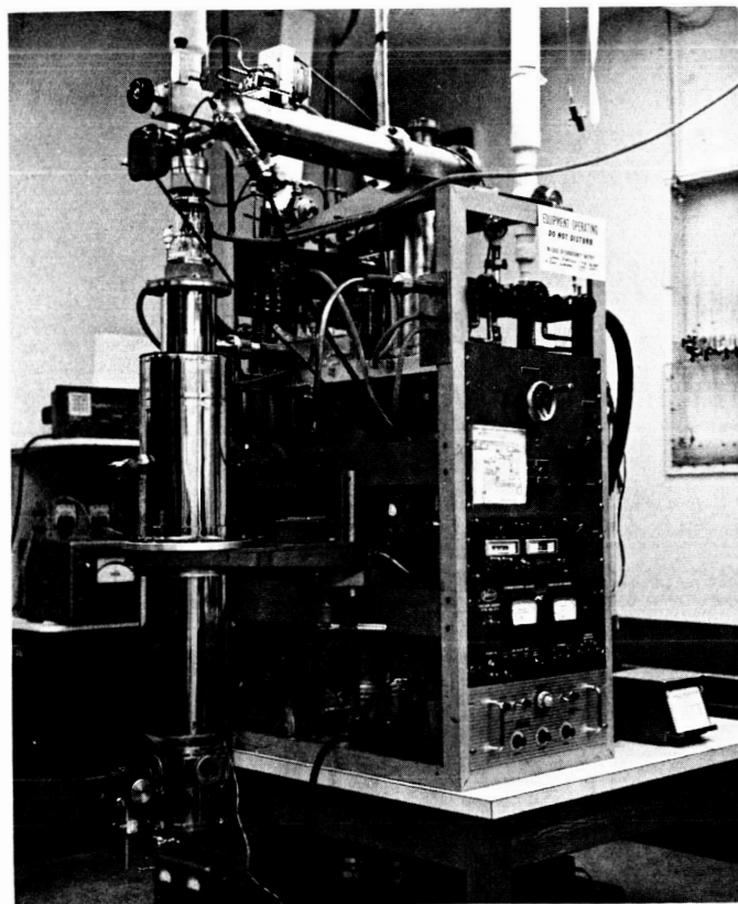
Fig. 7. Cryogenic gyro in Dewar
