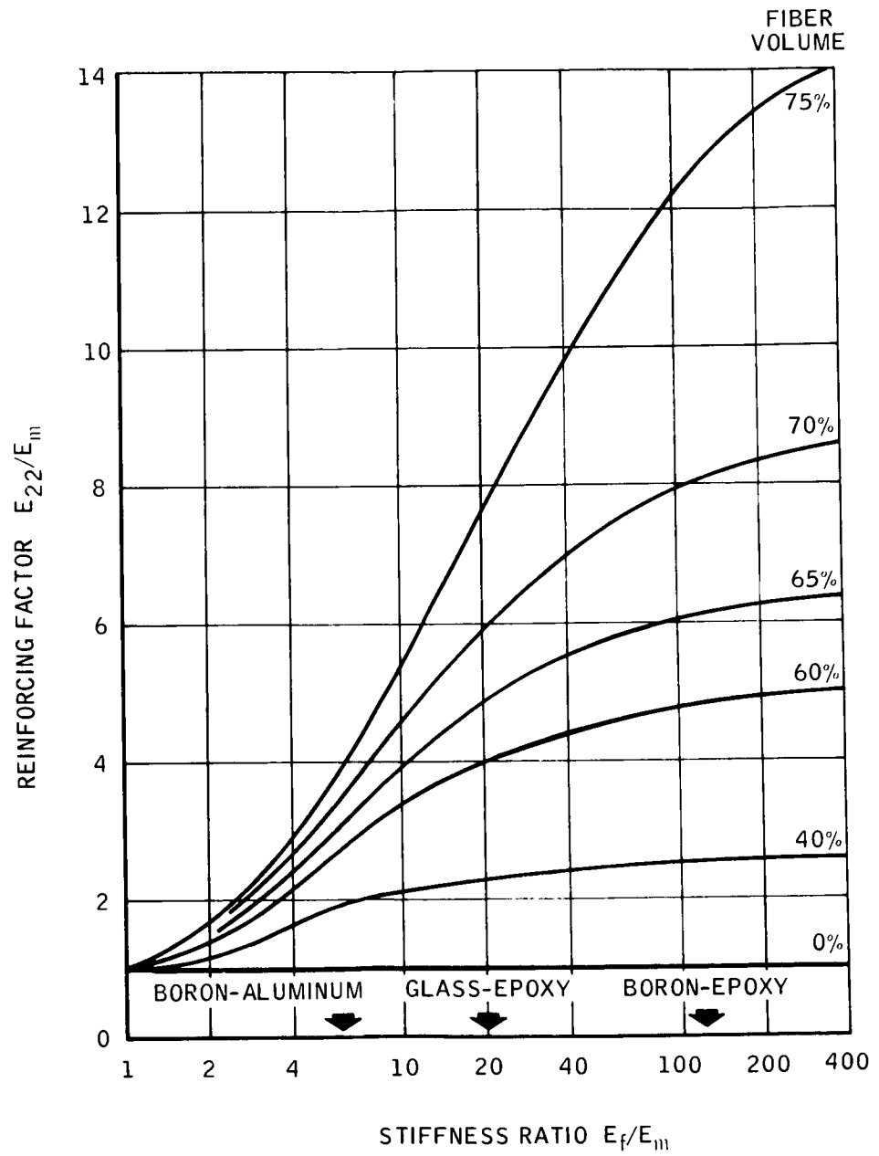
Figure 32. Composite Transverse Stiffness for Circular Fibers in a Square Array
