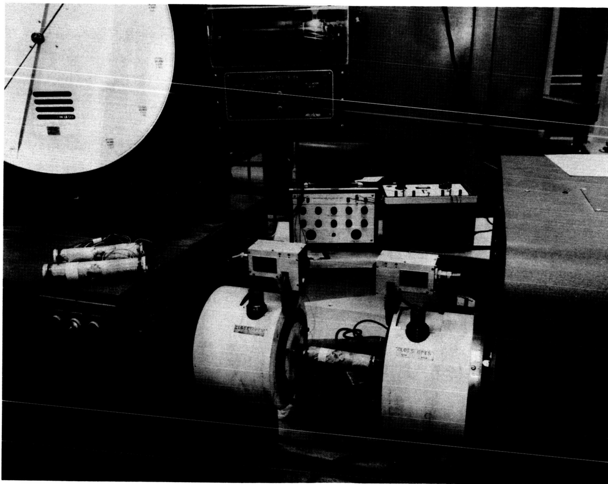
Figure 14. Torsion Test
