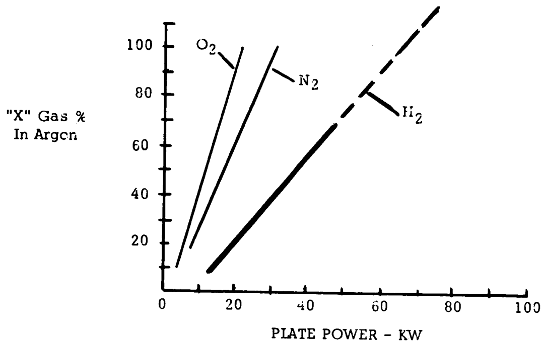
Figure 8. - Variation of gas capability with 5 MC power input to model 56 induction torch.
