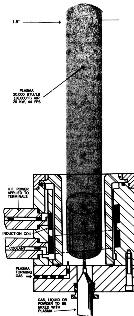
Figure 3. - Plasma torch.
