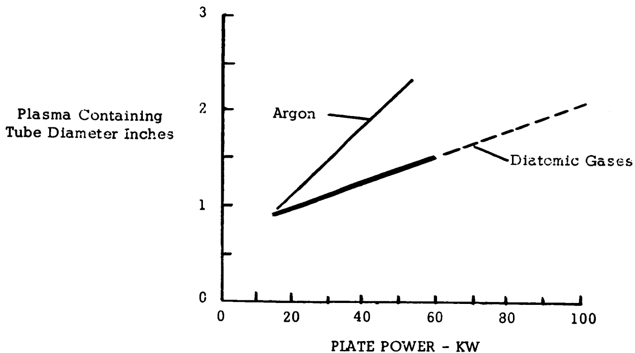
Figure 9. - Power rating various plasma tube diameter with various gases - 1 ATM.
