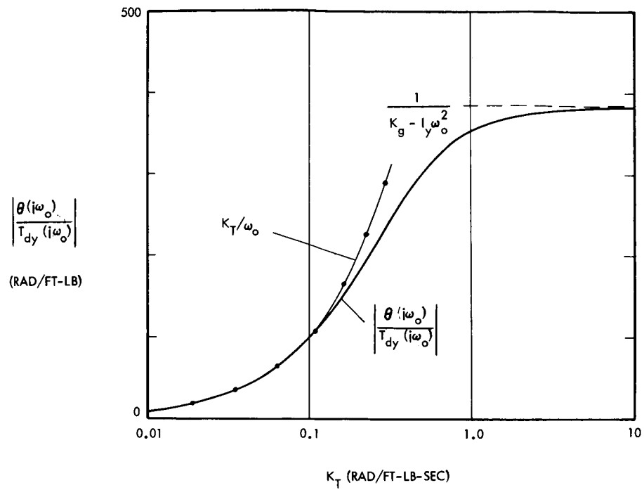
Figure 5 Effect of Tachometer Gain upon Pitch Attitude Error ( \omega_o = 0.001 rad/sec)
