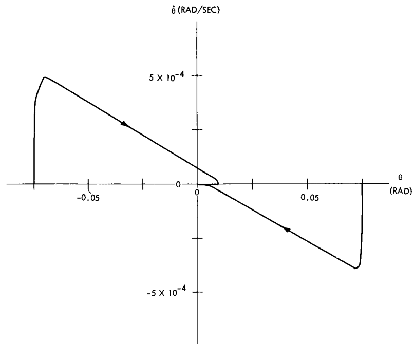
Figure 6 Pitch Transient Response
