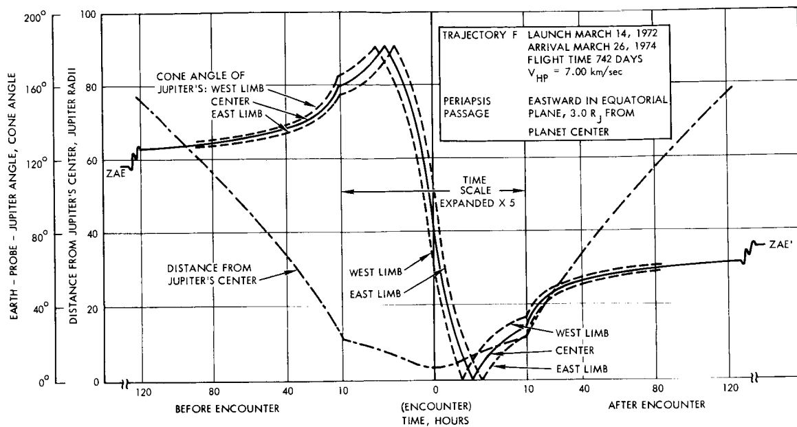
Figure 2-37. Cone Angle and Distance from Jupiter Versus Time from Encounter, R_P = 3 R_J
