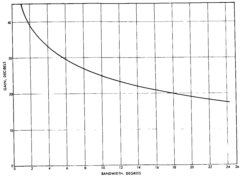
Figure 4-28. Antenna Gain Versus Beam Width
