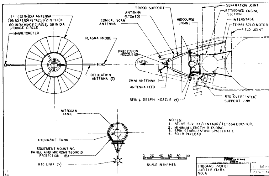
Figure 4-65. Inboard Profile — Jupiter Flyby No. 6
