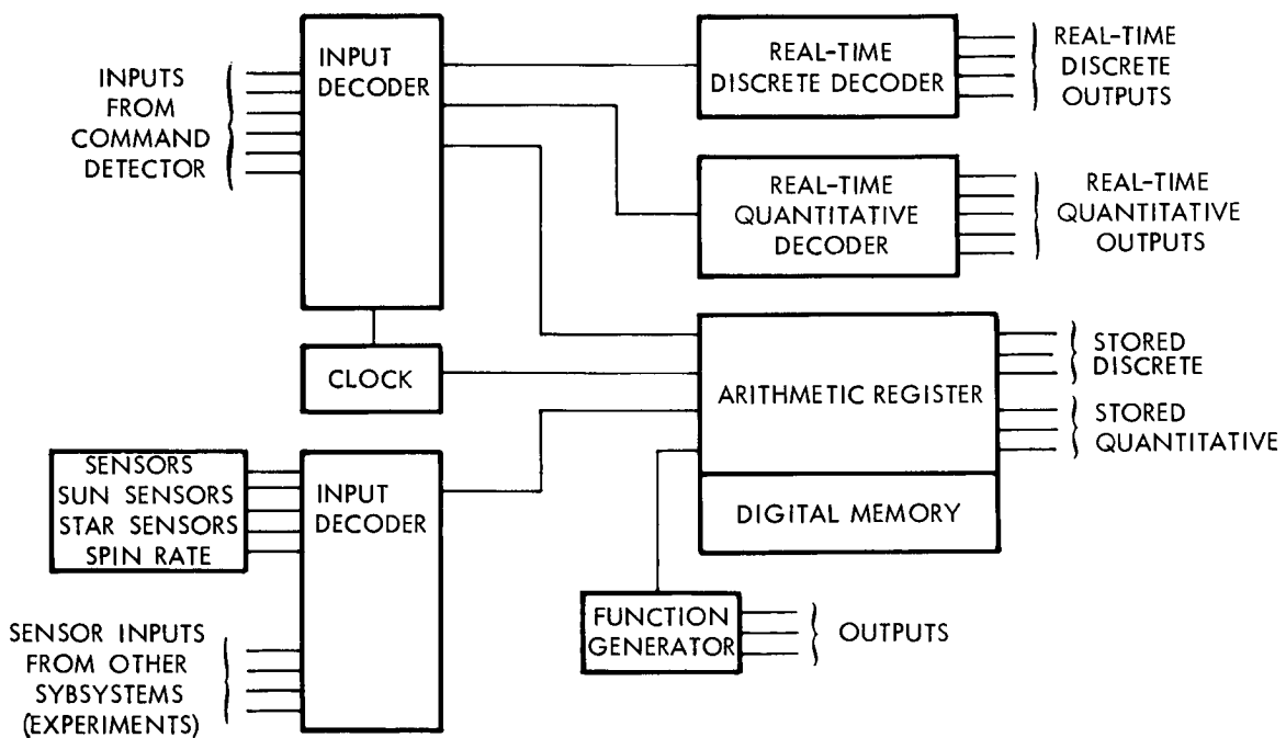
Figure 4-45. Autonomous System
