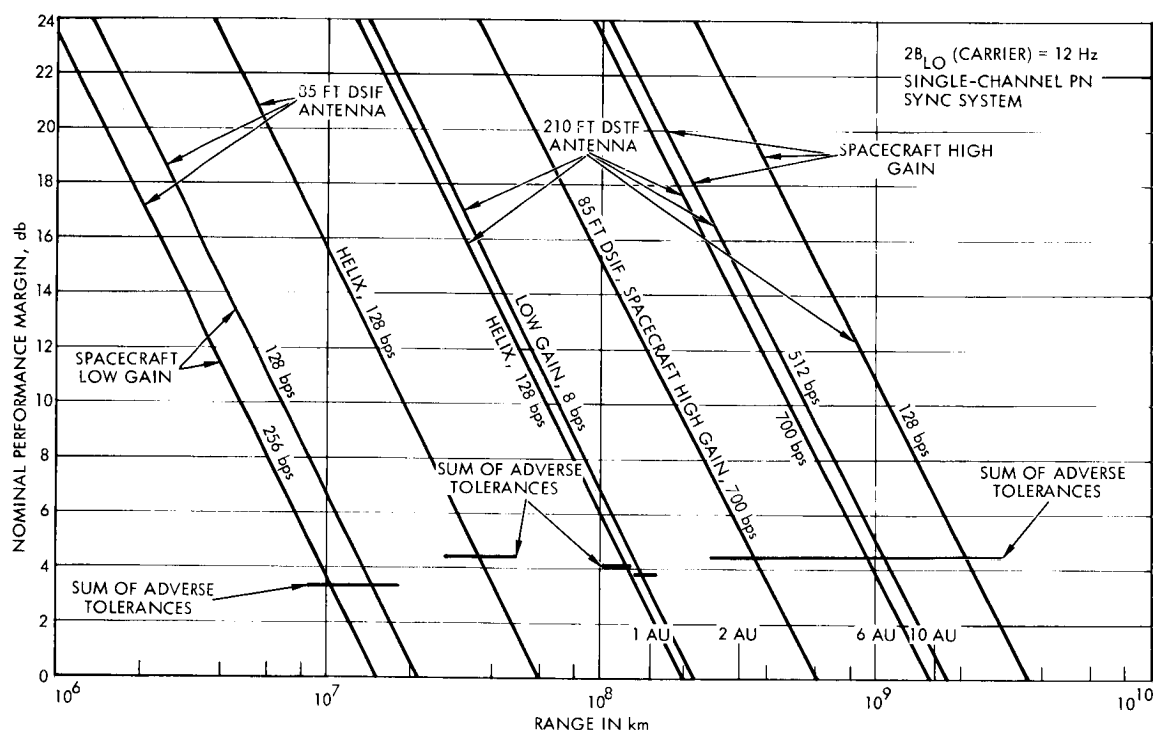
Figure 8-28. Spacecraft-to-Earth Performance Versus Range
