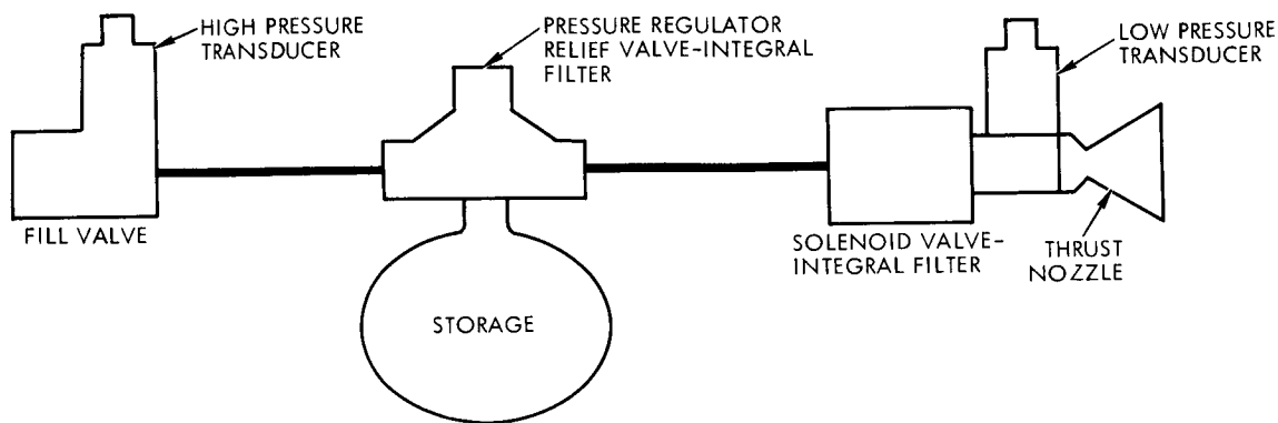
Figure 8-23. Pneumatic Assembly
