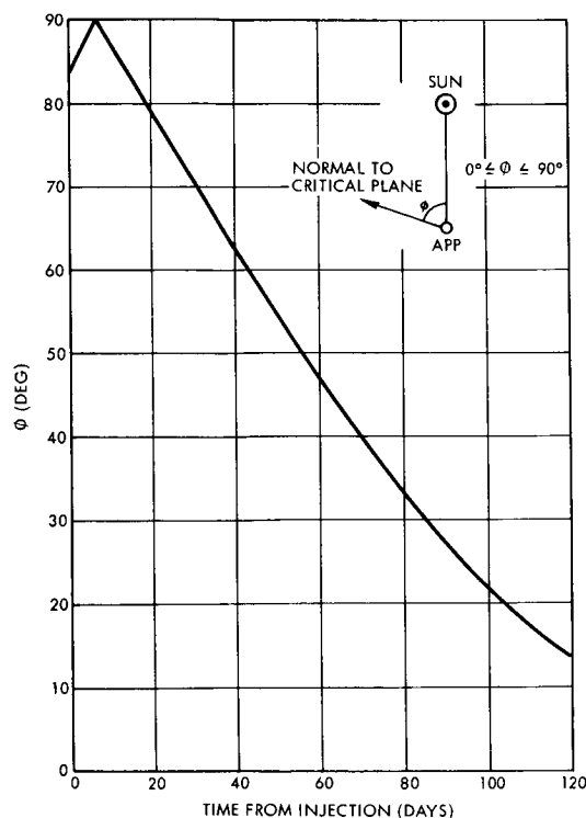
Figure 4-10. Orientation of Normal to Critical Plane
