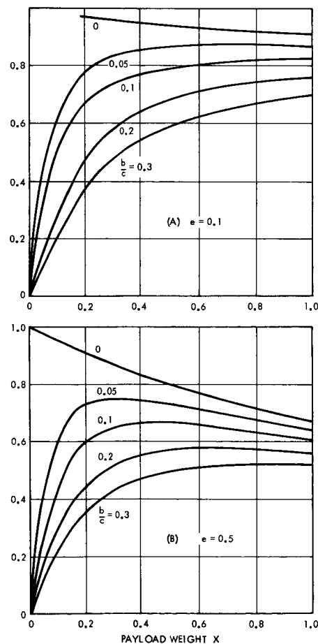
Figure 12-3. Cost-Effectiveness Index Versus Payload Weight
