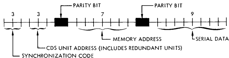
Figure 8-39. Word Formats for Special Purpose Programmer
