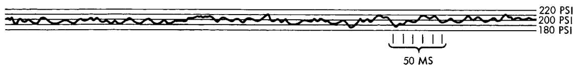
Figure 8-54. Steady State Operation
