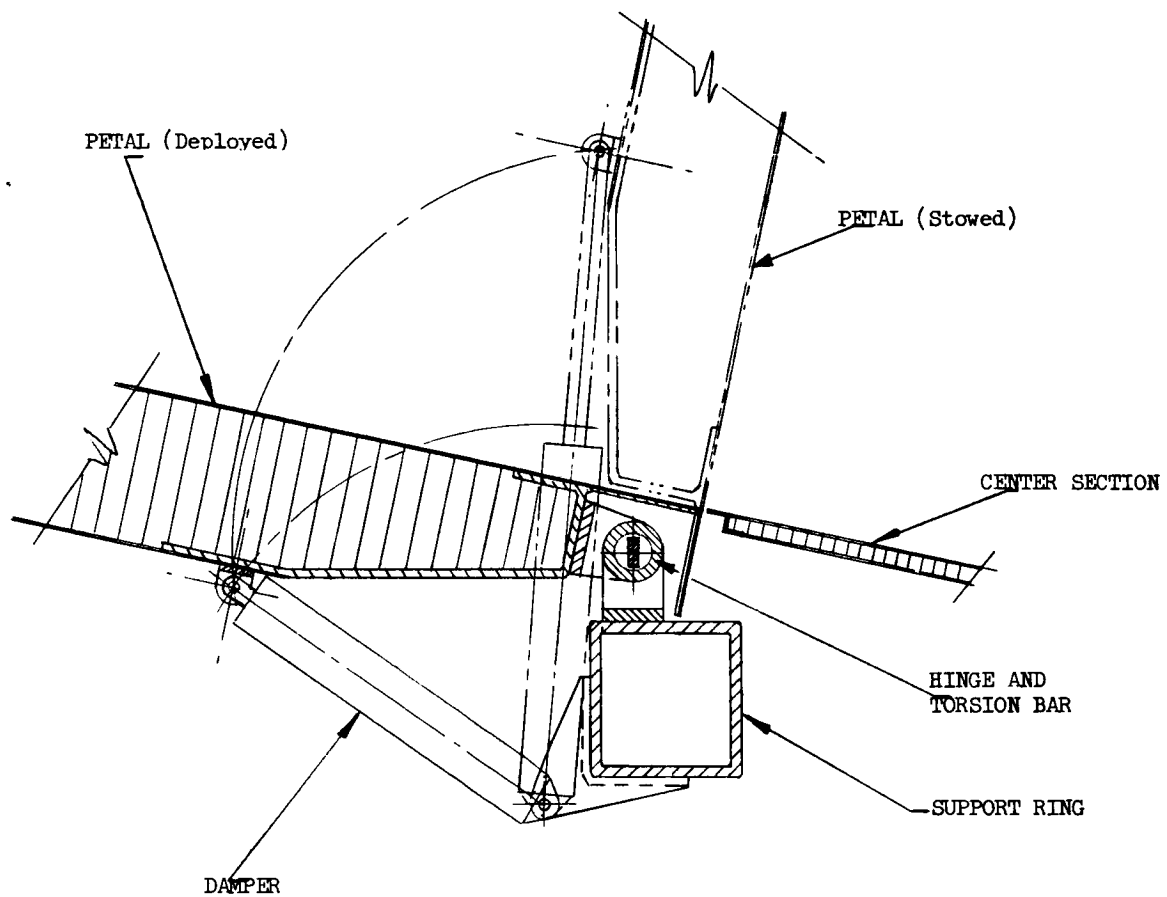
Figure 4-7. Viscous Damper
