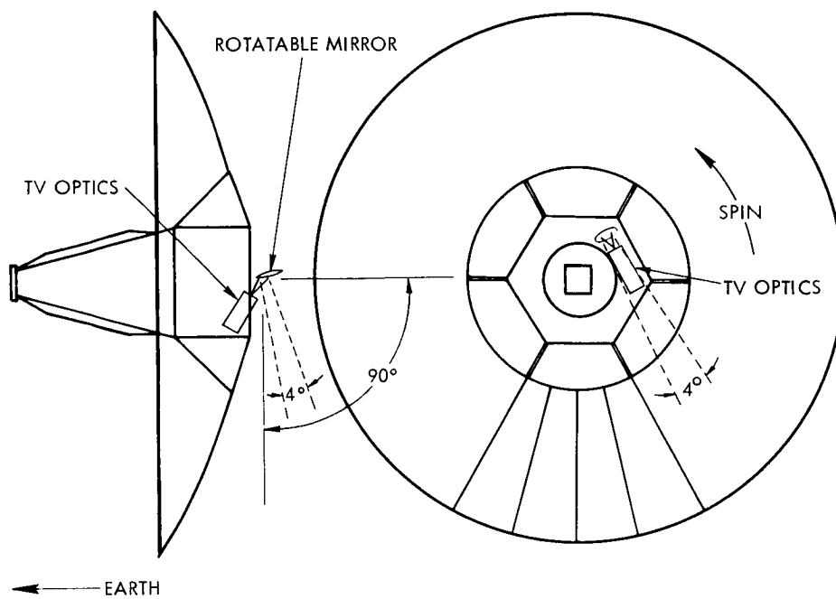
Figure 4-60. Television
