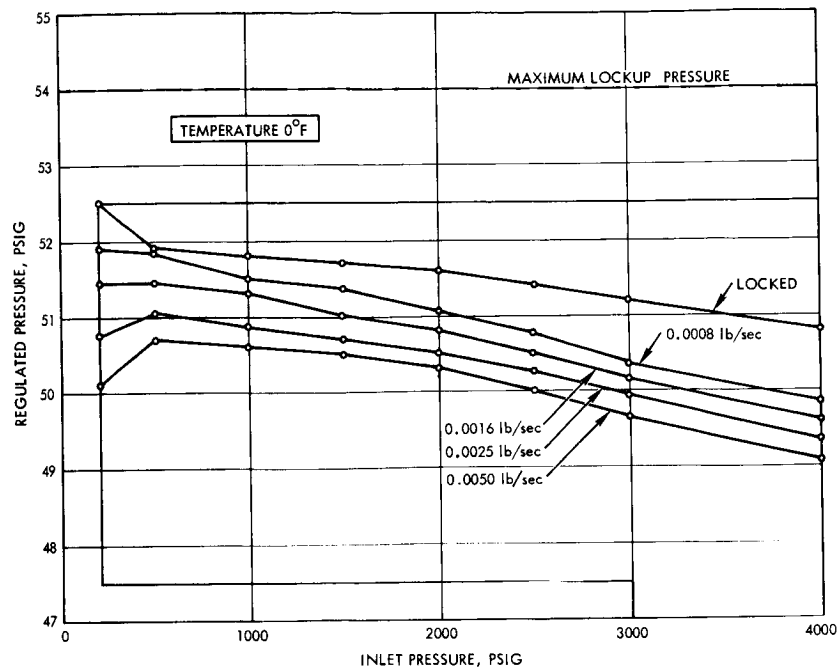
Figure 4-23. Characteristics of Pioneer Pressure Relief Valve
