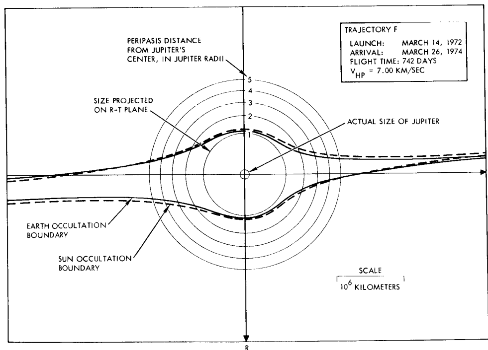
Figure 2-31. Occultation Boundaries
