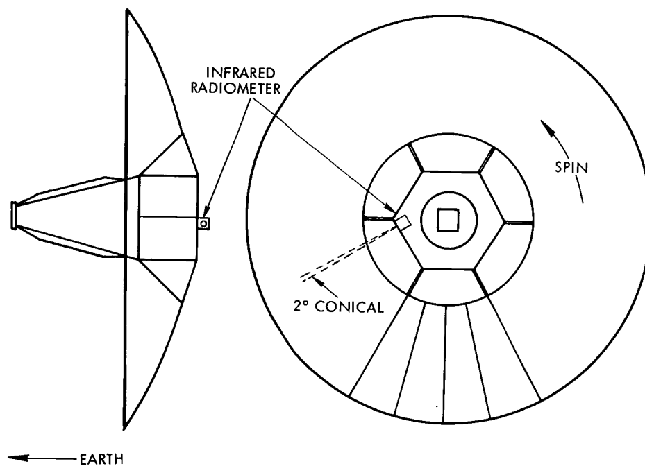
Figure 4-59. Infrared Radiometer
