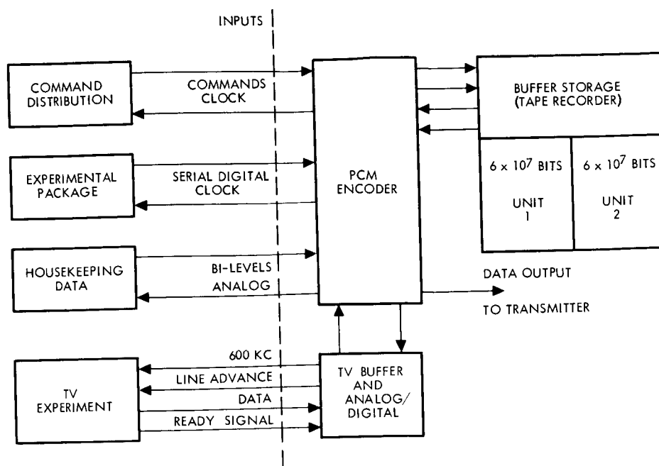
Figure 8-31. Data Handling Subsystem
