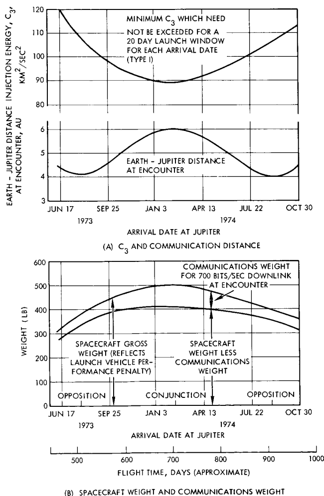
Figure 2-17. Influence of Communication Distance and C_3 Requirement on Selection of Arrival Date
