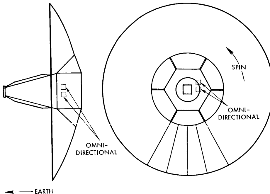
Figure 4-62. Trapped Radiation
