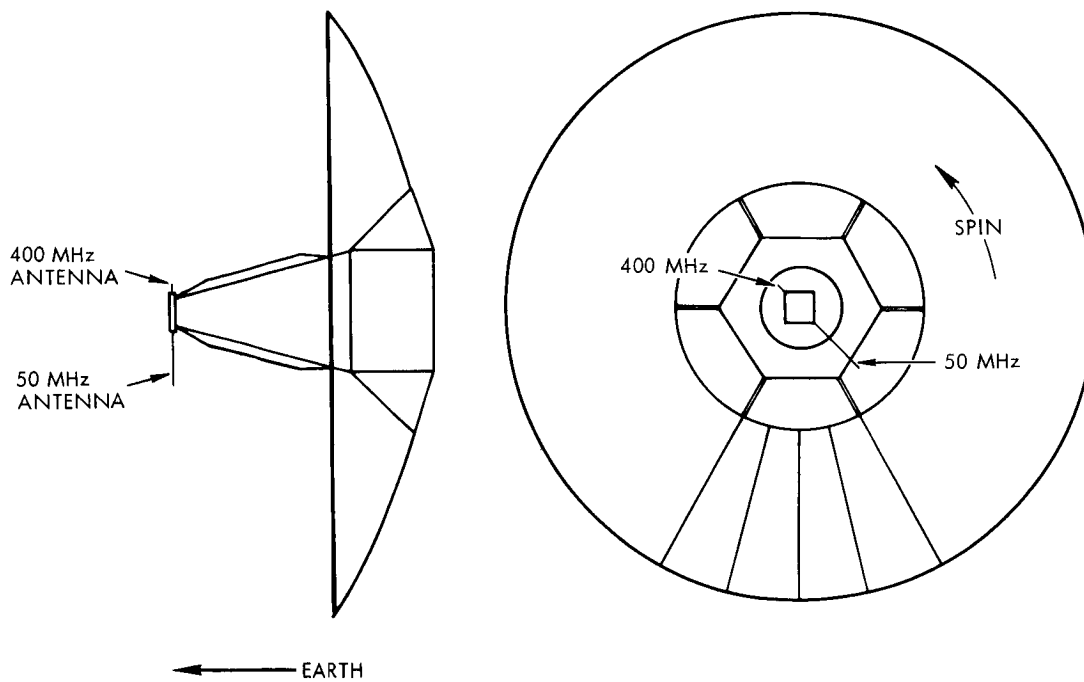
Figure 4-61. Radio Propagation
