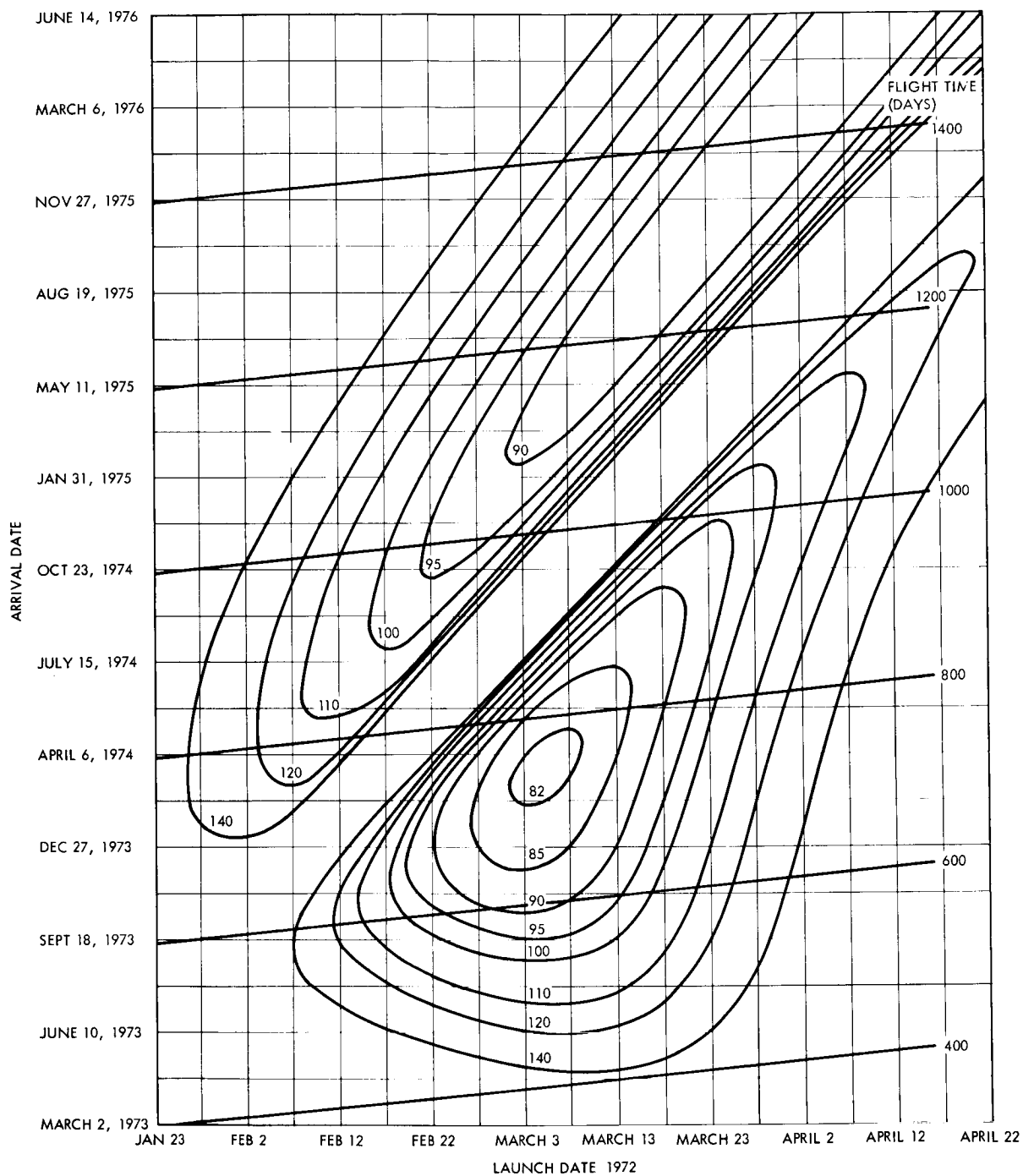
Figure 2-9. Earth-Jupiter 1972 Trajectories
