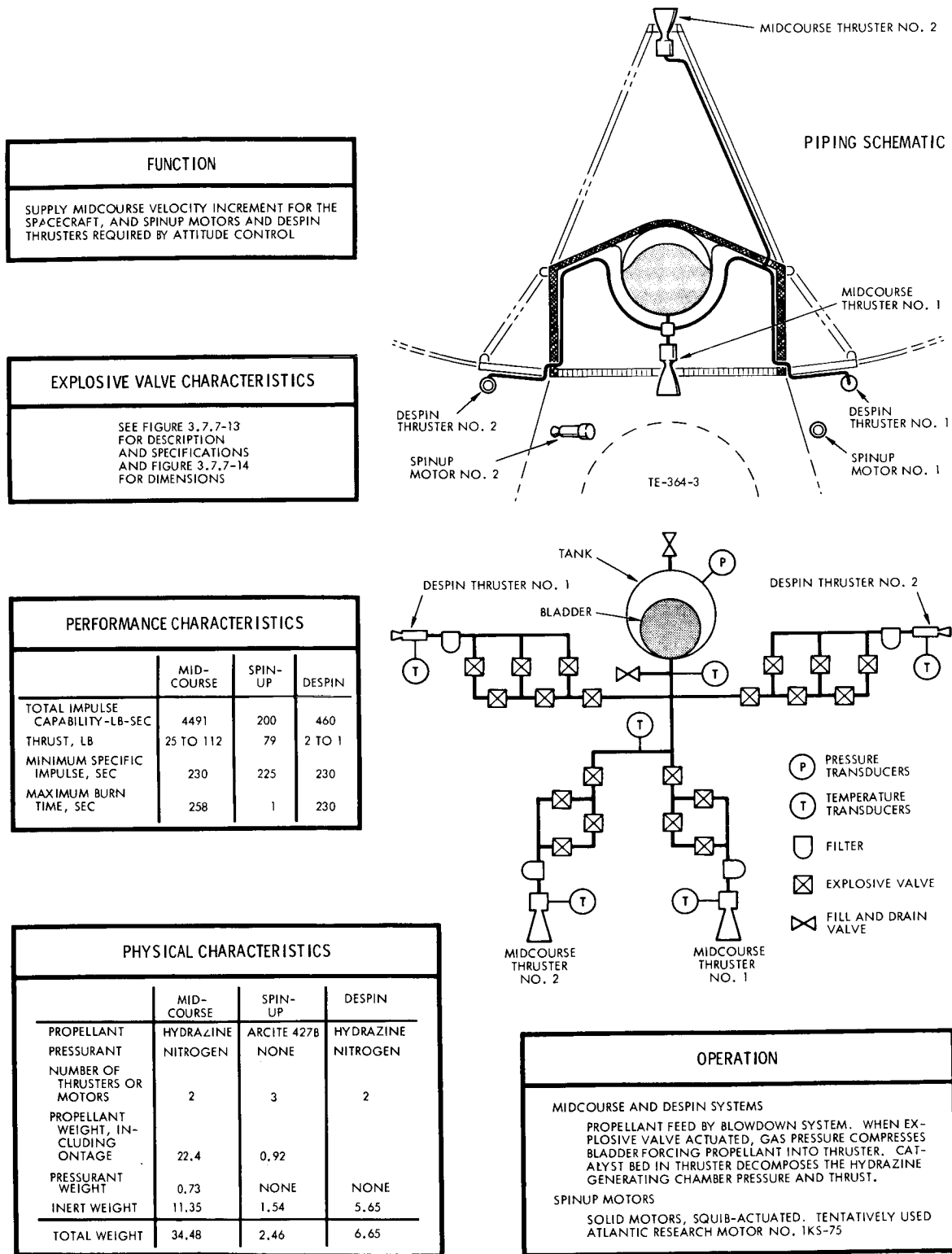
Figure 8-50. Preliminary Specification Propulsion Subsystem
