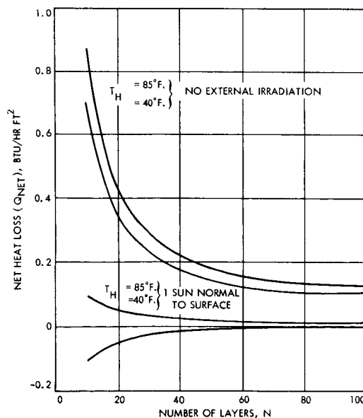
Figure 8-66. Heat Losses Through NRC-2 Insulation
