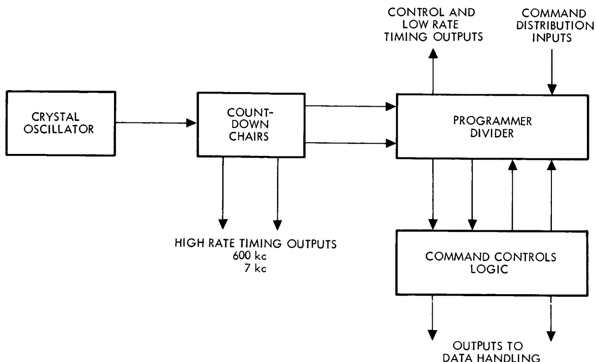
Figure 8-35. Clock and Programmer
