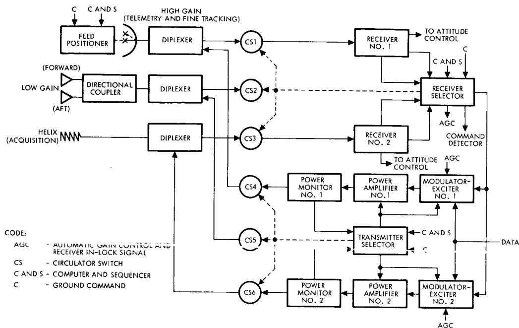
Figure 8-26. Recommended Telecommunication System for Spin-Stabilized Probe
