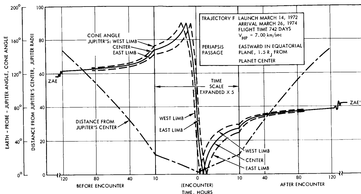
Figure 2-34. Cone Angle and Distance from Jupiter Versus Time from Encounter, R_P = 1.5 R_J
