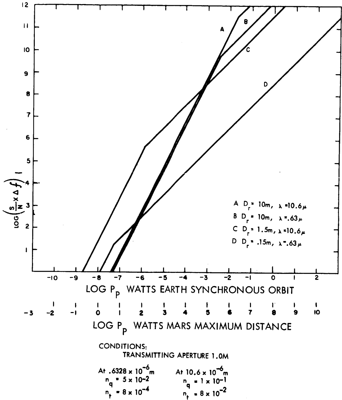
Figure 4.1-12. Direct System
