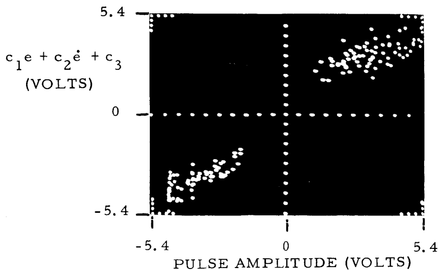
FIGURE 6 - c_1e + c_2\dot{e} + c_3 Vs PULSE AMPLITUDE, POSITIVE AND NEGATIVE PULSES OPTIMIZED SEPARATELY
