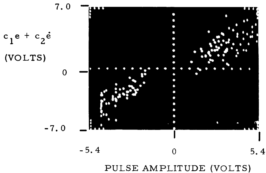
FIGURE 5 - c_1e + c_2\dot{e} Vs PULSE AMPLITUDE, POSITIVE AND NEGATIVE PULSES OPTIMIZED SEPARATELY
