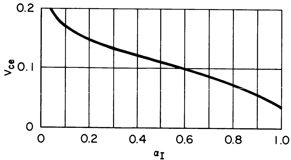
Fig. 2. V_{ce} vs a_I for \beta_N = 2 I_C/I_B = 15 kT/q = 26 \text{ mV}
