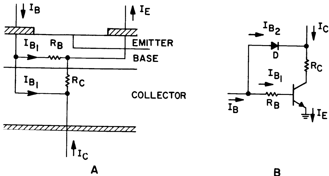
Fig. 3. Internal resistances
