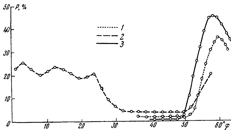
Fig. 4. Dependence of the frequency of occurrence of scintillations on the geographic latitude
