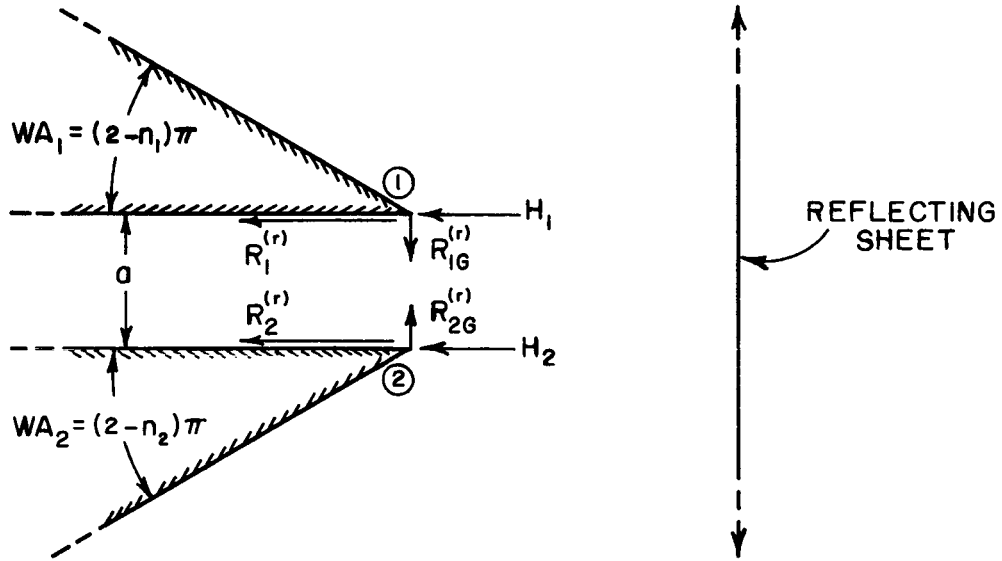
Fig. 19. Effect of the total reflected wave incident on the guide aperture.
