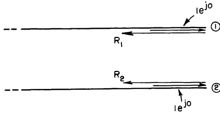
Fig. 11. Self-reflection coefficient ray diagram.
