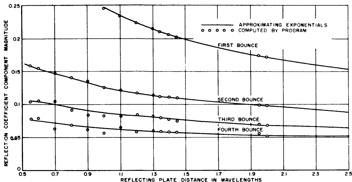
Fig. 31. Bounce wave reflection coefficient magnitudes.
