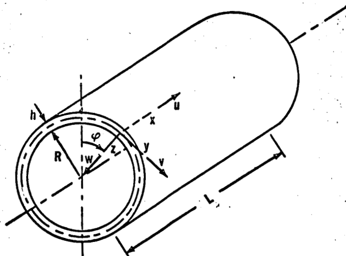
FIG. 1b. GEOMETRY OF CYLINDER.
