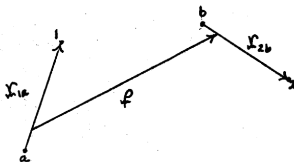
c. The " \phi " System for Two One-Electron Atoms
