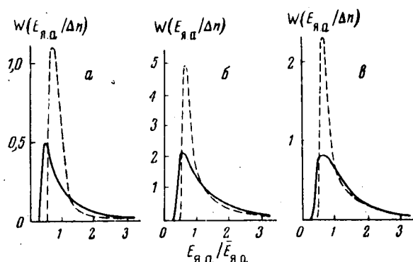
Fig. 2. - Distribution by energies of n.a. particles contributing to ionization impulses in the given interval of values — n \rightarrow n + \Delta n : a —: n = 10^2 \rightarrow 1.5 \cdot 10^2 ; b —: n = 10^3 \rightarrow 1.5 \cdot 10^3 ; c —: n = 10^4 \rightarrow 1.5 \cdot 10^4 . The solid line corresponds to nucleons, the dashed line — to a \pi -meson. The probability is plotted in ordinates in arbitrary units. The functions are normalized by areas.
