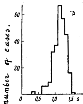
Fig. 5. - Distribution by s of showers with a number of particles N \geq 10^5 .
