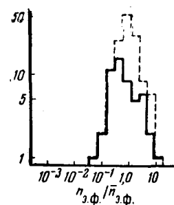
Fig. 1. — Experimental distribution of energy fluxes of the e-ph component in showers with the number of particles N = 10^5 \rightarrow 3 \cdot 10^5 at various distances from the axis:
