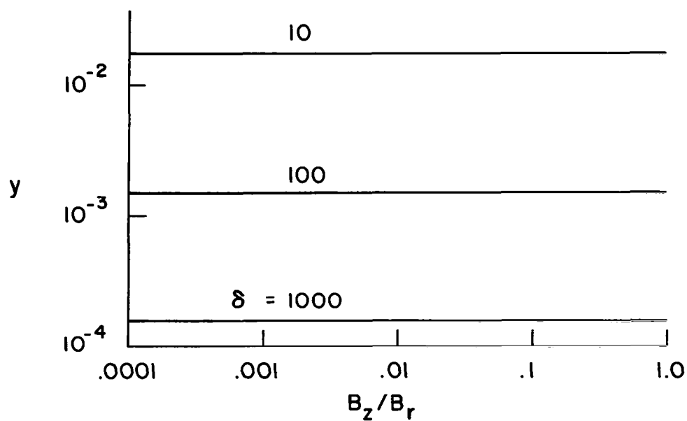
Figure 10. Critical magnetic field versus magnetic field ratio, \eta_0 = 0.01
