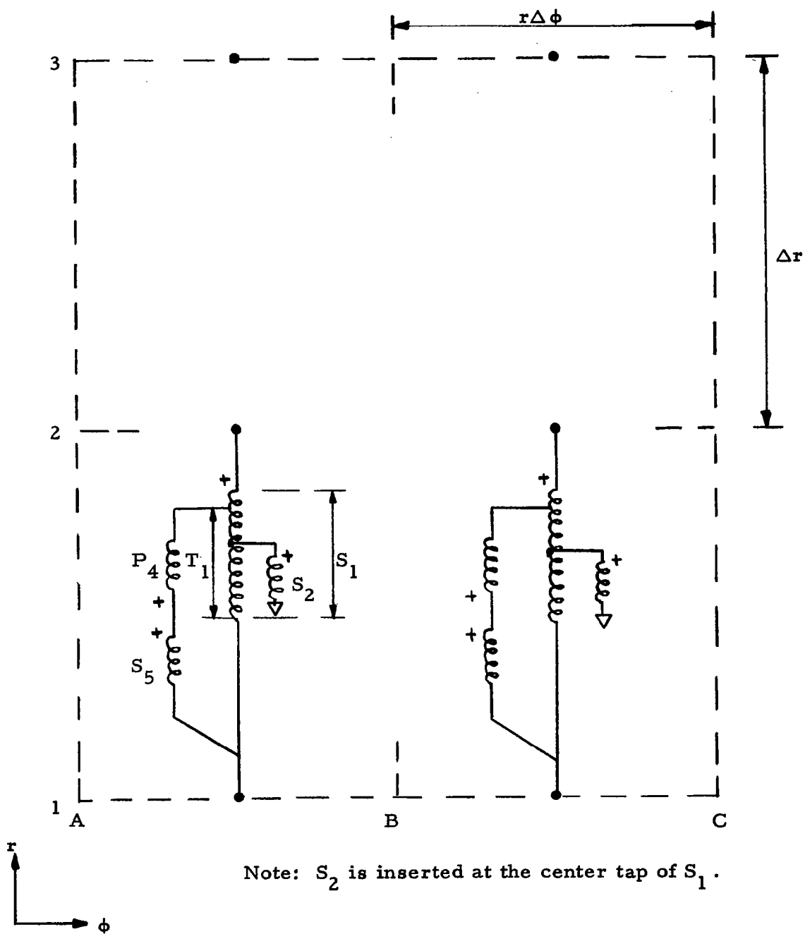
Figure 3-b. \theta_r Circuit for an Arbitrary Section of Flat Circular Plate
