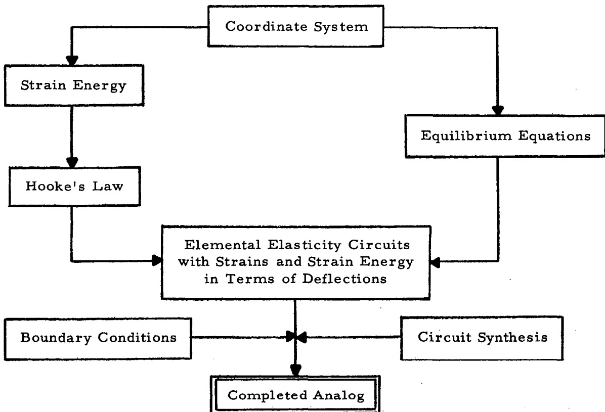
Figure 1. Strain Energy-Compatibility Approach for a Passive Electrical Analog of an Elastic Structural System
