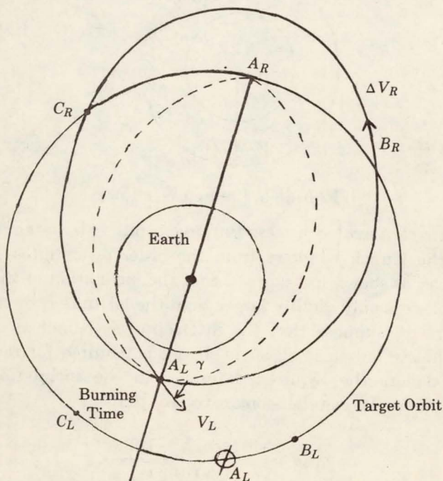
FIGURE 5. Transfer Orbits
