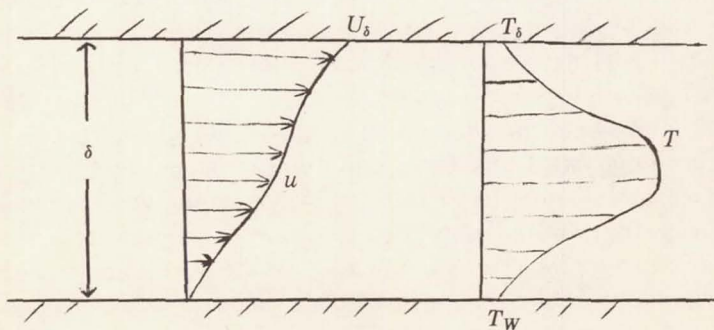
FIGURE 32. Couette Flow
