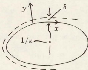
FIGURE 30. Boundary Layer over Curved Body.
