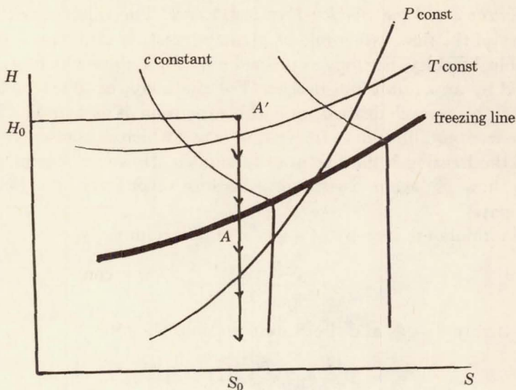
FIGURE 26. Mollier Diagram
