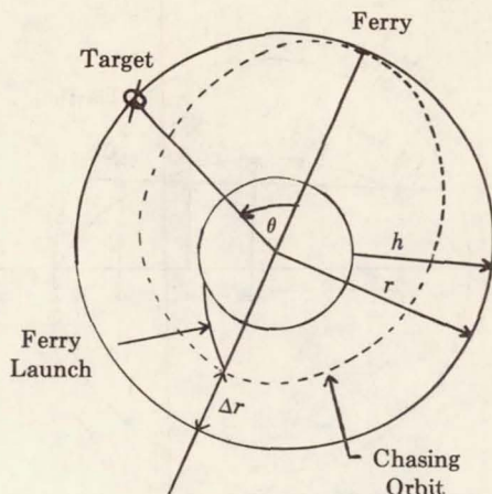
FIGURE 8. Hohmann-type Transfer
