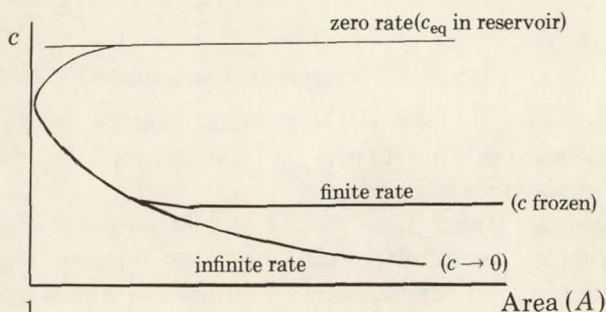
FIGURE 21. Atom Concentration against Area Ratio
