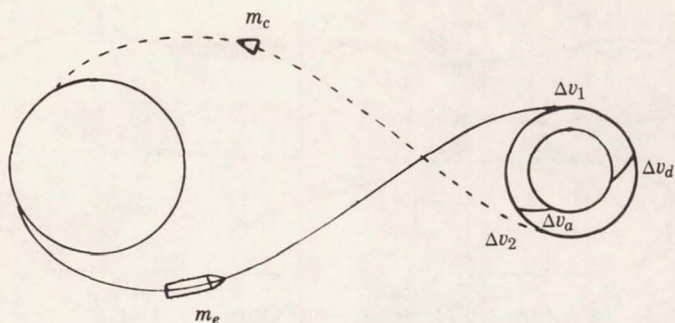
FIGURE 19. Lunar Rendezvous Orbits
