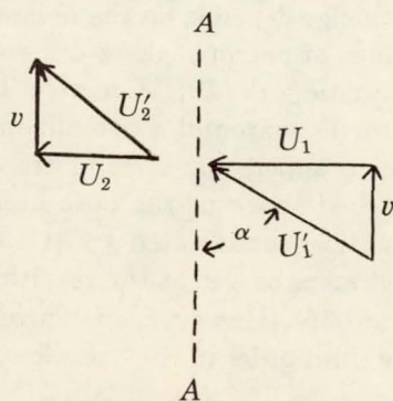
FIGURE 23. Region near Oblique Shock Wave.
