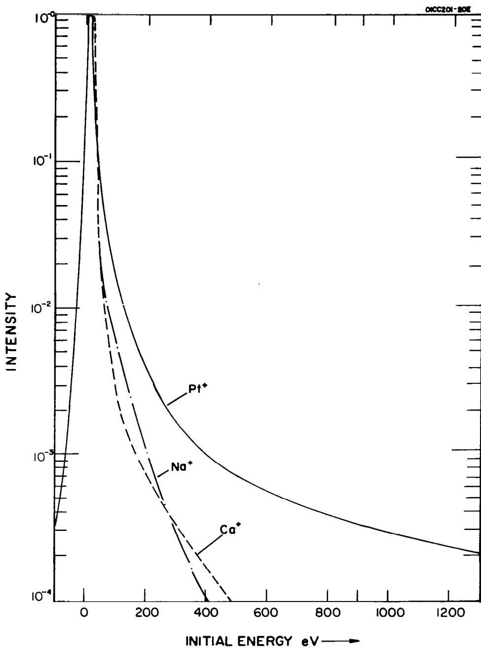
Figure 6. Energy distribution of \text{Pt}^+ , \text{Ca}^+ , and \text{Na}^+ sputtered from a platinum ingot with 12 KeV \text{Ar}^+ . (All intensities normalized to "one".)
