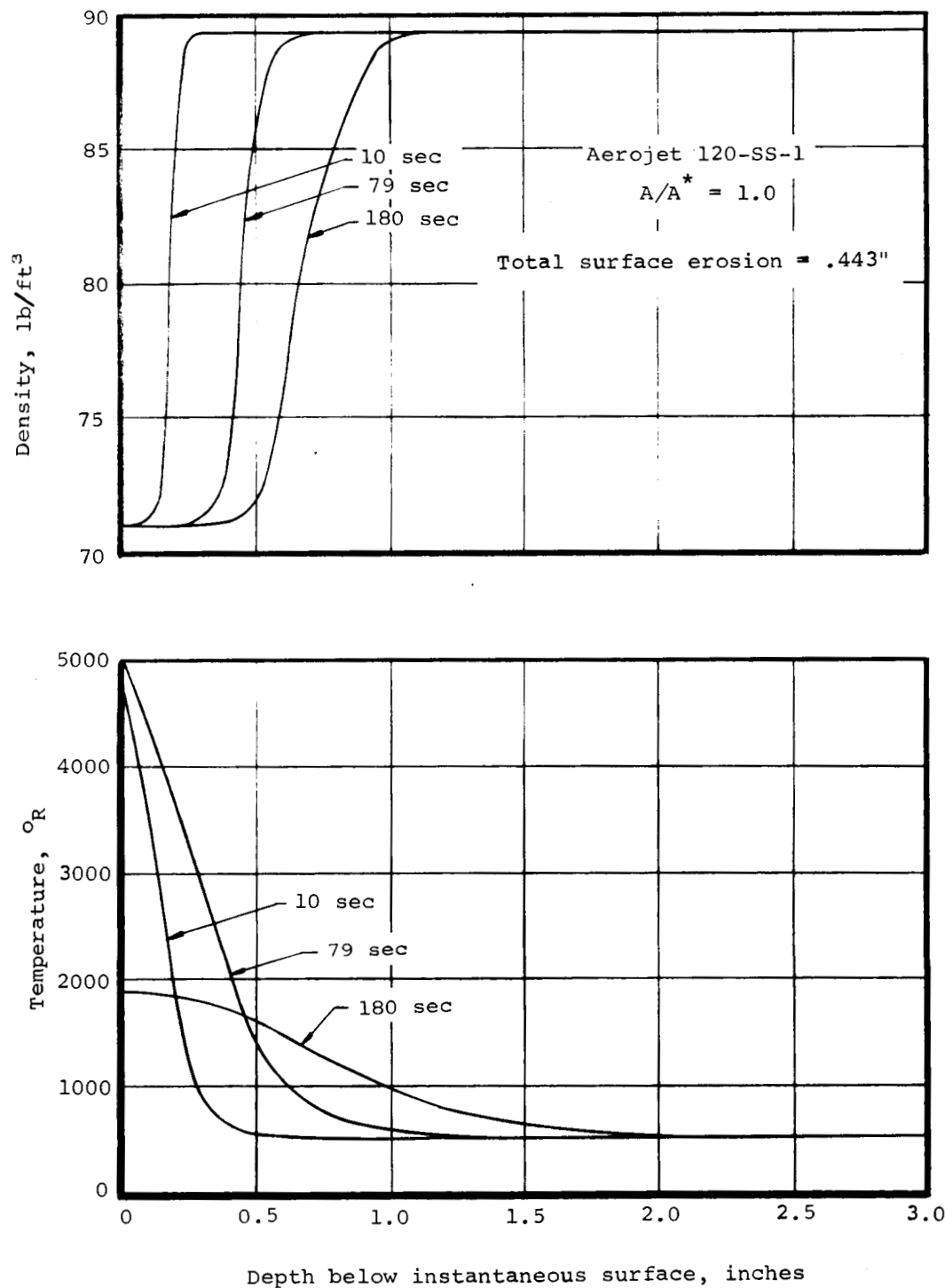
Figure 36.- Predicted temperature and density distributions for the throat of the 120-SS-1 nozzle for equal predicted and measured average surface erosion depth.
