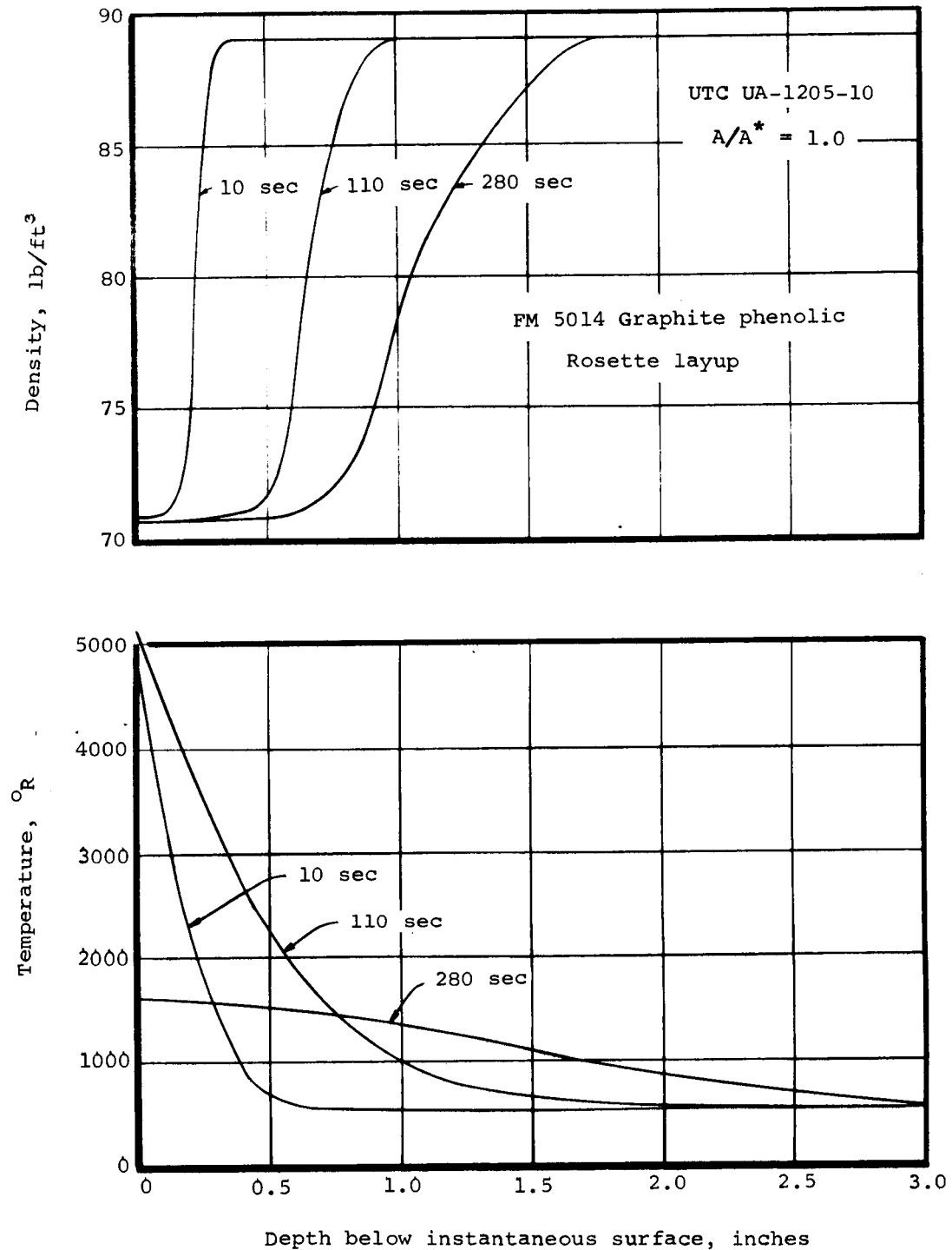
Figure 15- Predicted temperature and density distributions for the throat of the UA-1205-10 nozzle.
