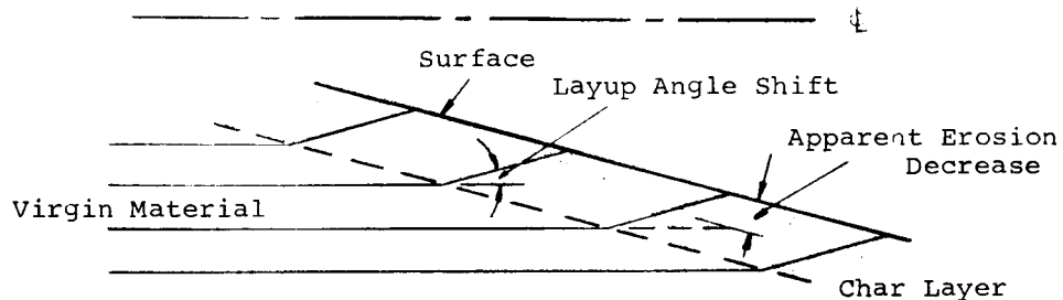
Figure 16.- Schematic of char layup angle warp phenomenon.
