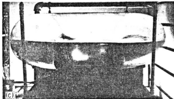
FIGURE 5.24.—Mode shapes for first three natural modes of liquid in a horizontal toroid. (a) First mode; (b) second mode; (c) third mode.
