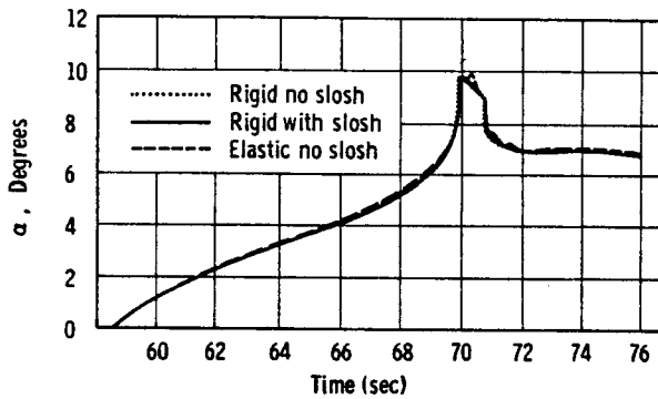
FIGURE 7.33.—Angle of attack.
