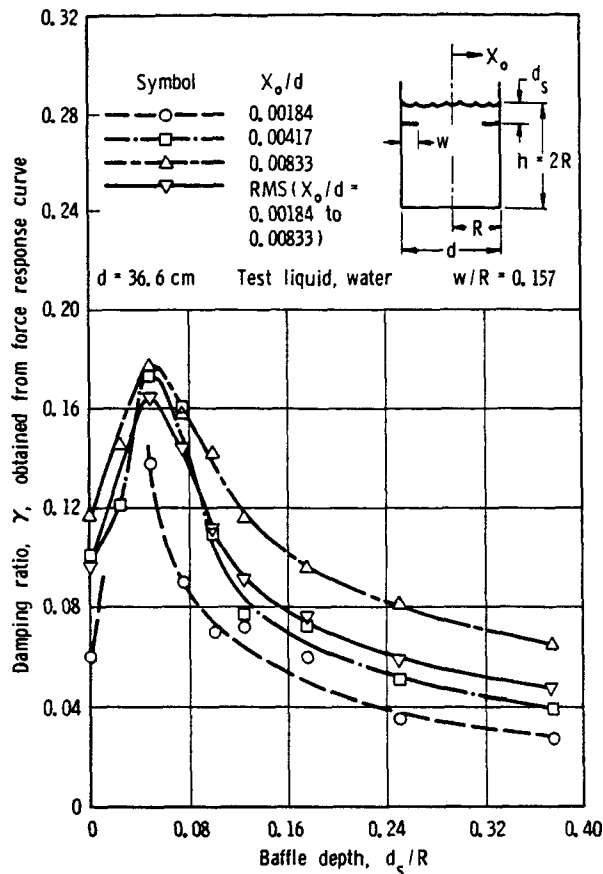
FIGURE 4.31.—Effect of excitation amplitude on damping effectiveness of a solid flat ring baffle as a function of baffle depth (ref. 4.38).
