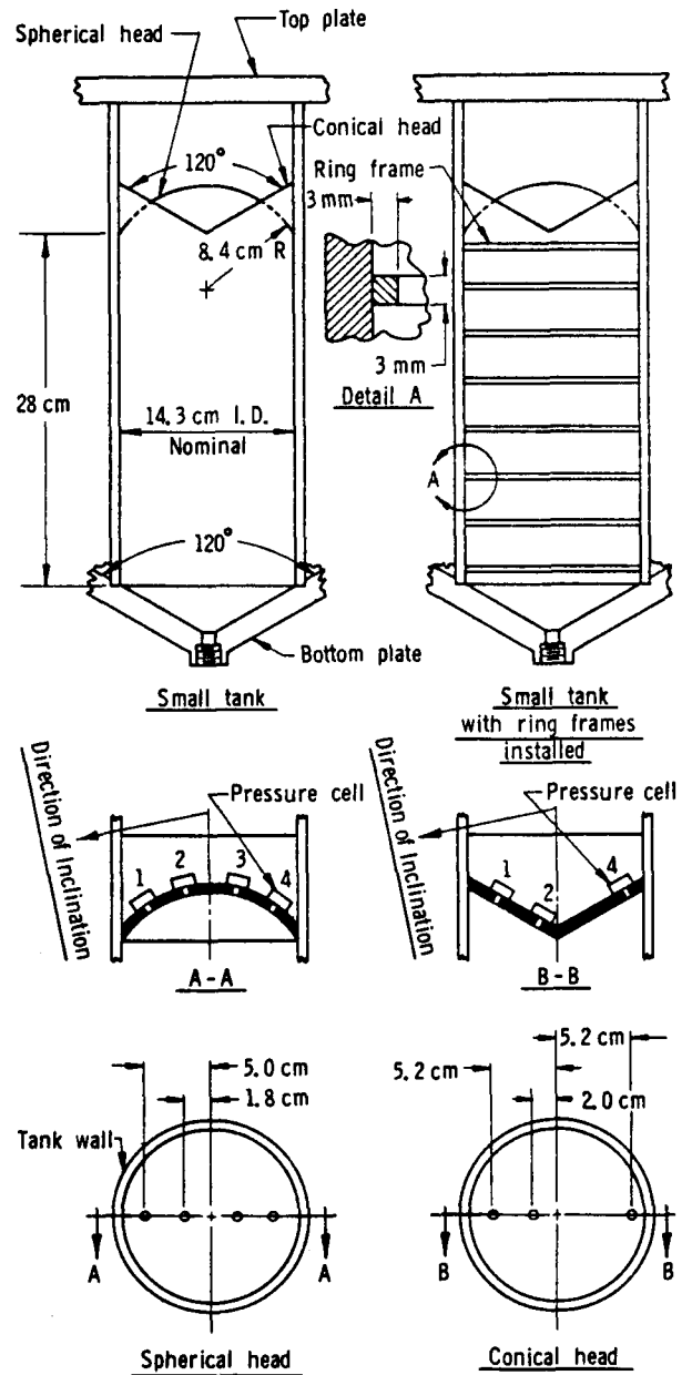
FIGURE 10.5.—Model tank geometries (ref. 10.4).
