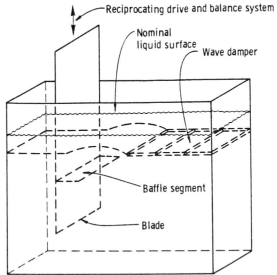
FIGURE 5.33.—Two-dimensional tank.
