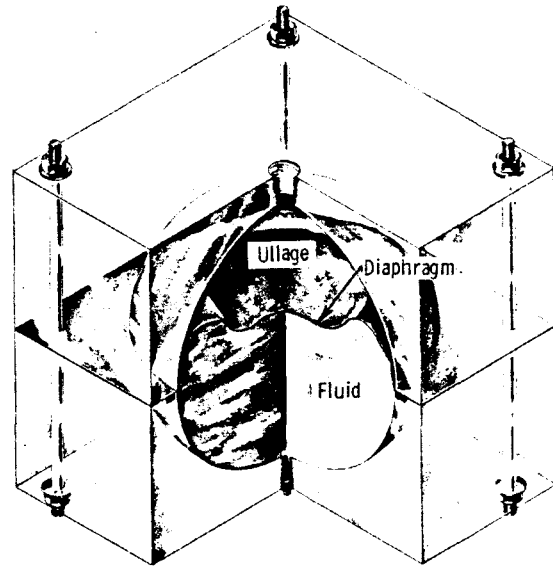
FIGURE 5.17.—Model tank constructed from Lucite blocks having internally formed tank geometry.
