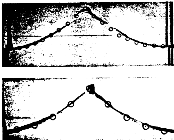
FIGURE 3.5.—Large amplitude stationary wave showing agreement with Penney and Price theory (ref. 3.11).
