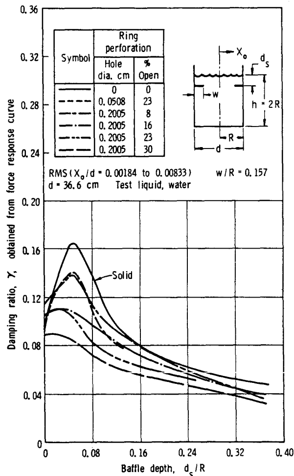
FIGURE 4.32.—Effect of percent perforation on damping effectiveness as a function of baffle depth (ref. 4.11).
