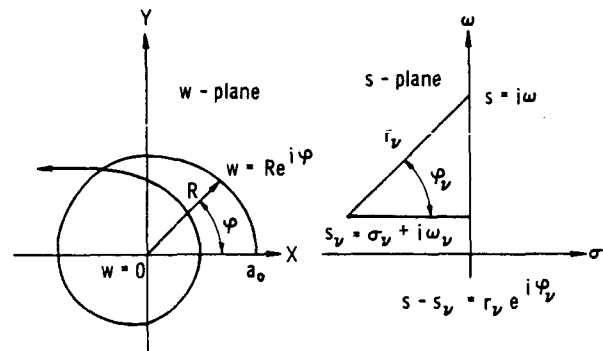
FIGURE 7.6.—Locus-curve method.
