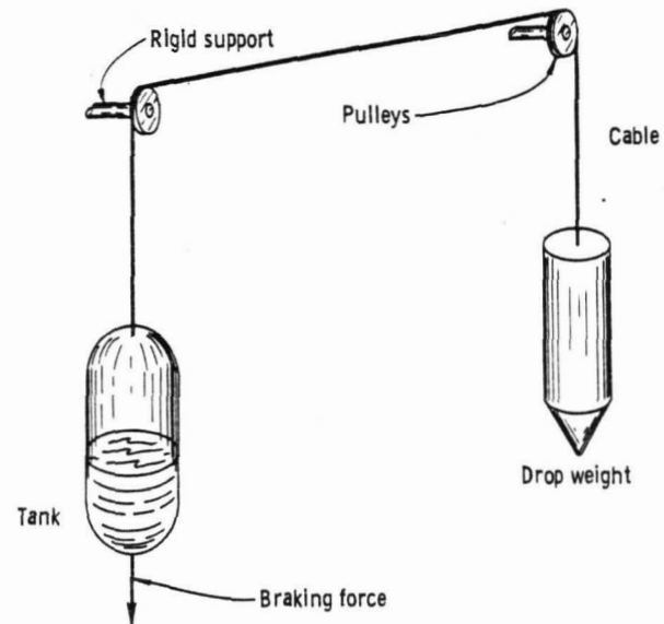
FIGURE 5.29.—Schematic of dome-impact slosh apparatus.
