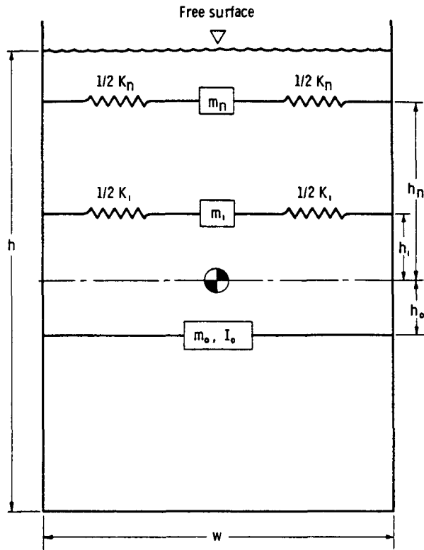
FIGURE 6.15.—Complex mechanical models for rectangular tanks.
