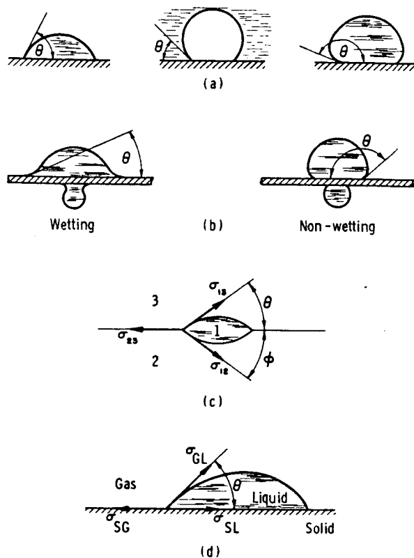
FIGURE 11.8.—Contact angles.
