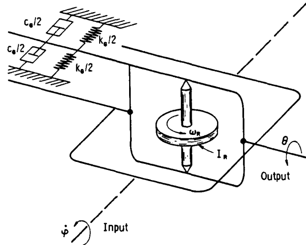
FIGURE 7.4.—Schematic of rate gyroscope mounting.
