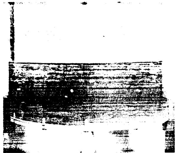
FIGURE 10.16.—Vortex formed during steady gravity draining from a cylindrical tank (ref. 10.11).
