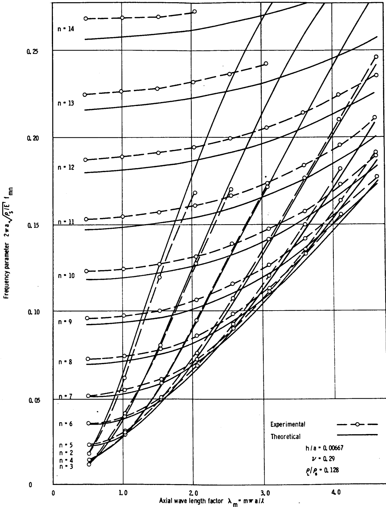
FIGURE 9.17.—Theoretical and experimental natural frequencies of liquid-filled cylinder in breathing vibration (ref. 9.9).
