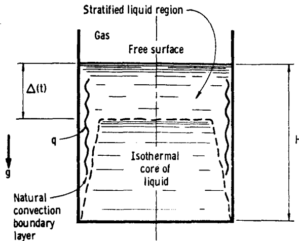
FIGURE 11.45.—Liquid stratification.
