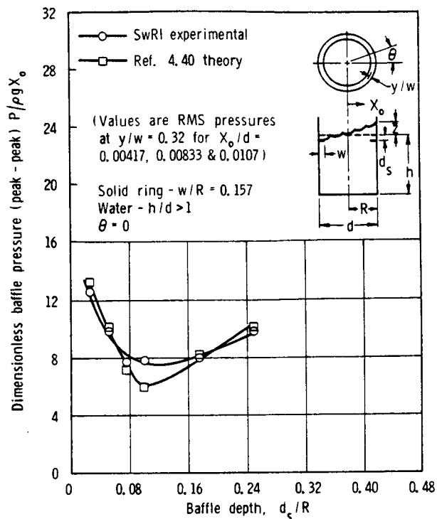
FIGURE 4.42.—Comparison of theoretical and experimental pressures on a solid-ring baffle (ref. 4.41).
