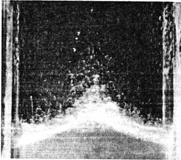
FIGURE 8.2.—Second-mode surface wave maintained by spray (ref. 8.18).
