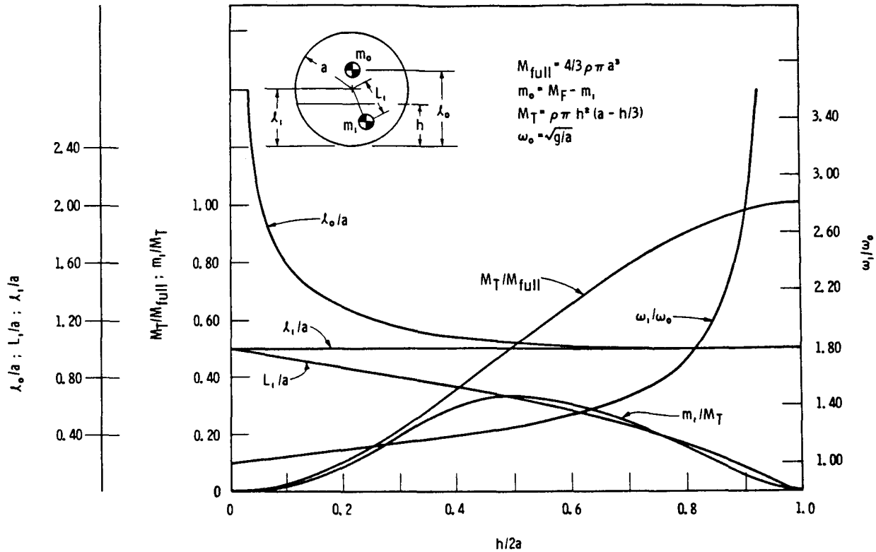
FIGURE 6.7.—Simple-pendulum mechanical model for spherical tanks (ref. 6.6).
