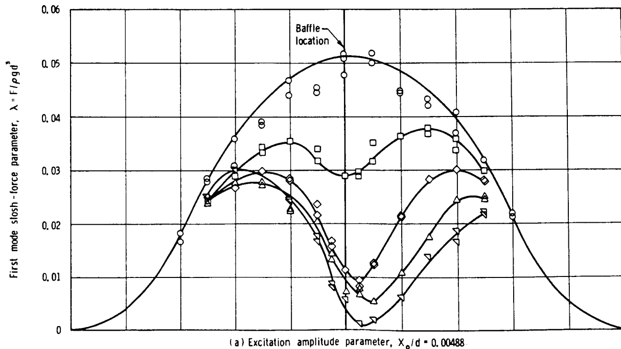
FIGURE 4.52.—Variation of first-mode slosh-force parameter with liquid depth ratio for rigid single-ring baffles in a spherical tank (ref. 4.42).
