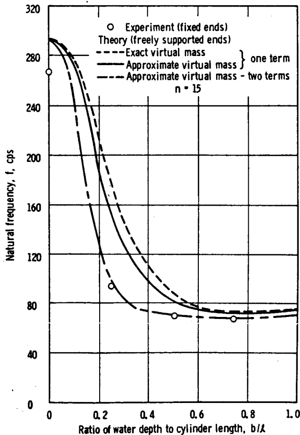
FIGURE 9.23a.—Theoretical and experimental variation of natural frequency of a pressurized cylinder with water depth (ref. 9.18). p_0 = 3.45 \times 10^4 dyne/cm 2 .
