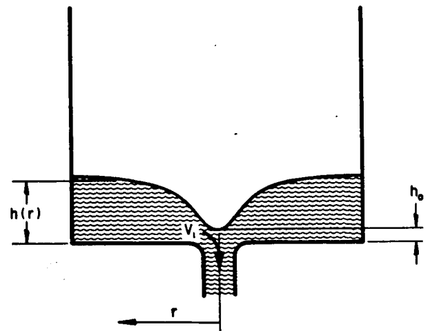
FIGURE 11.41.—Simple model for estimate of drain choking.
