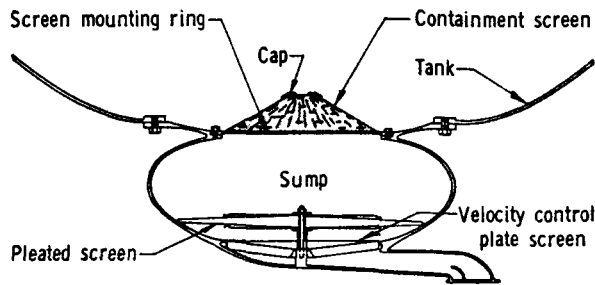
FIGURE 11.38.—Agena containment sump.
