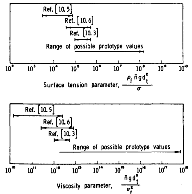
FIGURE 10.13.—Approximate ranges of viscosity and surface tension parameters.
