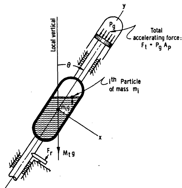
FIGURE 10.3.—Schematic of liquid impact test facility (ref. 10.4).
