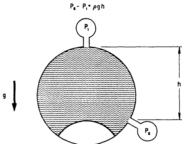
FIGURE 11.29.—Supporting pressure.
