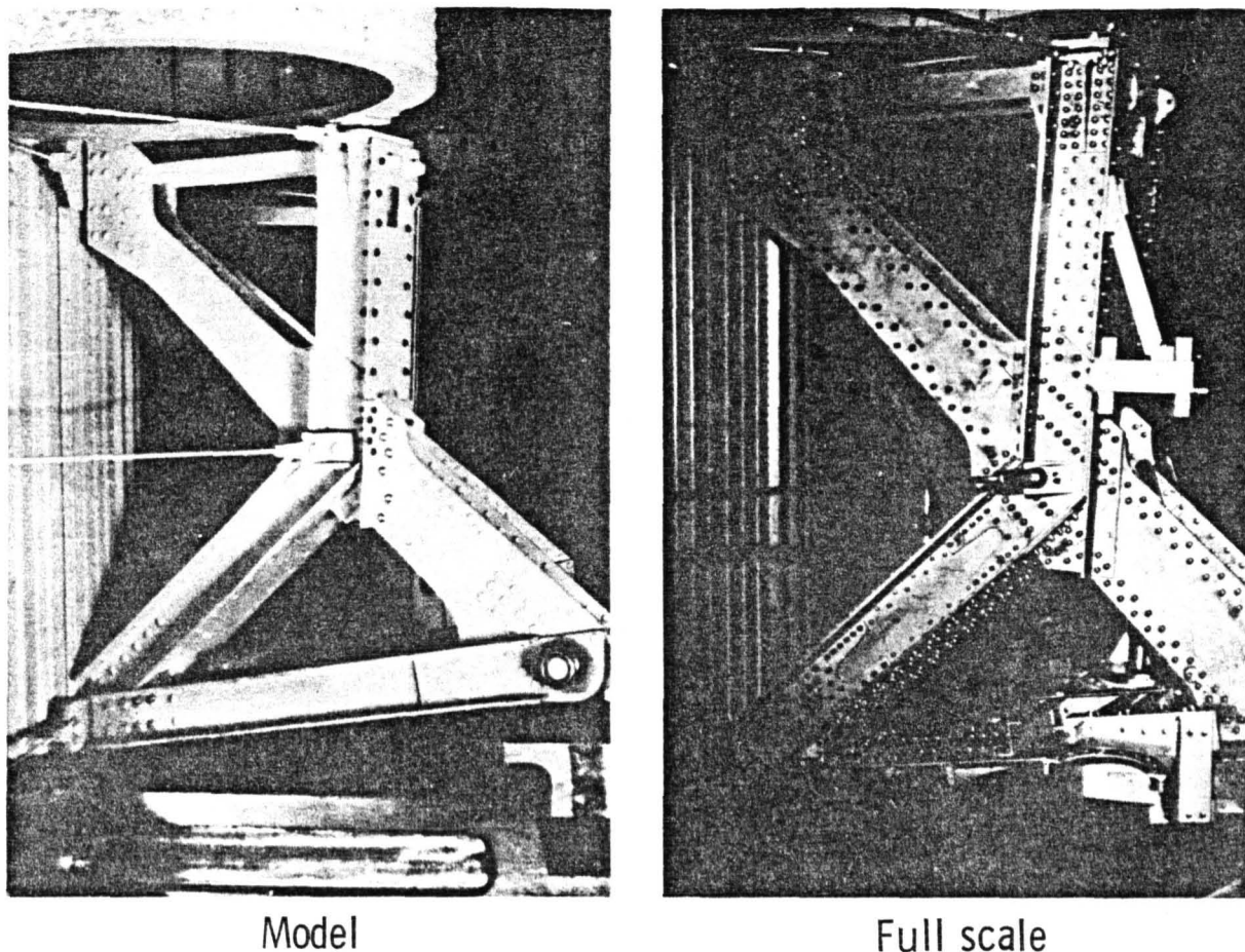
FIGURE 5.40.—Saturn SA-1 structural details.
