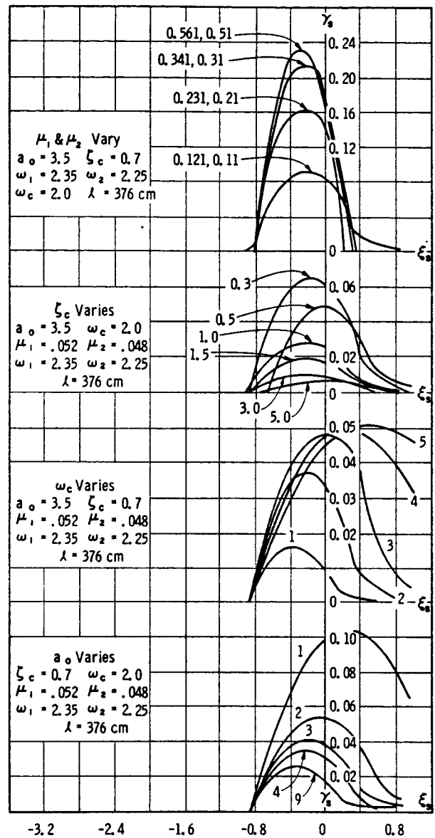
FIGURE 7.24.—Stability boundaries for sloshing in quarter-tank arrangement.
