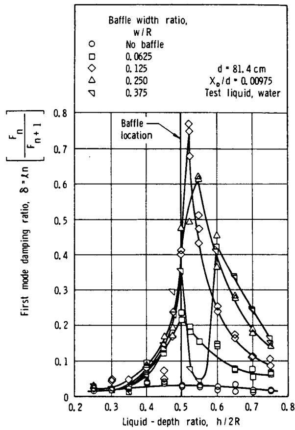
FIGURE 4.54.—Variation of first-mode damping ratio with liquid depth ratio for rigid single-ring baffles in a spherical tank (ref. 4.42).
