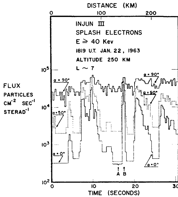
Fig. 2 Injun III > 40 keV electron precipitation fluxes
