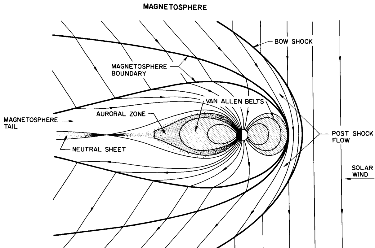
Fig. 1 Magnetosphere
