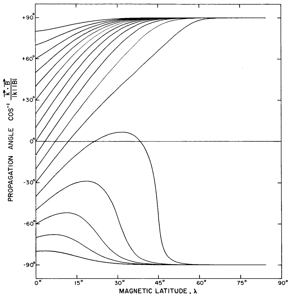
Fig. 4 Whistler Wave Normal Rotation
