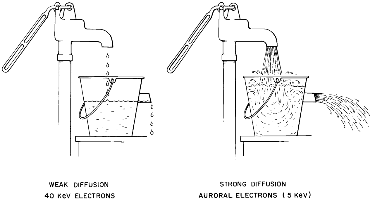
Fig. 9 Weak and Strong Diffusion
