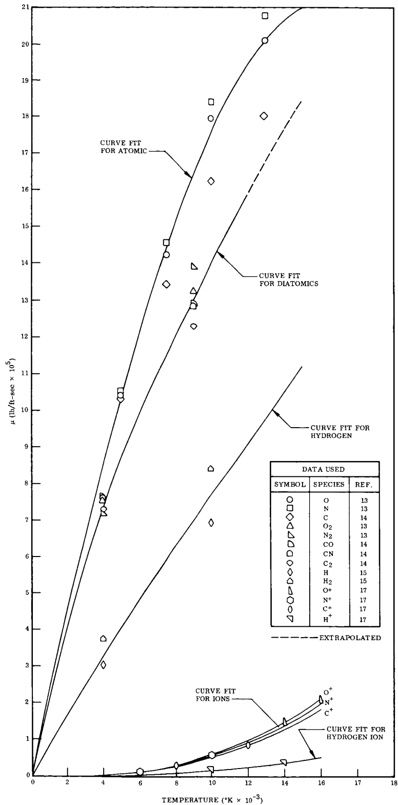
Fig. 6 Viscosity
