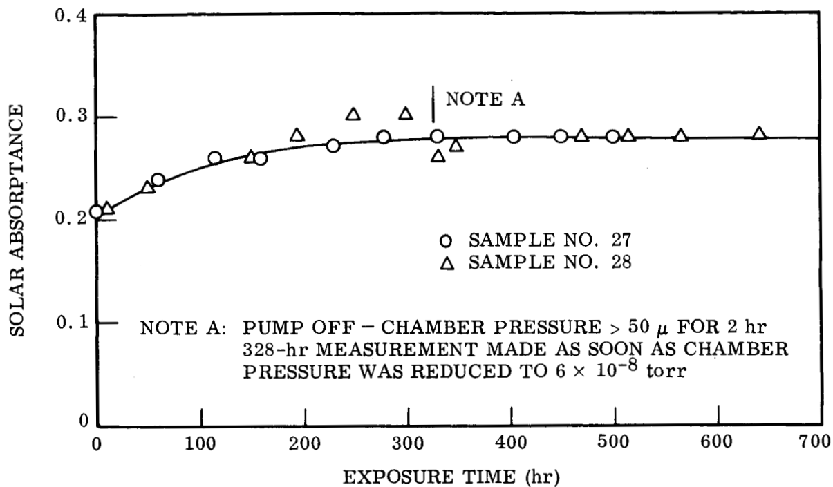
Fig. 2-1 Solar Absorptance of ZnO/Silicone (S-13) Coating Samples as a Function of Exposure Time at a 1-Sun Level and 395°K (252°F) Test Temperature
