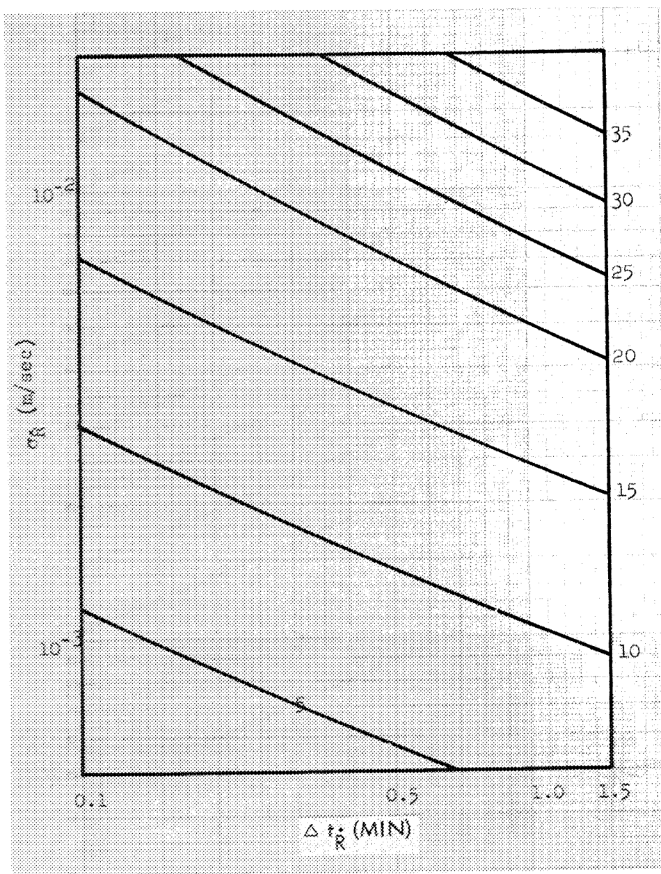
Figure 17. Velocity Error Contours in m/sec \sigma_R = 5m , \Delta t_R = 8 min (3 pts)
