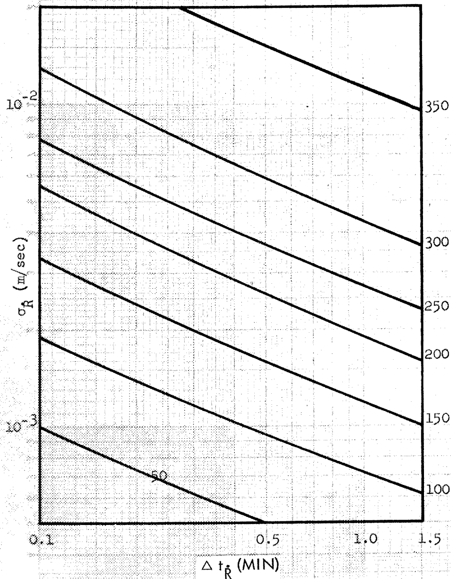
Figure 9. Position Error Contours in Meters for \sigma_R = 10\text{m} , \Delta t_R = 5 \text{ min} (4 pts)
