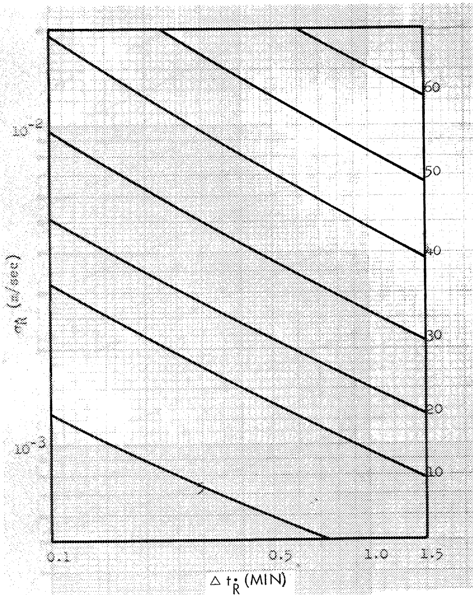
Figure 15. Velocity Error Contours in m/sec \sigma_R = 15m , \Delta t_R = 8 \text{ min (3 pts)}
