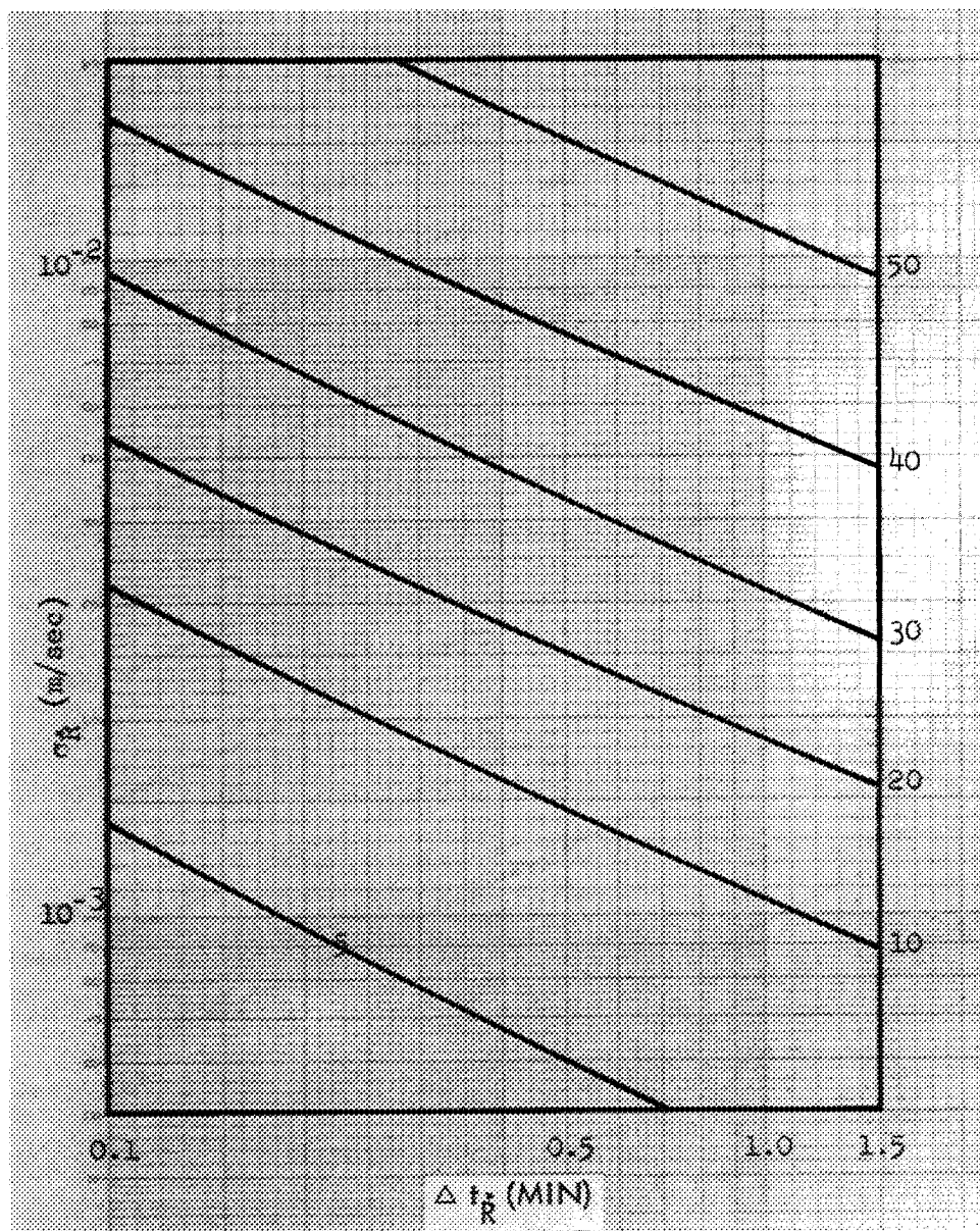
Figure 18. Velocity Error Contours in m/sec \sigma_R = 15m , \Delta t_R = 5 min (4 pts)
