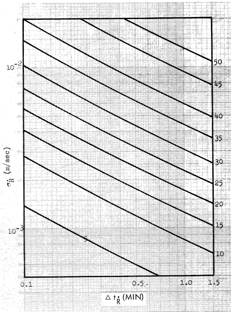
Figure 13. Velocity Error Contours in m/sec \sigma_R = 10m , \Delta t_R = 15 min (2 pts)
