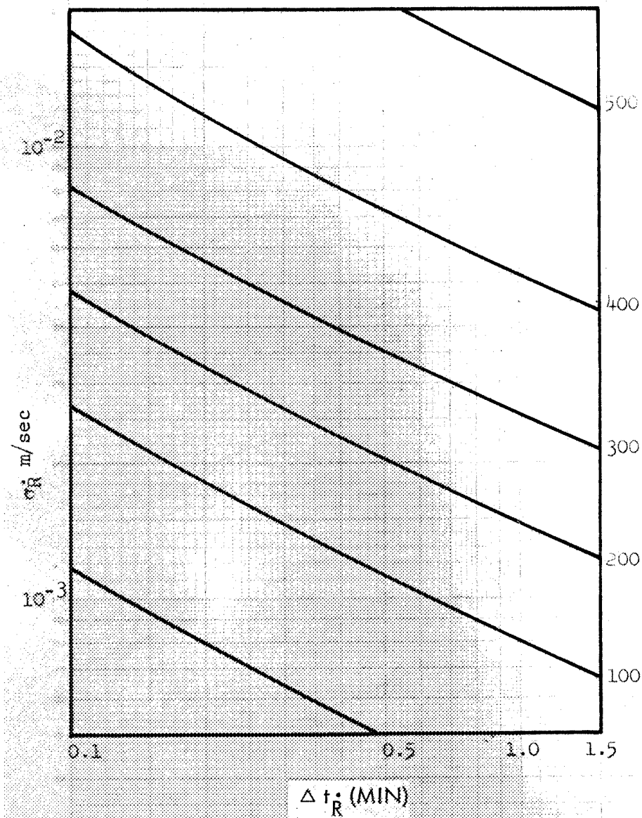
Figure 3. Position Error Contours in Meters for \sigma_R = 10\text{m} , \Delta t_R = 15 \text{ min} (2 pts)
