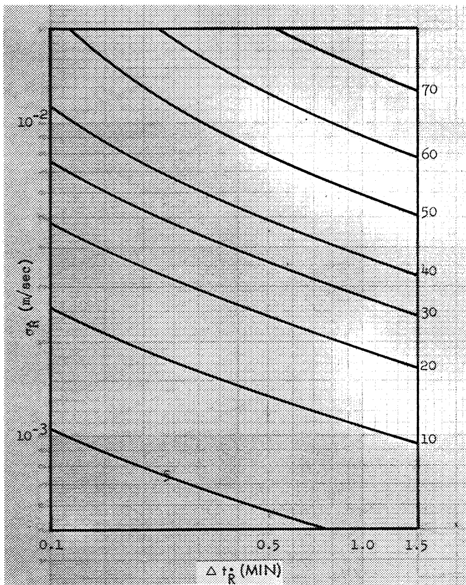
Figure 12. Velocity Error Contours in m/sec \sigma_R = 15m , \Delta t_R = 15 min (2 pts)
