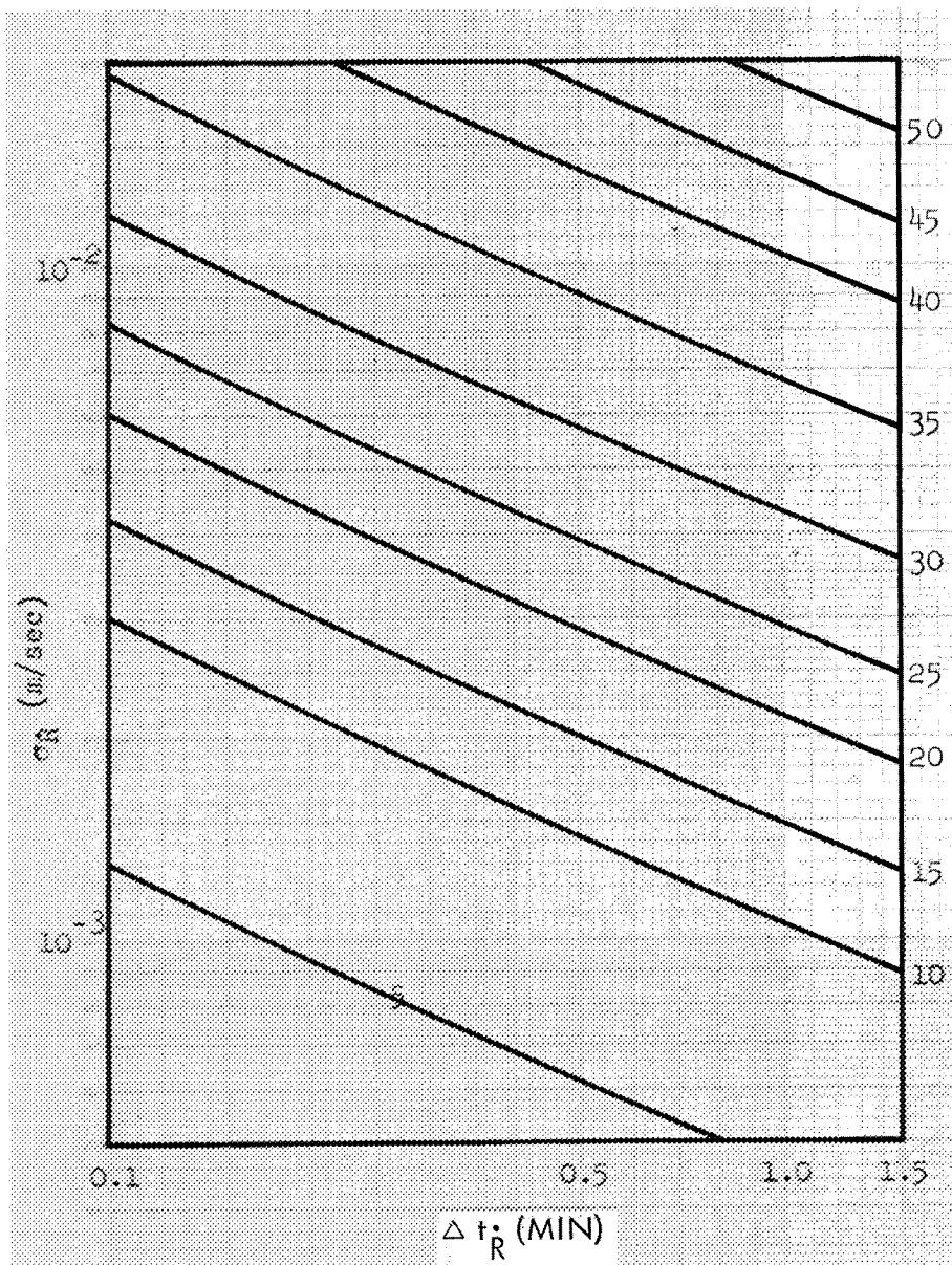
Figure 16. Velocity Error Contours in m/sec \sigma_R = 10m , \Delta t_R = 8 min (3 pts)
