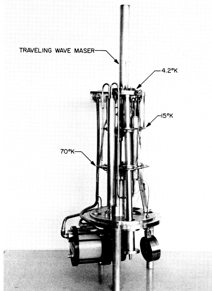
Fig. 21. Refrigerator with maser (vacuum jacket removed)
