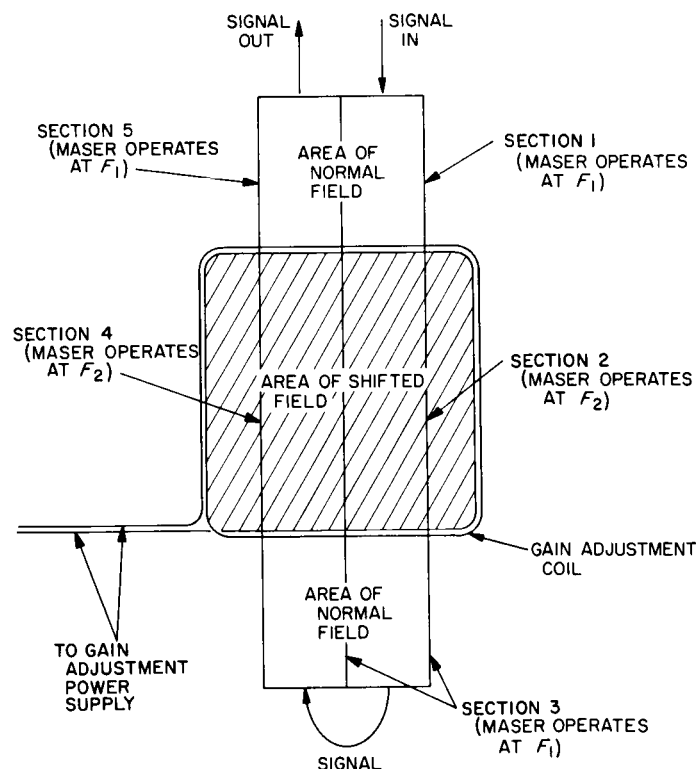
Fig. 12. Gain adjustment coil
