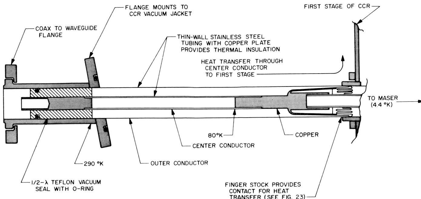
Fig. 22. Signal input coaxial line assembly
