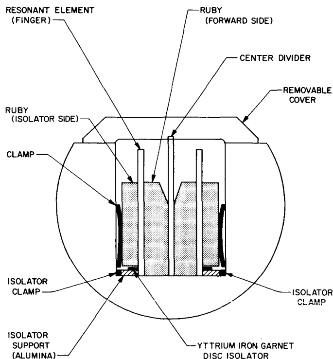
Fig. 8. End view of TWM
