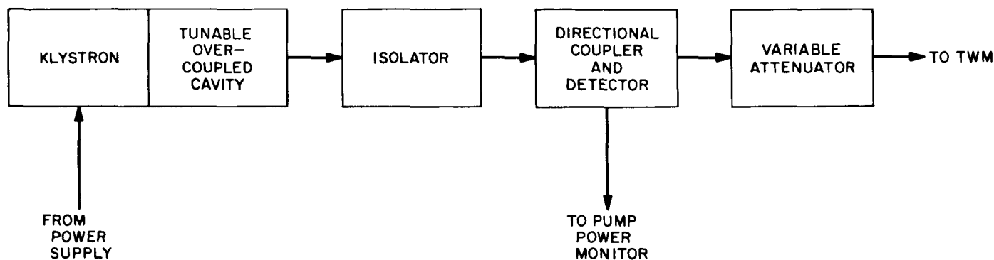
Fig. 17. Dual-frequency klystron package block diagram
