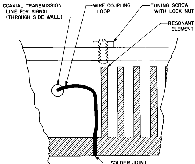
Fig. 4. TWM signal coupling loop
