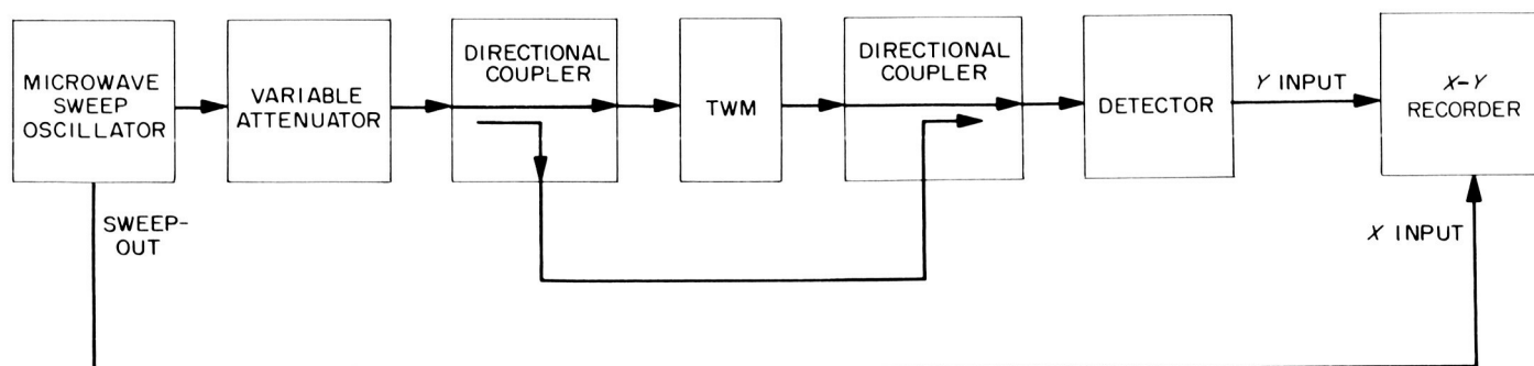
Fig. 2. Method for measurement of TWM electrical length
