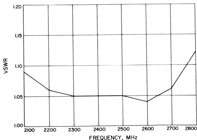
Fig. 24. VSWR vs frequency for thermal short circuit
