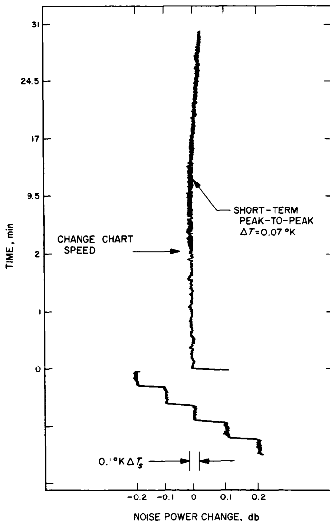
Fig. 28. Recording of total system noise power
