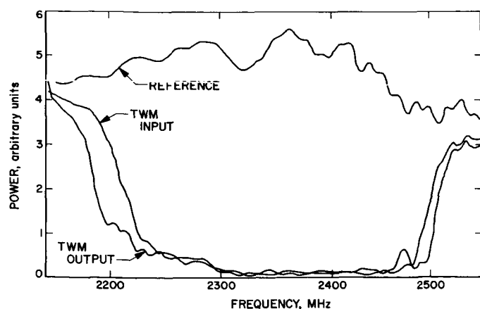
Fig. 7. Reflected power from TWM
