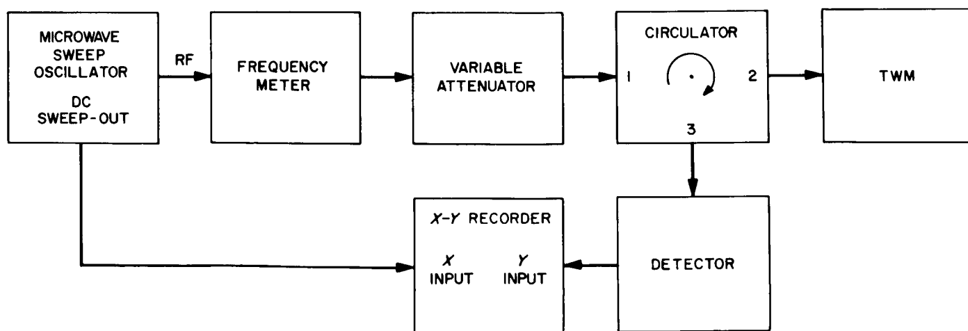
Fig. 5. Test setup for measuring reflected power
