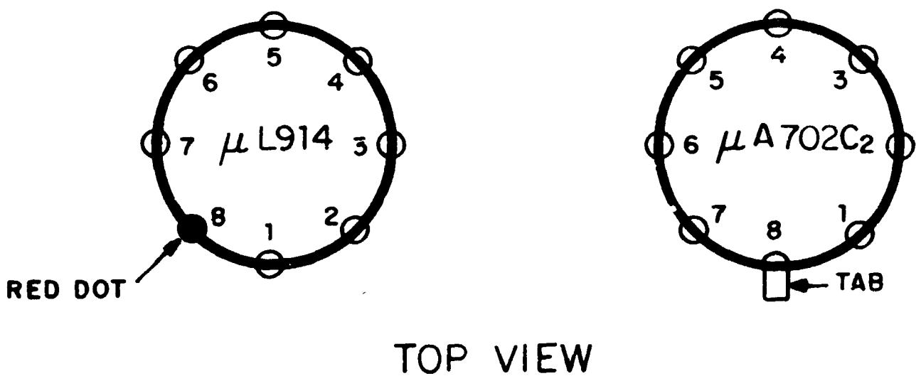
FIGURE 2D Basing diagrams for \mu L914 and \mu A702C .
