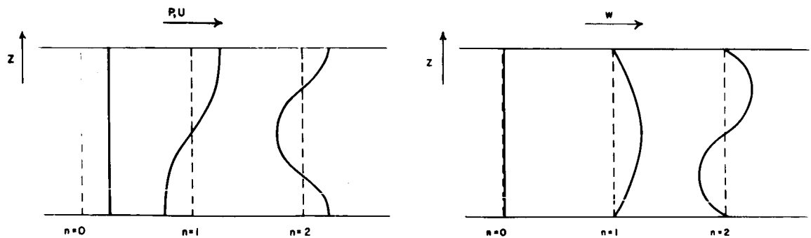
Fig. 10. The dependence of fluctuating pressure and velocities across a guide with perfectly reflecting rigid boundaries, for the first few modes. (After Budden, 1961)
