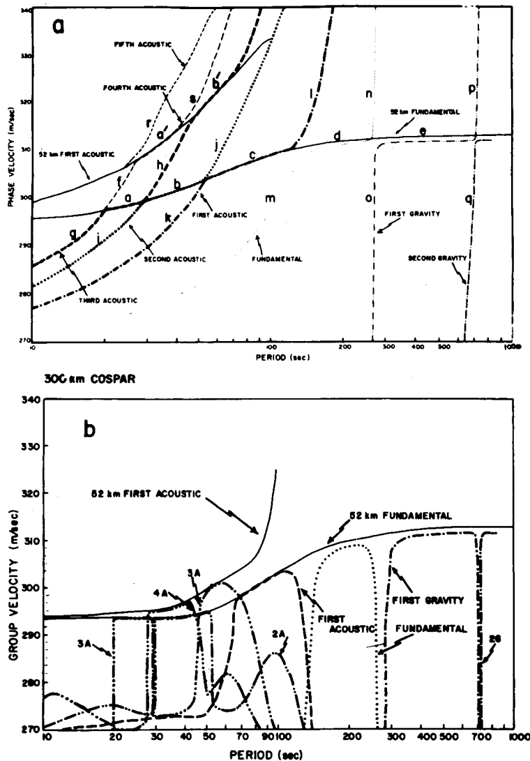
Fig. 23. Comparison between dispersion curves for the 52 km and 300 km models, showing the quasi-horizontal portions of the phase and group velocity curves for the 300 km model coincide with the solutions for the 52 km model. (a) phase velocity vs. period; (b) group velocity vs. period. The small letters in the upper figure refer to points at which vertical profiles of kinetic energy were calculated and are shown in Fig. 26. (After Pfeffer and Zarichny, 1963)
