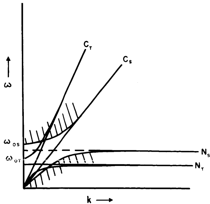
Fig. 2. Characteristic diagram for two layer atmosphere with warm troposphere, cold stratosphere.
