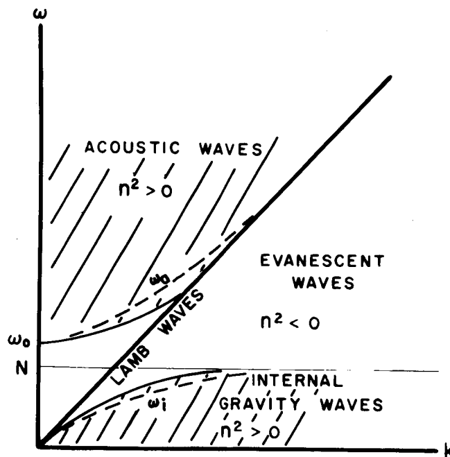
Fig. 3. Regions of solutions for a compressible, stratified fluid in a gravity field. Dashed curves correspond to neglect of gravity ( \omega_0 ) and compressibility ( \omega_i ). (After Tolstoy, 1963)
