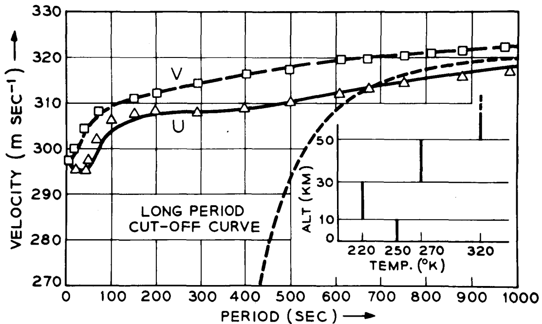
Fig. 6. Variation of group velocity (U) and phase velocity (V) with period for the fundamental mode for each of two four layer models. The curves are for the atmosphere shown in Fig. 5. Squares and triangles are for the four isothermal layers shown in the inset. The temperature of each layer is the mean of the corresponding layer in Fig. 5. The dashed cut off curve represents the boundary between cellular and non-cellular solutions in the infinite layer. (After Pfeffer and Zarichny, 1962)
