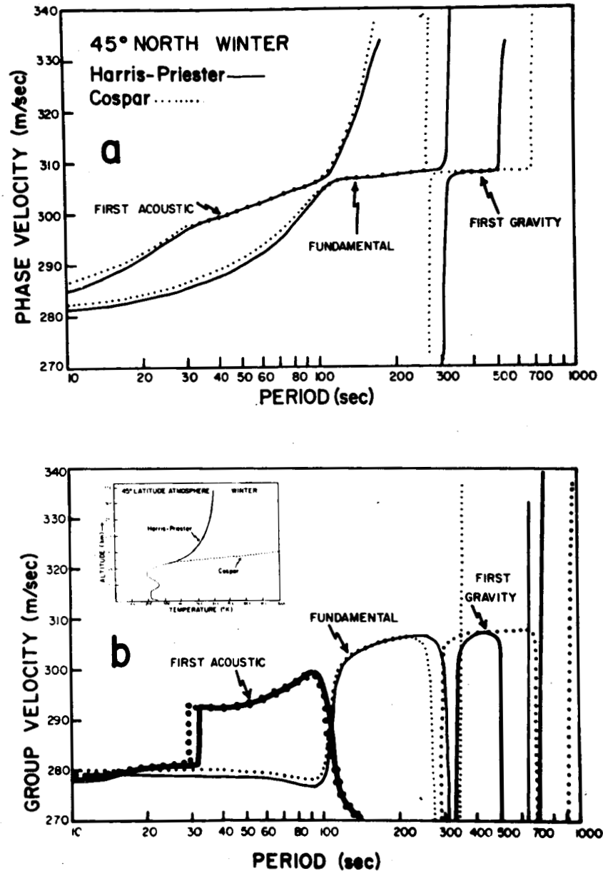
Fig. 24. Dispersion curves for model atmospheres consisting of the temperature structure at 45°N in winter up to 90 km merged with a nighttime atmosphere for a period of minimum solar activity due to Harris and Priester (solid curves) and with the mean COSPAR atmosphere (dotted curves). (a) phase velocity vs. period, (b) group velocity vs. period. The atmospheres are shown in the inset. (After Pfeffer and Zarichny, 1963)
