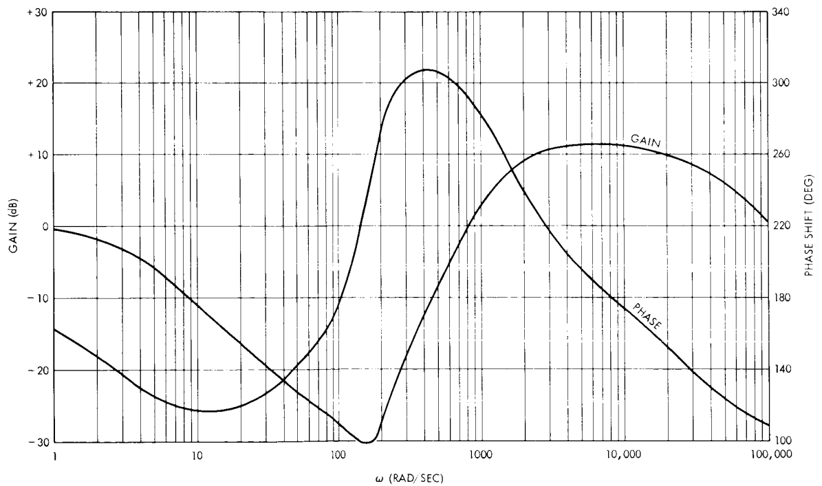
Figure A-4. Voltage Gain and Phase for Active Filter (Lead Network)
