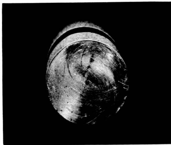
FIGURE 11. LIGHT GALLING DAMAGE OF ALUMINUM AND STAINLESS STEEL SURFACES CAUSED BY RELATIVE MOTION WITH SPECIMEN SURFACES LUBRICATED WITH KEROSENE
