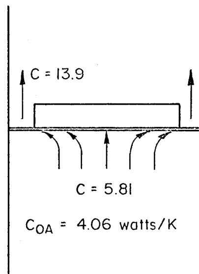
b) Diaphragm joint, no fluid conductance h = 50,000 \text{ Btu/hr-sq ft (F)}
