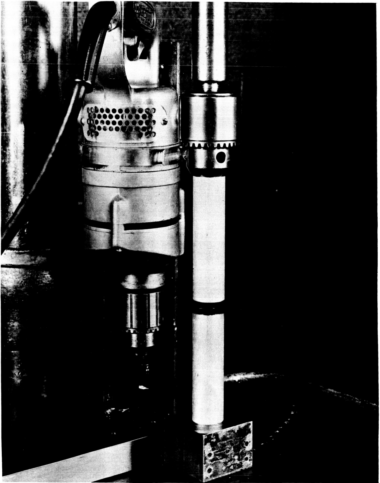
FIGURE 2. RIGID-SURFACE SPECIMEN-PAIR SETUP FOR AN EXPERIMENT
