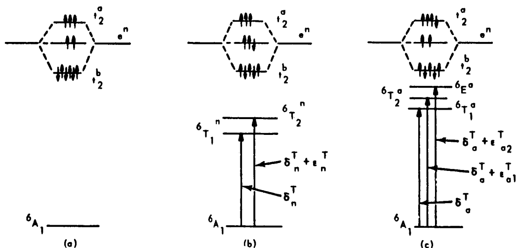
Fig. 5.2. (a) Ground state of complex [\Sigma\Lambda_4]^{-n'} , (b) t_2^b - e^n charge transfer states and their schematic energy levels, and (c) t_2^b - t_2^a charge transfer states and their schematic energy levels.
