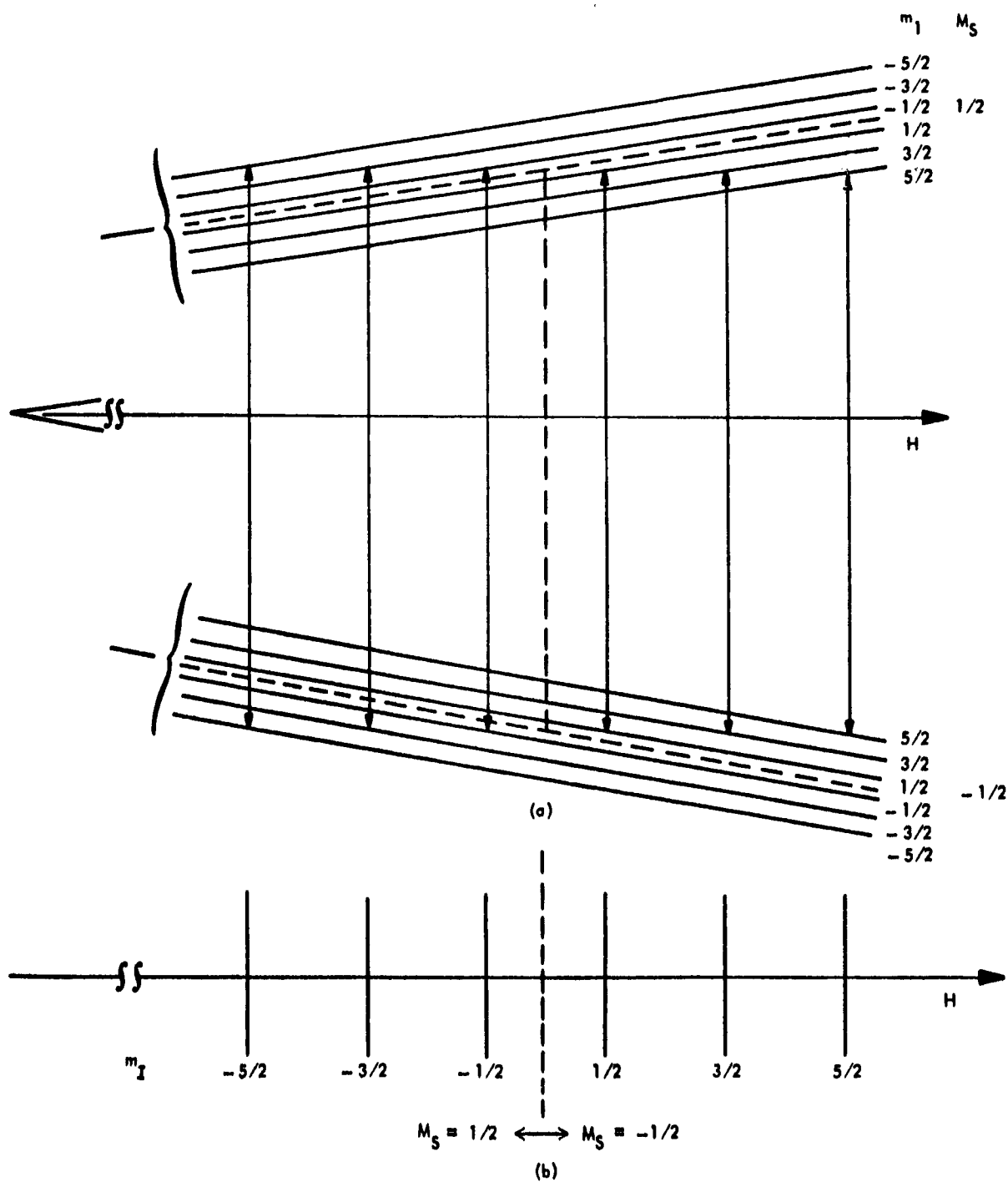
Fig. 2.5. (a) The splittings of M_S = \frac{1}{2} and -\frac{1}{2} levels into six close lying levels and (b) the splitting of the M_S = \frac{1}{2} \leftrightarrow M_S = -\frac{1}{2} transition into six approximately equally spaced transitions.
