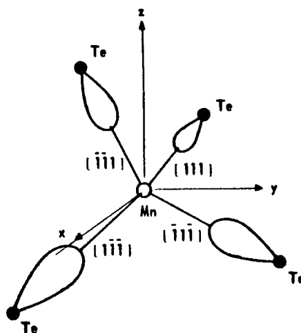
Fig. 2.2. The tetrahedral coordination in cubic II-VI compounds ( \text{ZnTe}:\text{Mn} ).
