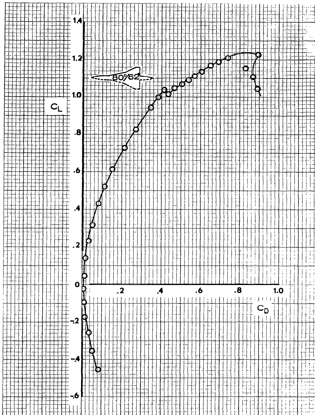
Figure 4b Lift-Drag Polar, 80°/62° Double-Delta Wing
