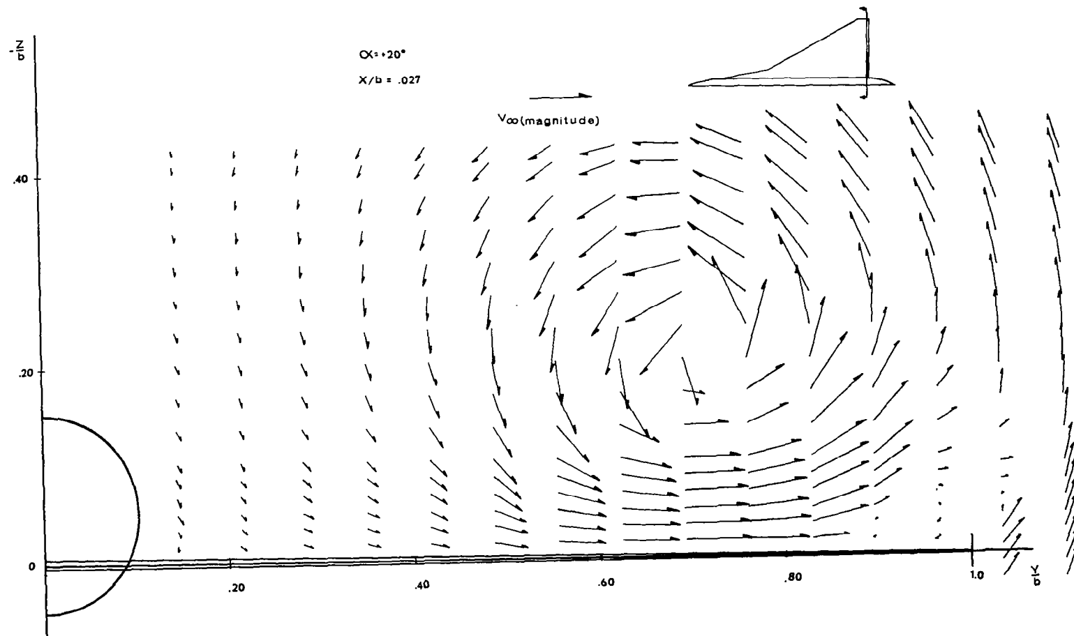
FIGURE 12d- Upper Surface Flow Field - 80\frac{1}{2}^\circ \Delta^2 - \alpha = 20^\circ X/b = .027
