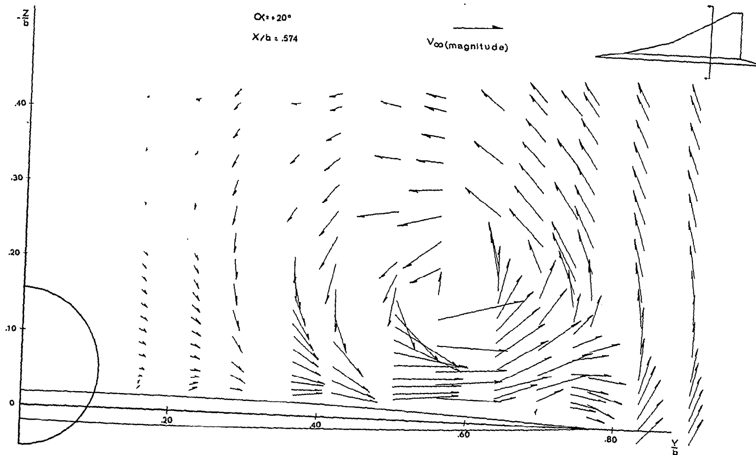
FIGURE 17b- Upper Surface Flow Field - 75^\circ 62' \Delta^2 - \alpha = 20^\circ X/b = .574
