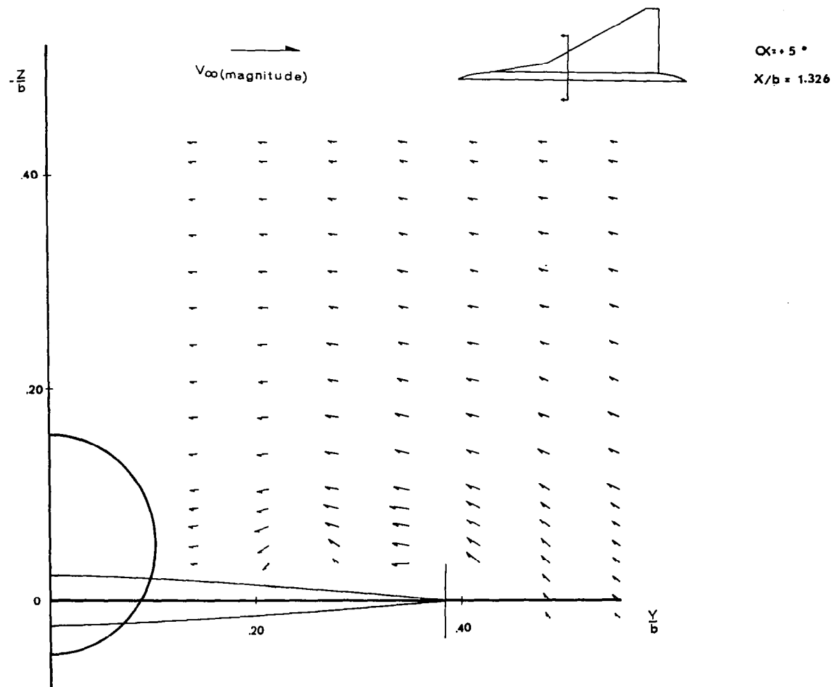
FIGURE 10b- Upper Surface Flow Field - 80\%62^\circ \Delta^2 - \alpha = 5^\circ X/b = 1.326
