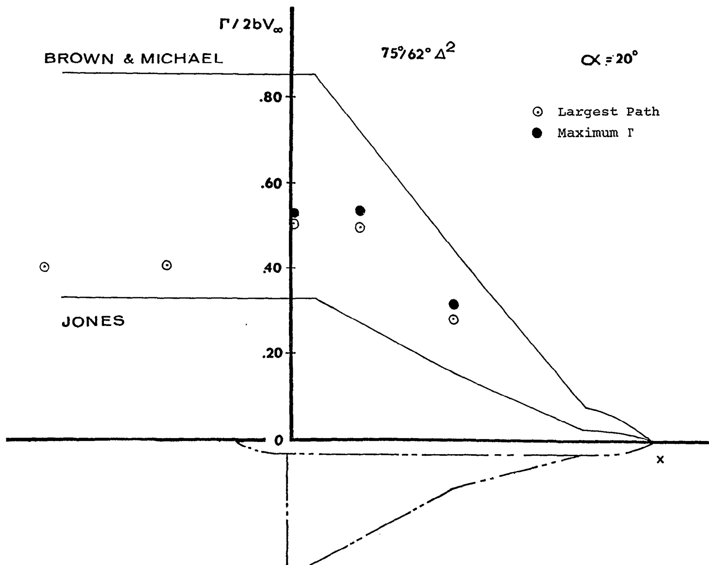
Figure 19c Circulation Integrals 75°/62° Double-Delta Wing, \alpha = 20^\circ
