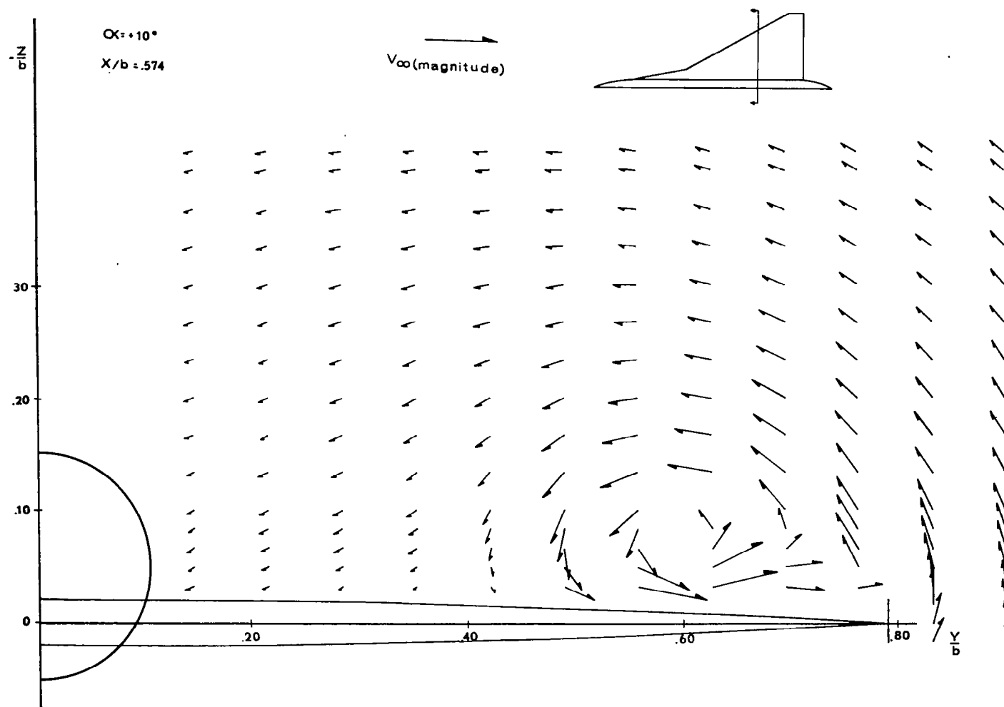
FIGURE 11c - Upper Surface Flow Field - 80^\circ/62^\circ \Delta^2 - \alpha = 10^\circ X/b = .574
