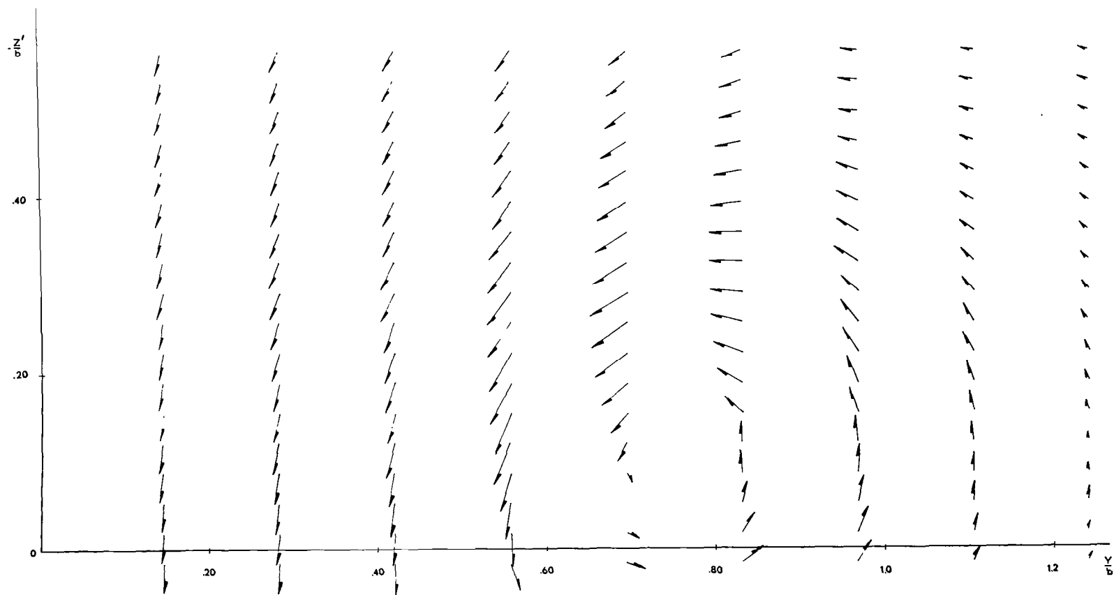
FIGURE 12f - Upper Surface Flow Field - 80/62^\circ \Delta^2 - \alpha = 20^\circ X/b = -2.0
