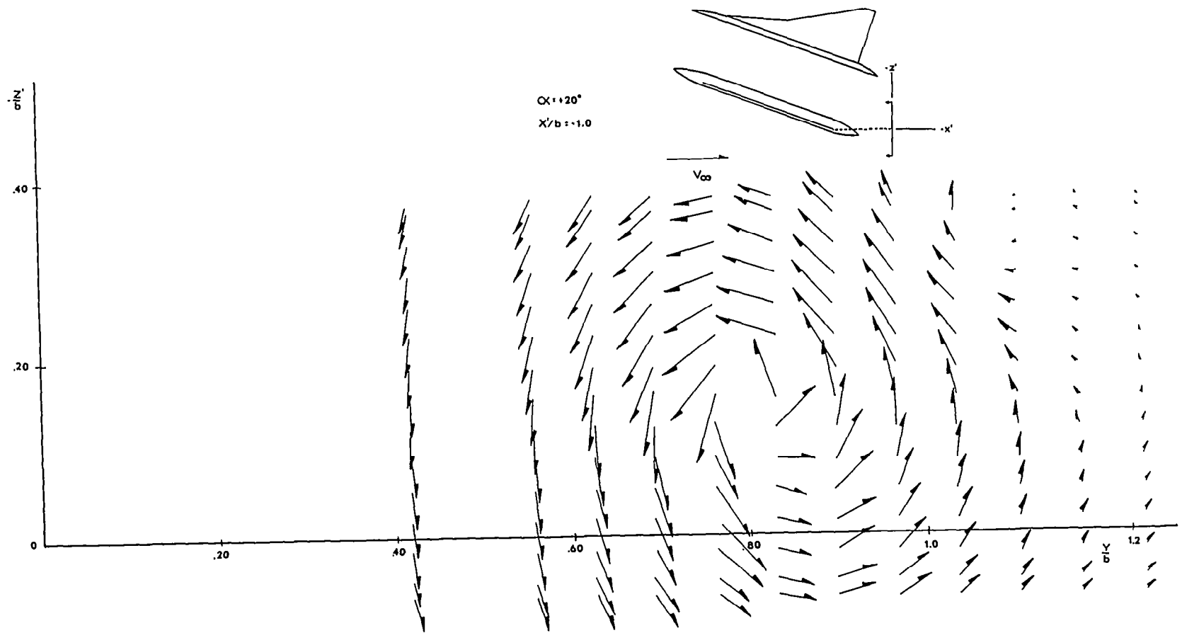
FIGURE 17d - Upper Surface Flow Field - 75\frac{7}{62}^\circ \Delta^2 - \alpha = 20^\circ X'/b = -1.0
