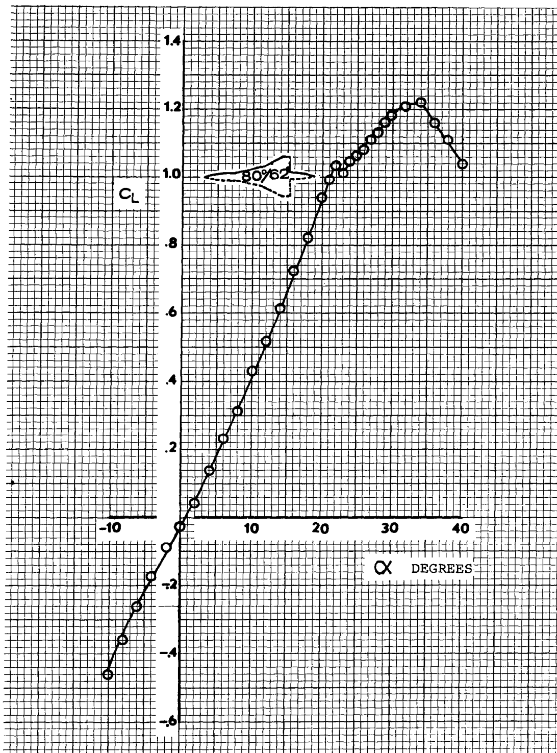
Figure 4a Lift Characteristic, 80°/62° Double-Delta Wing
