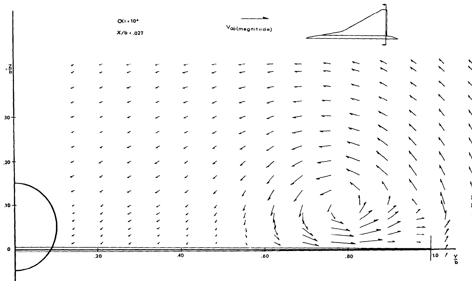
FIGURE 11d - Upper Surface Flow Field - 80^\circ 62' \Delta^2 - \alpha = +10^\circ X/b = .027
