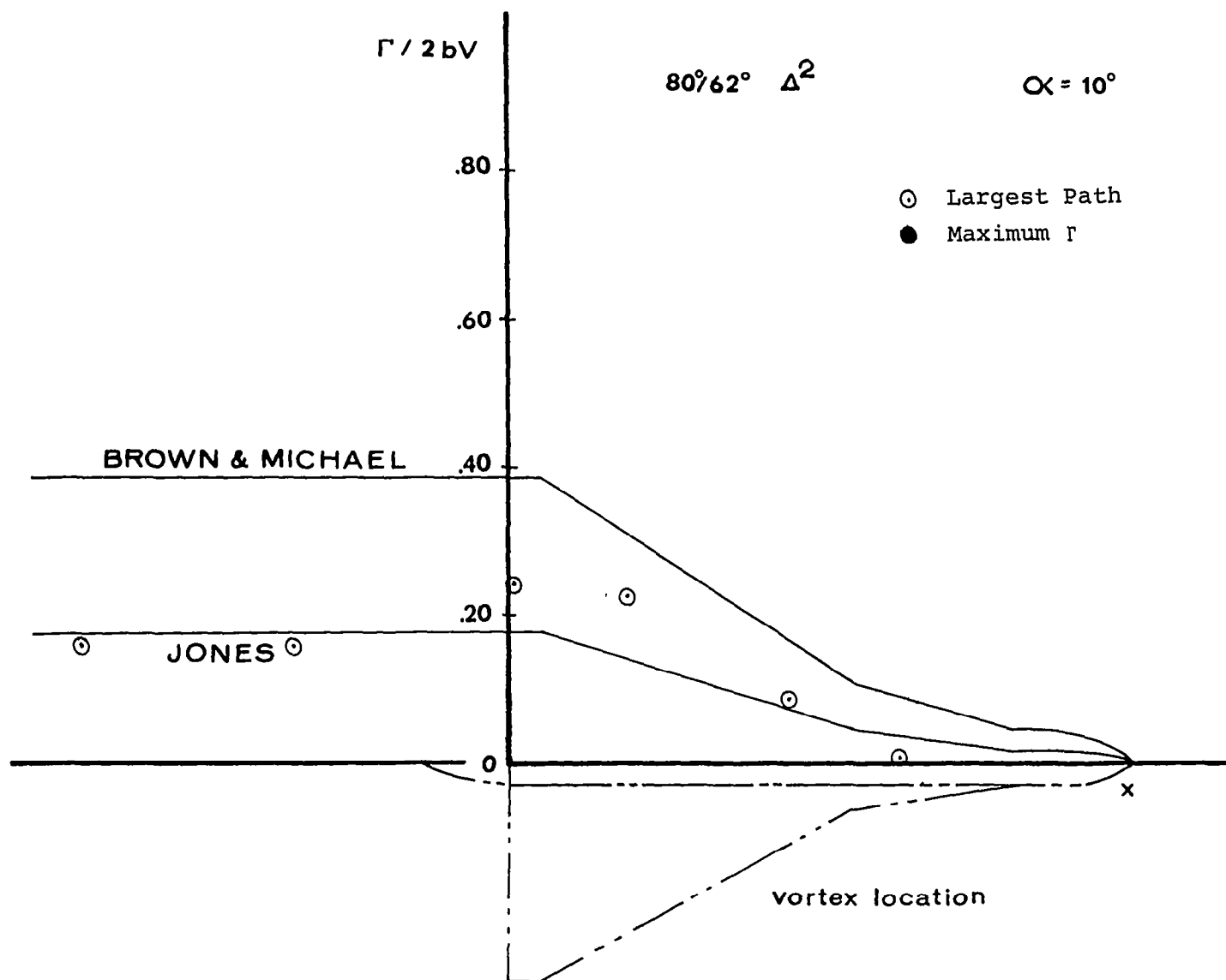
Figure 19d Circulation Integrals 80^\circ/62^\circ Double-Delta Wing, \alpha = 10^\circ
