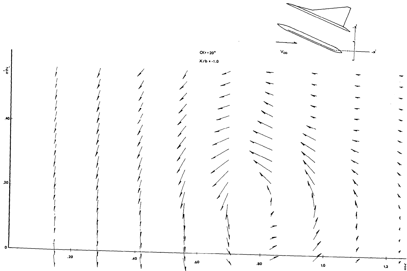
FIGURE 12e - Upper Surface Flow Field - 60/62° \Delta^2 - \alpha = 20^\circ X/b = -1.0
