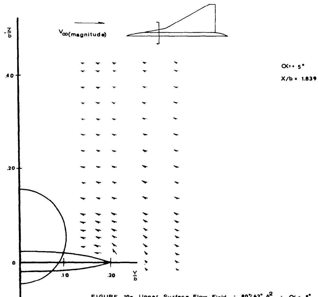
FIGURE 10a Upper Surface Flow Field - 80^\circ/62^\circ \Delta^2 - \alpha = 5^\circ X/b = 1.839
