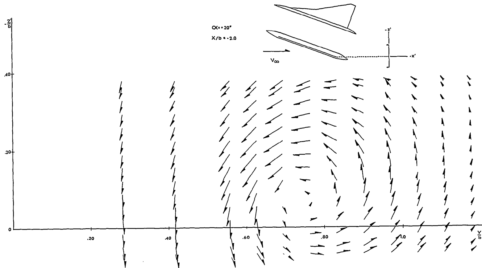
FIGURE 17e - Upper Surface Flow Field - 75^\circ 62' \Delta^2 - \alpha = 20^\circ X/b = 2.0
