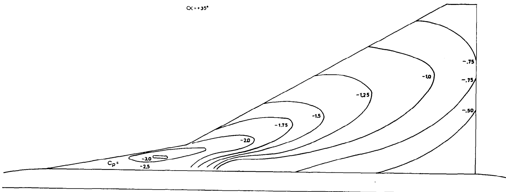
FIGURE 8h- Pressure Distribution - \alpha = +35^\circ
