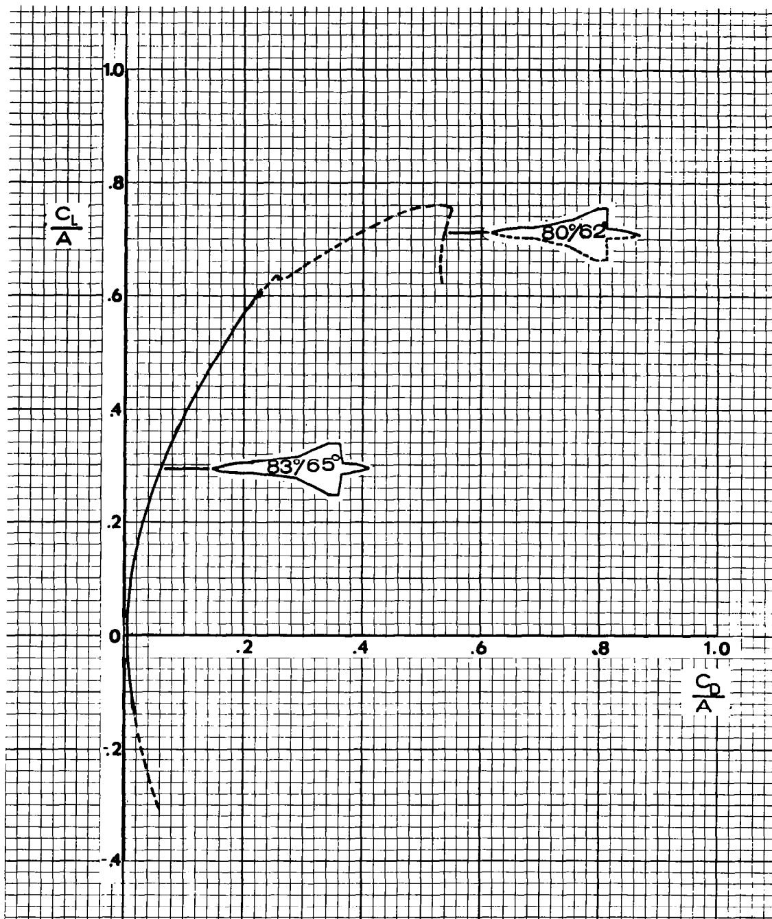
Figure 6b Drag Comparison, 80°/62° Double-Delta Wing and 83°/65° Double-Delta Wing
