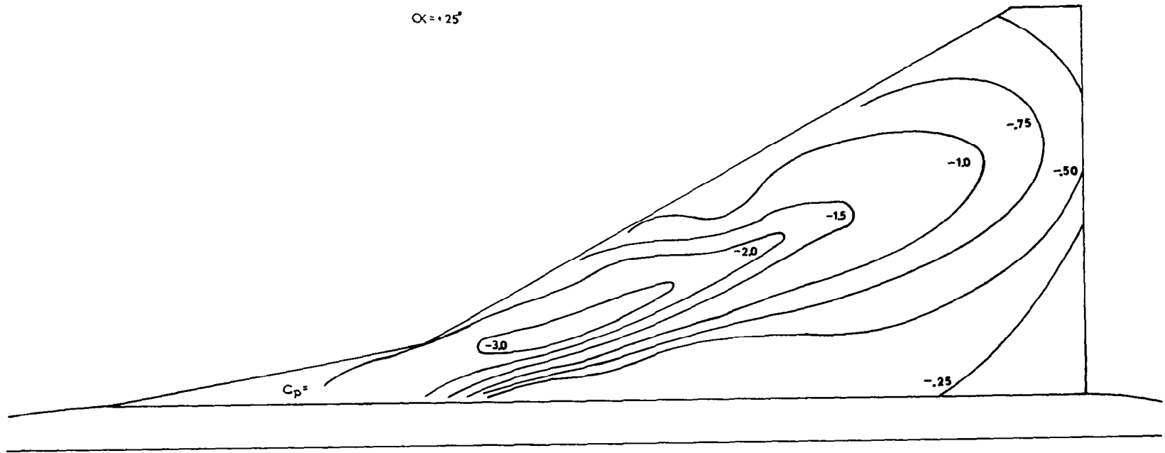
FIGURE 8f - Pressure Distribution - \alpha = +25^\circ
