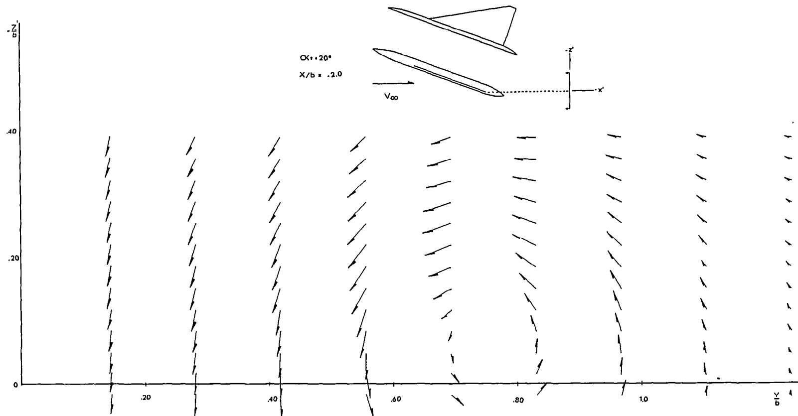
FIGURE 15a - Upper Surface Flow Field - 62^\circ \Delta - \alpha = 20^\circ X/b = 1.0
