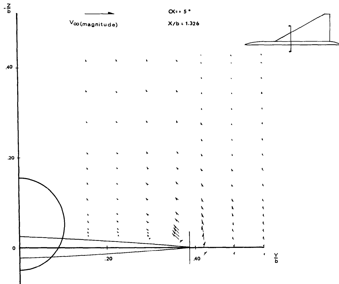
FIGURE 13a - Upper Surface Flow Field - 62^\circ \Delta - \alpha = 5^\circ X/b = 1.326
